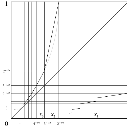
Figure 3: A graph of T_1 in Example 6
