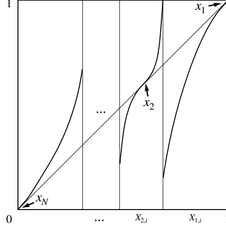
Figure 1: A graph of T_i for some i \in I in Definition 4.16
