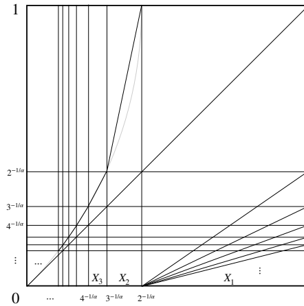
Figure 5: A graph of transformations in Example 10 (infinitely many branches on X_1 correspond to T_i|_{X_1} , i \in I , respectively)
