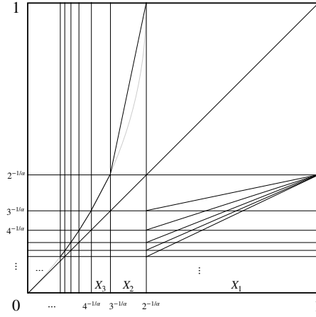
Figure 4: A graph of transformations in Example 8 and 9 (infinitely many branches on X_1 correspond to T_i|_{X_1} , i \in I , respectively)
