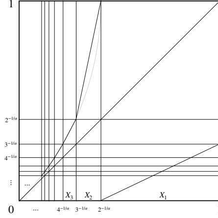
Figure 2: A graph of T_i for some i \in I of piecewise linear intermittent Markov maps
