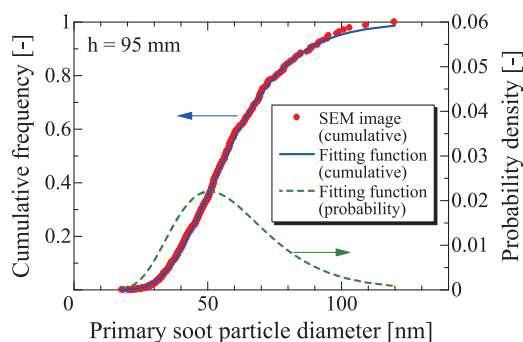
(c-2) Cumulative frequency and probability density functions for primary soot particle diameter ( h = 95 mm)
