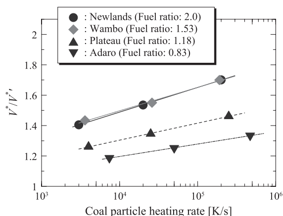
Fig. 4 V^*/V^{*'} (Appropriate value for Q-factor) as a function of the coal particle heating rate calculated by FLASHCHAIN model. Reprinted with permission from Ref. (Hashimoto N. et al., 2012a). Copyright: (2012) Elsevier B.V.
