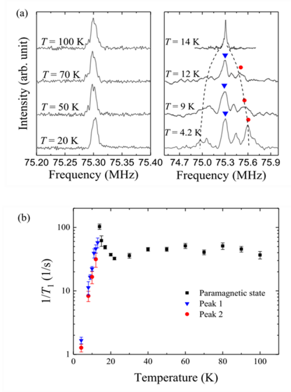
Figure 11: Temperature dependence of (a) the NMR spectra and (b) the nuclear spin-lattice relaxation rate ( 1/T_1 ) of \lambda\text{-(ET)}_2\text{GaCl}_4 [13].
