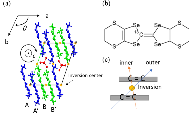
Figure 29: (a) Crystal structure of \lambda -(BETS) _2 GaCl _4 . The green and blue molecules represent crystallographically independent molecule. Yellow dots represent the inversion symmetry. (b) ^{13}\text{C} enriched BETS molecule. (c) Crystallographically independent ^{13}\text{C} sites (inner and outer cite).
