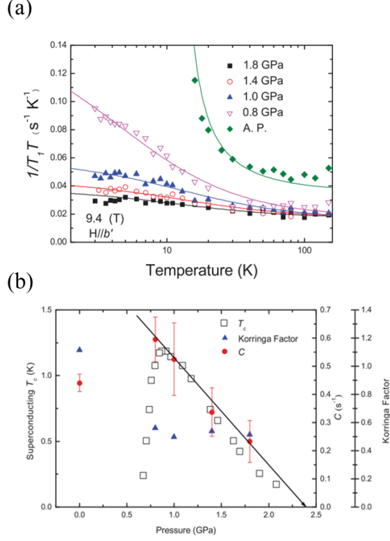
Figure 35: (a) Temperature dependence of 1/T_1T for (\text{TMTSF})_2\text{PF}_6 measured by ^{13}\text{C} -NMR under pressure. (b) Pressure dependence of the strength of SDW fluctuation (constant C ), superconducting T_c , and Korringa factor [26].
