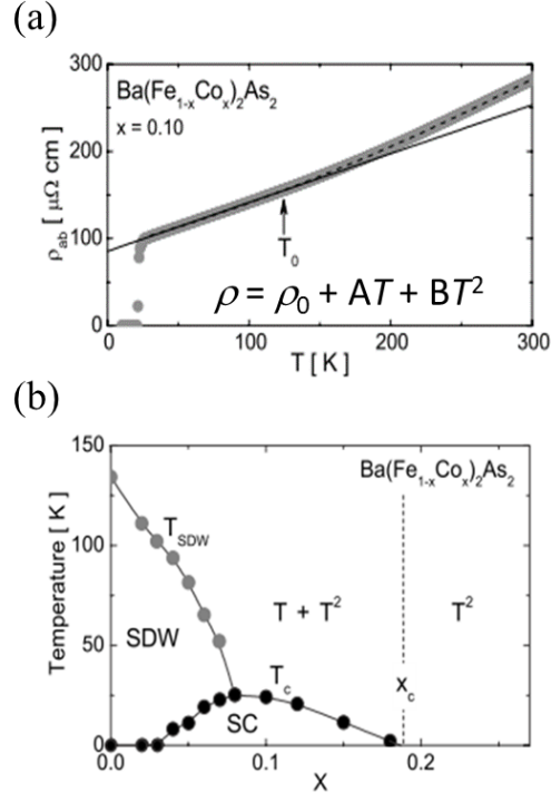
Figure 38: (a) Temperature dependence of electric resistivity for \text{Ba}(\text{Fe}_{1-x}\text{Co}_x)_2\text{As}_2 . (b) Phase diagram of \text{Ba}(\text{Fe}_{1-x}\text{Co}_x)_2\text{As}_2 .
