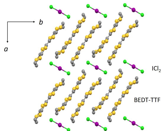
Figure 40: Crystal structure of \beta'-(\text{ET})_2\text{ICl}_2 .
