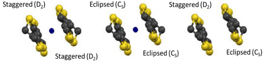
Figure 52: The schematics of the possible origin of the charge degrees of freedom in a dimer.
