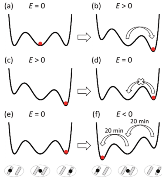
Figure 49: Schematics of the three valley model.
