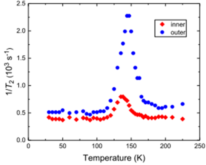
Figure 60: The temperature dependence of the spin-spin relaxation rate ^{13}\text{T}_2^{-1} .
