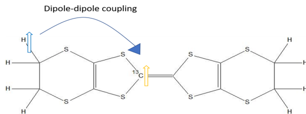
Figure 61: The schematic of the direct coupling mechanism.
