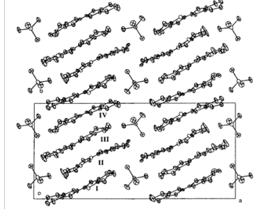
Figure 24: Cell parameter and crystal structure of \delta -(ET) 2 GaCl 4 .
