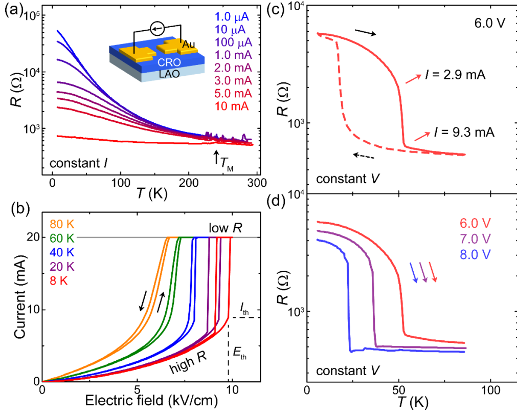
Figure 3. (a) Temperature dependence of the resistance of a CRO thin film on an LAO (001) substrate measured under a constant current of 1.0 \mu\text{A} –10 mA. The inset is a schematic illustration of the two-terminal electrode with a lateral gap of 20 \mu\text{m} used for the measurements. (b) I – E characteristics of a CRO thin film on an LAO (001) substrate measured at T = 8 –80 K. The arrows indicate the directions of the electric field sweeping. The horizontal line at 20 mA shows the current compliance set by the measurement unit. (c) Temperature dependence of the resistance of a CRO thin film on an LAO (001) substrate measured under a constant voltage of 6.0 V, and (d) its voltage-amplitude dependence. The current values shown in (c) are for the two representative data points before/after the rapid change in the resistance was observed.
