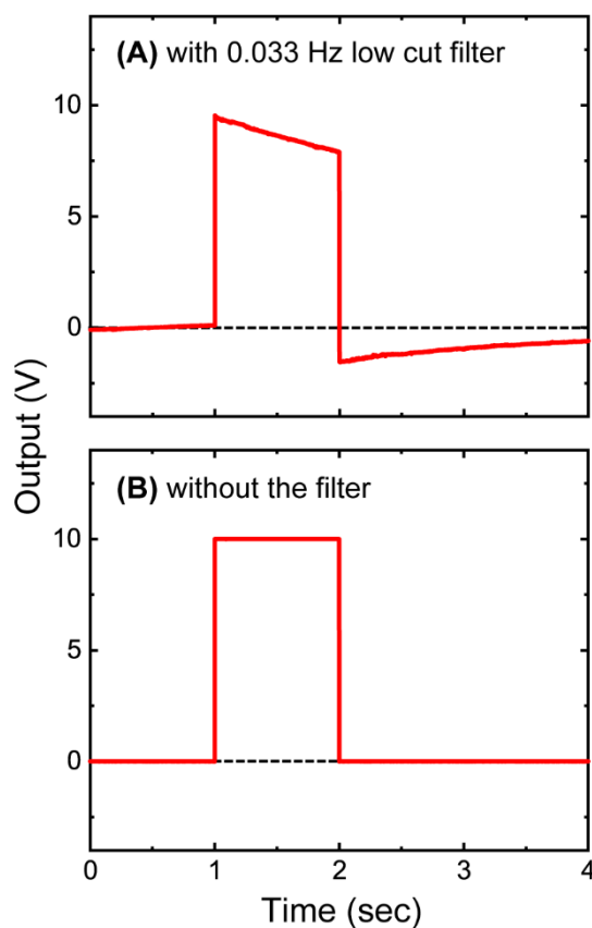
Figure 2-4. The response of the voltage amplifier for the input of square wave voltage. This amplifier is equipped with a removal 0.033 Hz low cut filter. Panels A and B show the output voltages with and without the filter, respectively. Here, we inputted the square wave voltage. The output with the filter was slightly differentiated. Reprinted with permission from {Keisuke, Murabe; Takashi, Tsukamoto; Tomoyasu, Aizawa; Makoto, Demura; Takashi, Kikukawa. Direct Detection of the Substrate Uptake and Release Reactions of the Light-Driven Sodium-Pump Rhodopsin. J. Am. Chem. Soc. 2020, 142, 37, 16023–16030.}. Copyright {2020} American Chemical Society.
