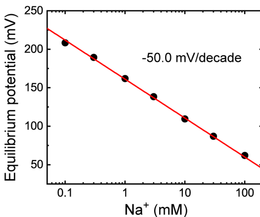
Figure 1-3. The Na + -concentration responses of the bare Na + -selective membrane. Reprinted with permission from {Keisuke, Murabe; Takashi, Tsukamoto; Tomoyasu, Aizawa; Makoto, Demura; Takashi, Kikukawa. Direct Detection of the Substrate Uptake and Release Reactions of the Light-Driven Sodium-Pump Rhodopsin. J. Am. Chem. Soc. 2020, 142, 37, 16023–16030.}. Copyright {2020} American Chemical Society.
