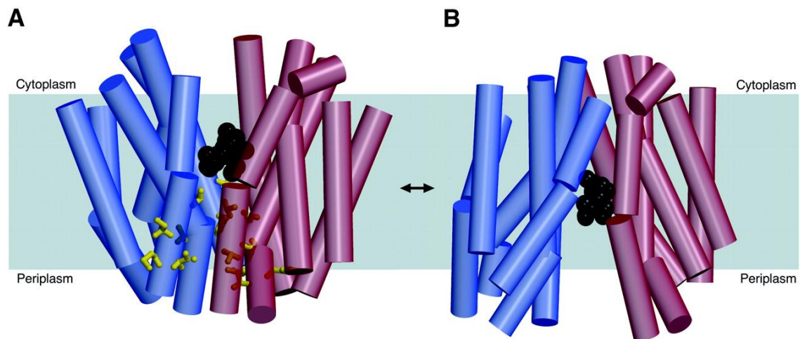
Fig 1. Schematic illustration of the alternating access model [14]. The predicted conformation changes are shown for the Lactose symporter. (A) Inward-facing conformation determined by the X-ray structural analysis. (B) A possible model for the outward-facing conformation based on the biochemical analyses. The substrate \beta -D-galactopyranosyl-1-thio- \beta -D-galactopyranoside (TDG) is shown in black.
