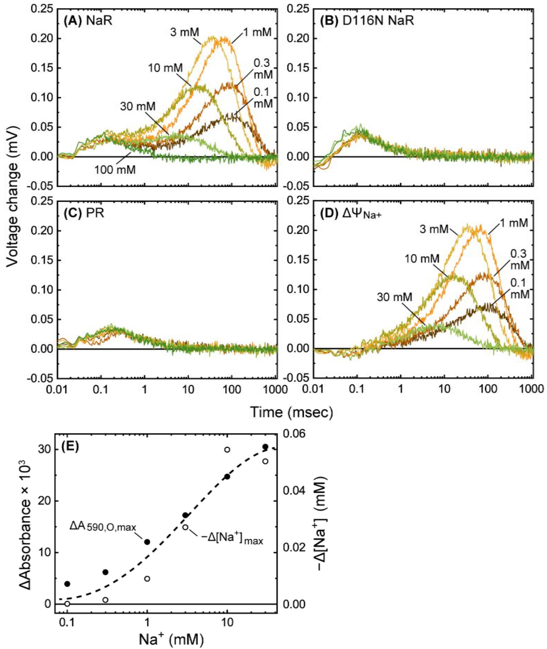
Figure 2-8. Flash-induced potential changes of the Na + -selective membrane. The membrane surfaces were covered with the lipid-reconstituted NaR (A), its D116N mutant (B), and PR (C), respectively. Panel D shows the remaining potential changes for wild-type NaR after subtraction of trace at 100 mM Na + . The peak values in this panel were picked up and then used for the calculations of the corresponding Na + -concentration changes ( \Delta [\text{Na}^+]_{\text{max}} ). The calculated values were plotted in Panel E (open circles) together with the peak values of the traces in Fig. 3D ( \Delta A_{590, \text{O}, \text{max}} , filled circles). For details, see the text.
