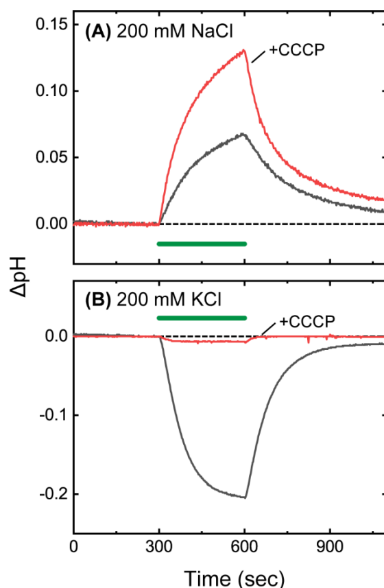
Figure 2-6. Light-induced pH changes of suspensions of E. coli cells expressing GLR. After harvest, the cells were starved in 200 mM NaCl or KCl overnight, respectively. These cells were washed again with the same salt solutions and then suspended so that the OD values at 660 nm became 0.5. The green bar indicates the period of green light illumination. In the presence of Na + (Panel A), pH increase was observed, indicating the outward Na + pumping activity of GLR. This activity creates inside negative potential, which drives H + influx and then induces pH increase. By the presence of 10 μM CCCP, the pH increase became large, reflecting the facilitation of membrane penetration of H + . On the other hand, in the absence of Na + (Panel B), pH decrease was observed due to the outward H + pumping activity of GLR. This pH change was disappeared by the addition of 10 μM CCCP, indicating that H + was indeed pumped by GLR. Reprinted with permission from {Keisuke, Murabe; Takashi, Tsukamoto; Tomoyasu, Aizawa; Makoto, Demura; Takashi, Kikukawa. Direct Detection of the Substrate Uptake and Release Reactions of the Light-Driven Sodium-Pump Rhodopsin. J. Am. Chem. Soc. 2020, 142, 37, 16023–16030.}. Copyright {2020} American Chemical Society.
