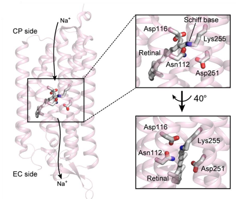
Figure 2-5. Positions of key residues for putative \text{Na}^+ binding sites. In this panel, crystal structure of NaR from Krokinobacter eikastus (PDB code: 3X3C) is shown with retinal and the nearby amino acid residues. Reprinted with permission from {Keisuke, Murabe; Takashi, Tsukamoto; Tomoyasu, Aizawa; Makoto, Demura; Takashi, Kikukawa. Direct Detection of the Substrate Uptake and Release Reactions of the Light-Driven Sodium-Pump Rhodopsin. J. Am. Chem. Soc. 2020, 142, 37, 16023–16030.}. Copyright {2020} American Chemical Society.
