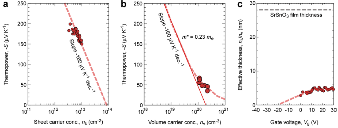
Figure 3. Electric field thermopower modulation analysis of the SrSnO 3 -based TFT at room temperature. (a) Sheet carrier concentration ( n_s ) dependences of S . The slope of S – n_s relationship is -160 \mu\text{V K}^{-1} \text{decade}^{-1} (dotted line). (b) Volume carrier concentration ( n_v ) dependence S of the La-doped SrSnO 3 films. We calculated the carrier effective mass ( m^* ) of the La-doped SrSnO 3 film around 0.23 m_e . The dotted line indicates the result of the calculation of S . A linear line can be drawn with a slope of -160 \mu\text{V K}^{-1} \text{decade}^{-1} . (c) The effective thickness ( t_{\text{eff}} ), which is defined as n_s/n_v , as a function of V_g . The t_{\text{eff}} increases with V_g and saturates around 5 nm, whereas the La-doped SrSnO 3 film thickness is 28 nm.
