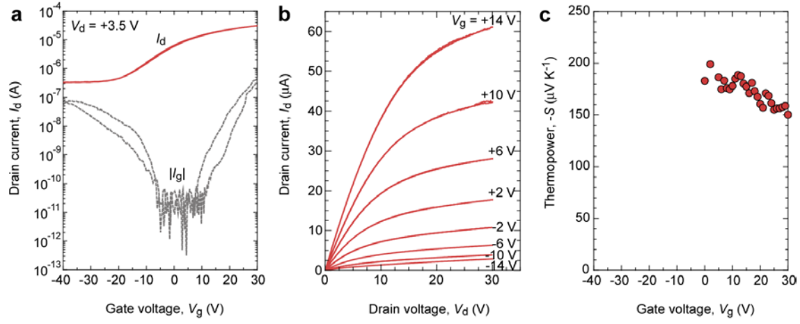
Figure 2. Transistor characteristics of the resultant TFT at room temperature. (a) Transfer ( I_d – V_g ) characteristics ( V_d = 3.5 V). The absolute values of the gate leakage current ( |I_g| ) are also plotted. The on-to-off current ratio of I_d is \sim 10^2 . (b) Output characteristics. Pinch-off behavior is clearly seen. (c) Change in the thermopower ( S ) as a function of V_g . The -S gradually decreases with V_g .
