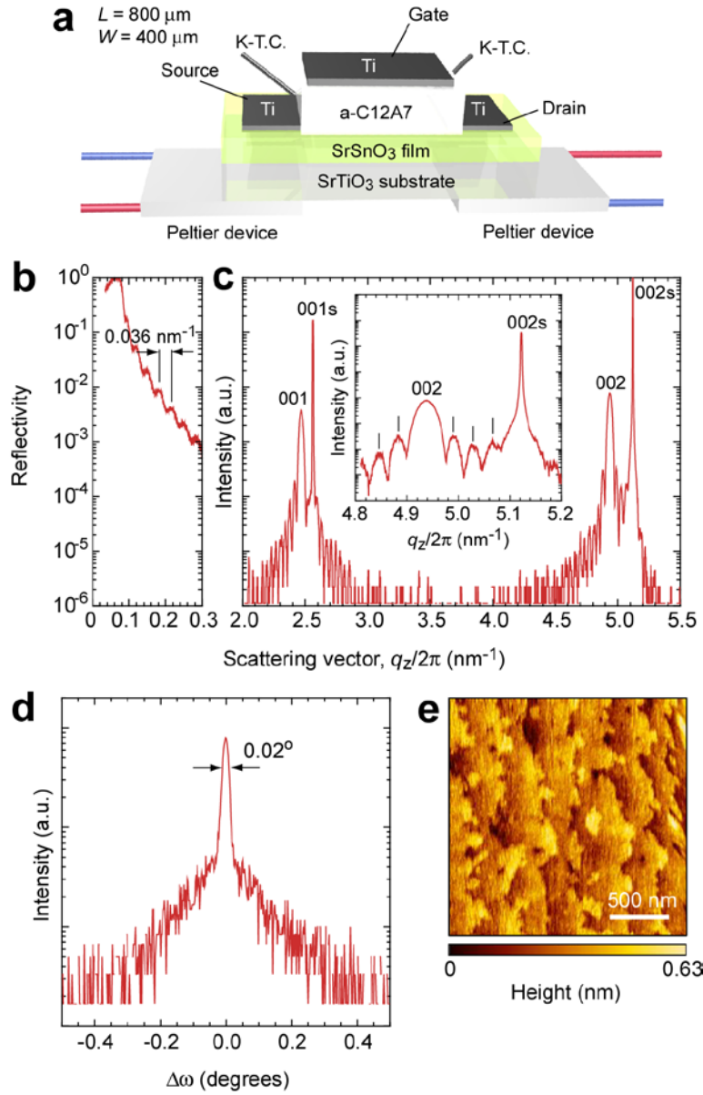
Figure 1. La-doped SrSnO 3 -based TFT. (a) Schematic illustration of the La-doped SrSnO 3 -based TFT, which is placed on the gap between two Peltier devices. The Peltier devices are used to provide temperature difference ( \Delta T ) between both edges of the TFT channel. The thermo-electromotive force ( \Delta V ) and \Delta T are measured simultaneously during gate voltage ( V_g ) application. (b) X-ray reflection pattern of the La-doped SrSnO 3 film. Kiessig fringes observed at lower scattering vector were used to calculate the thickness of the La-doped SrSnO 3 films, which was 27.8 nm. (c) Out-of-plane XRD pattern. The inset is the zoomed region around the 002 Bragg peak of La-doped SrSnO 3 . Pendellösung fringes are clearly observed around 00l diffraction peaks. (d) Rocking curve of the 002 La-doped SrSnO 3 . The full-width-at-half-maximum (FWHM) is 0.02°, showing strong 00l orientation of the film. (e) Topographic AFM image of the La-doped SrSnO 3 film. Stepped and terraced surface is seen.
