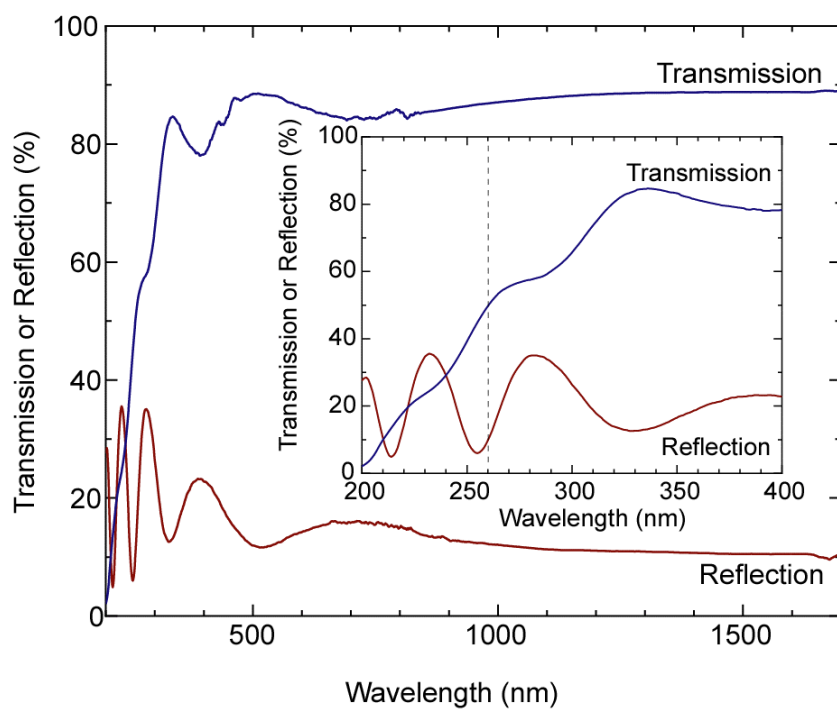
Figure S2. Optical transmission and reflection spectra of the multilayer of a-C12A7 film (300 nm) / La-doped SrSnO 3 film (23 nm) / (001) MgO substrate (0.5 mm). The optical transmission at 260 nm in wavelength is greater than 50%.
