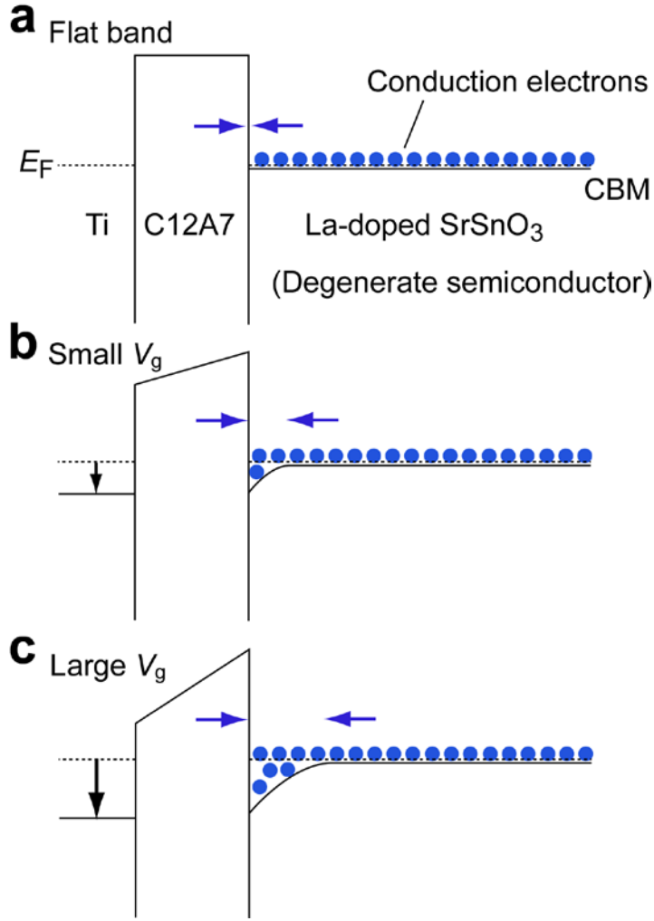
Figure 4. Electric field modulation mechanism of the SrSnO 3 -based TFT. (a) Without any gate voltage ( V_g ) application. (b) Under small V_g application. The conduction band bending happened. The conducting channel formed at the C12A7/La-doped SrSnO 3 interface. The thickness of conducting channel ( t_{eff} ) gradually increases up to ~5 nm. (c) Under large V_g application. The t_{eff} saturated at ~5 nm.
