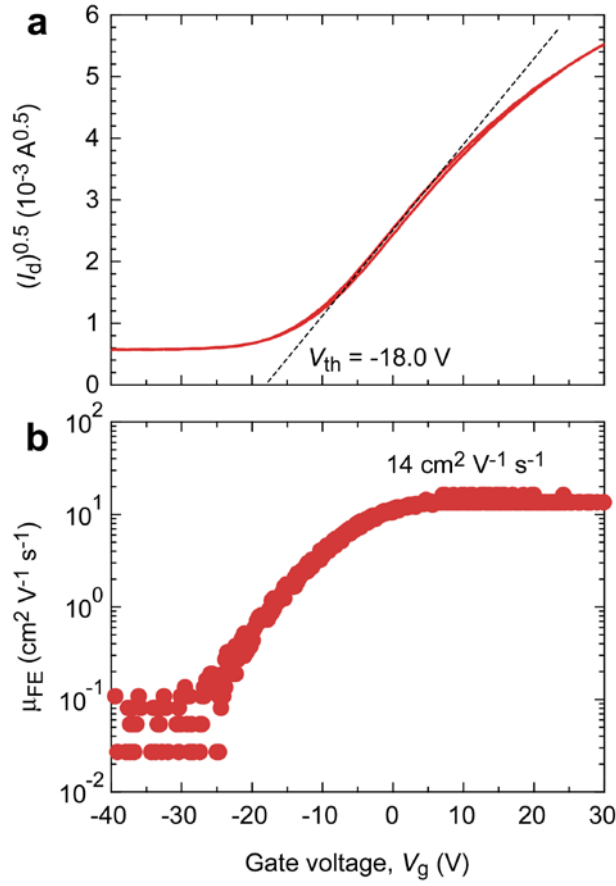
Figure S1. Detailed transistor characteristics of the SrSnO 3 -based TFT. (a) I_d^{0.5} – V_g plot. The threshold voltage ( V_{th} ) is -18.0 \text{ V} . (b) V_g dependence of the field effect mobility ( \mu_{FE} ). \mu_{FE} increases with V_g and reaches \sim 14 \text{ cm}^2 \text{ V}^{-1} \text{ s}^{-1} .
