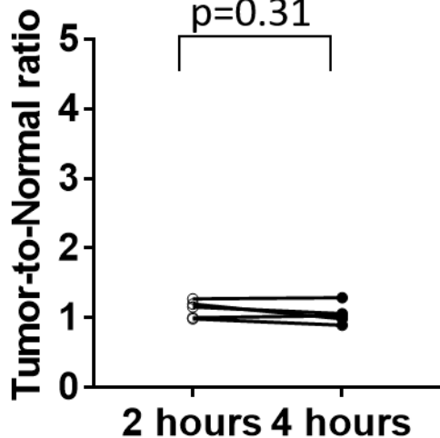
C. non-GBM
