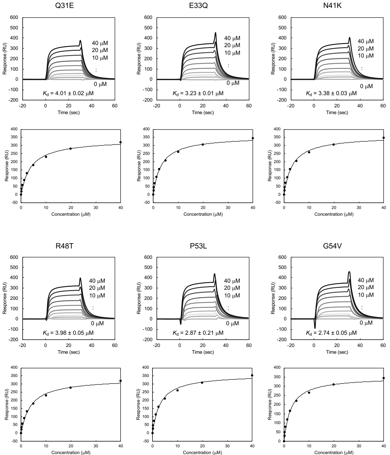
Figure. S6. Binding analysis between LILRA2 domain1 single mutants and N-truncated Ig. Each 0.16–40 \mu\text{M} LILRA2 mt was injected over the N-truncated Ig immobilized chip. Equilibrium analyses were performed to calculate the K_d value.
