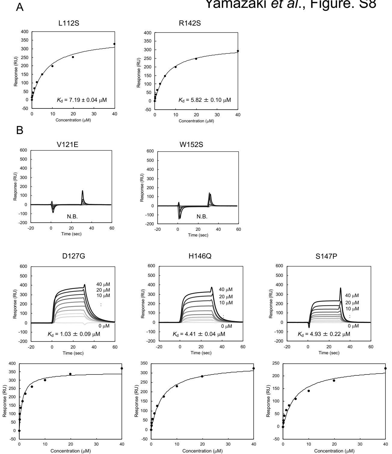
Figure. S8. Binding analysis between LILRA2 domain2 mutants and N-truncated Ig.
