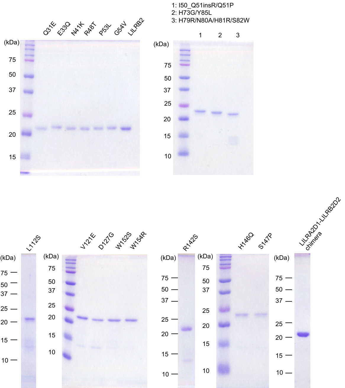
Figure. S4. SDS-PAGE of the proteins used for SPR analyses.
