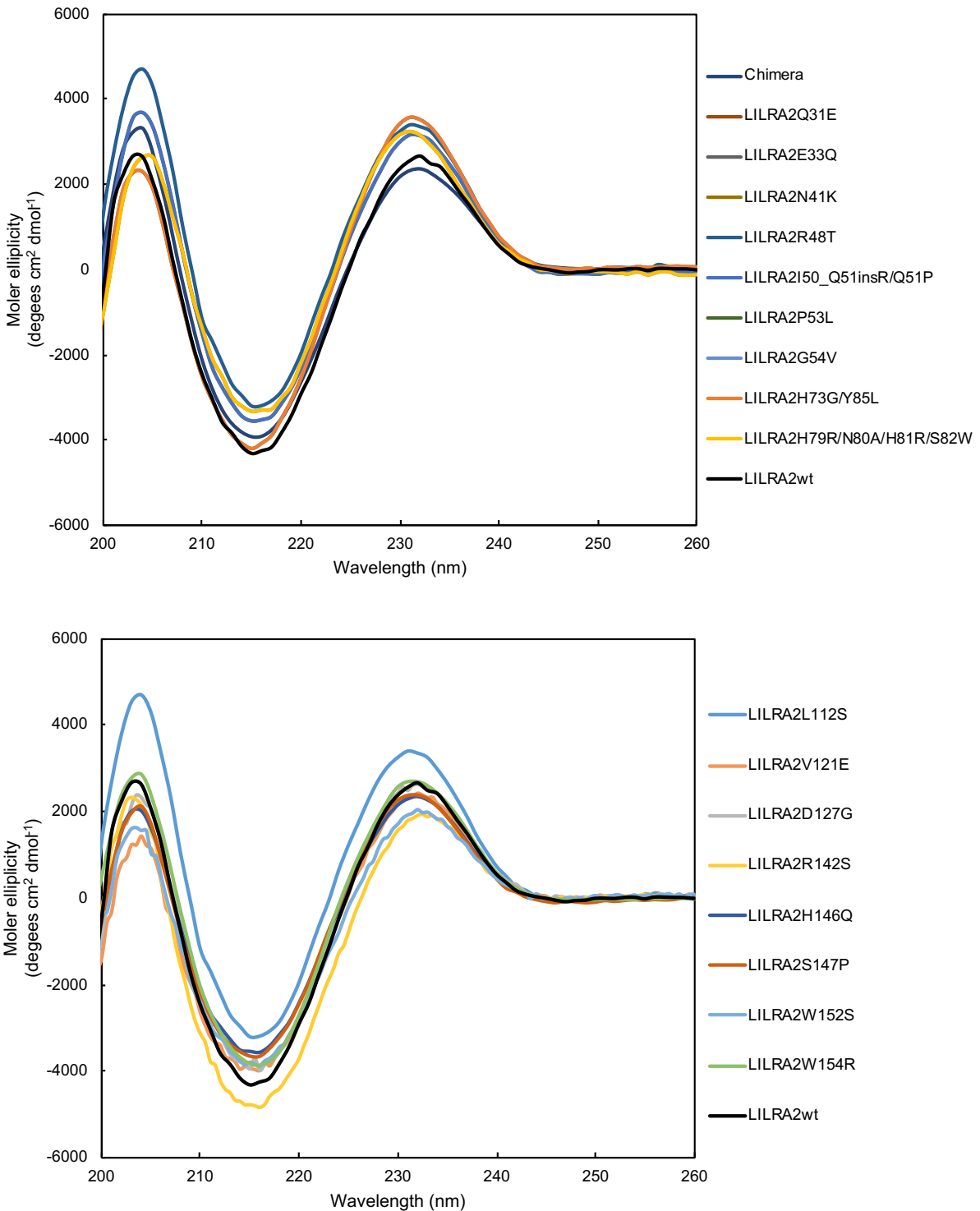
Figure. S5. Circular dichroism (CD) spectra of LILRA2 wt and LILRA2 mutants.
