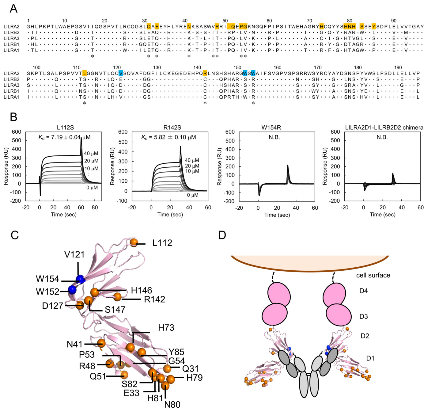
Figure 4. Mutagenesis analysis for LILRA2 binding mode toward N-truncated Ig. A, Alignment of group 1 LILRs. The asterisks below the sequence indicate the LILRA2 unique residues among group 1 LILRs. The mutated residues that did not affect N-truncated Ig binding are shown with orange background. The identified residues involved in ligand binding are shown with blue background. B, Mutagenesis analysis using SPR. LILRA2 mutants were injected onto N-truncated Ig immobilized chip. K_d value is presented as mean \pm range from two experiments or mean \pm standard deviation from three experiments. N.B. means no detectable binding. C, Mapping of mutated amino acid residues of LILRA2. Blue spheres represent the residues that are involved in N-truncated Ig binding. Orange spheres represent the residues that are not involved in N-truncated Ig binding. The structure was based on LILRB2 (PDB entry 2GW5). D, Proposed model of N-truncated Ig recognition by LILRA2.
