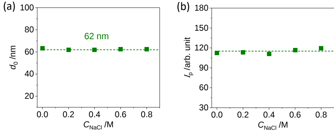
Figure 8. Effect of dialysis kinetics on phase structure of PA gel. The as-prepared gels were first dialyzed in NaCl solutions of prescribed concentrations ( C_{\text{NaCl}} ) at room temperature for one week, and then were dialyzed in pure water for another week. After that, SAXS was used to measure the phase structure of these gels. (a) d -spacing and (b) peak intensity of the gels against the NaCl concentration of dialysis solution. The gel is P(NaSS-co-DMAEA-Q)-2.6-0.1.
