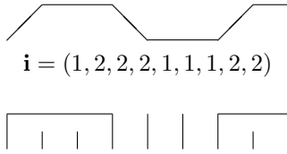
Figure 1. \pi(1, 2, 2, 2, 1, 1, 1, 2, 2) .
