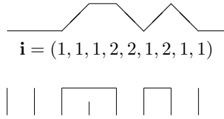
Figure 2. \pi(1, 1, 1, 2, 2, 1, 2, 1, 1) .
