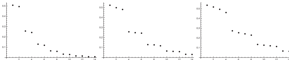
Figure 3. Eigenvalues \lambda_1, \dots, \lambda_{14} of \left\{D + \sum_{i=1}^k U_i D U_i^*\right\}_{k=1,2,3} ( n = 1000 ).
