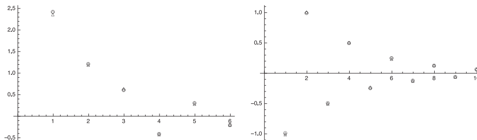
Figure 4. Left: comparing \text{EV}(AB + BA) (triangle), \text{EV}(pA) \sqcup \text{EV}(qA) (circle) and the theoretical limiting eigenvalues (square). Right: comparing \text{EV}(i(AB - BA)) (triangle), \text{EV}(rA) \sqcup \text{EV}(-rA) (circle) and the theoretical limiting eigenvalues (square).
