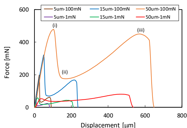
Figure 2. Relationship between the force and displacement measured using a glass sphere
