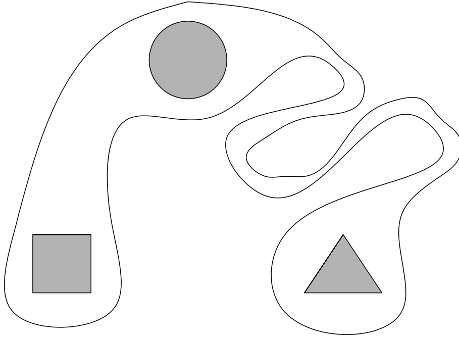
Figure 4: D_0 and O_- that do not satisfy the assumptions of Theorem 3.6
