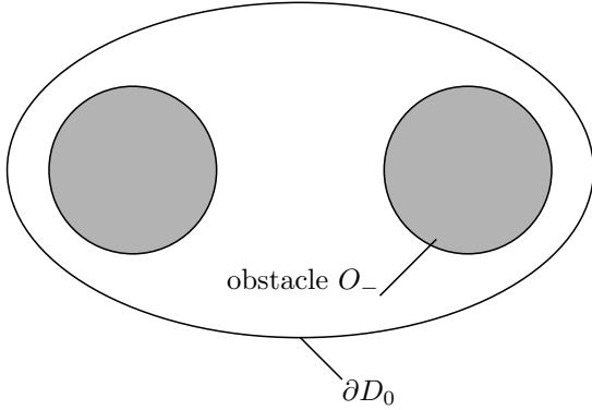
Figure 1: D_0 contains \text{Conv}(O_-)
