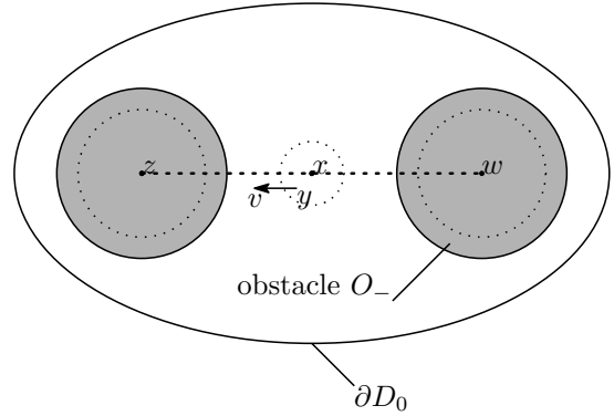
Figure 2: A strategy of Player I
