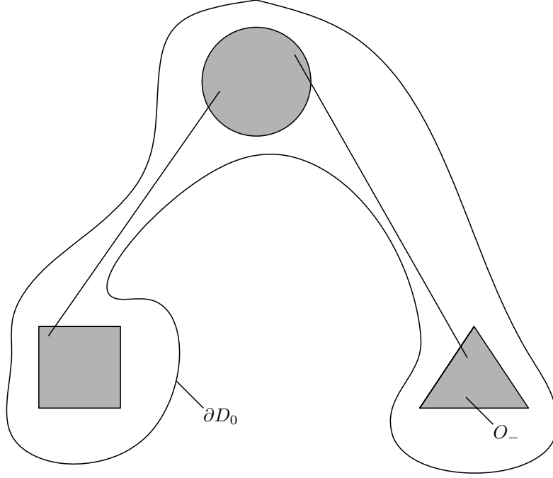
Figure 3: D_0 and O_- that satisfy the assumptions of Theorem 3.6
