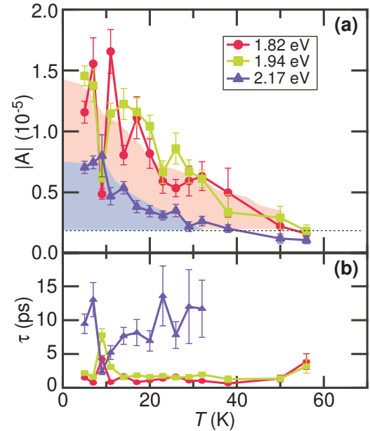
Fig. 3 (a) Temperature dependences of signal amplitude at 1.82 eV, 1.94 eV and 2.17 eV. The dashed line indicates a noise level. (b) Temperature dependences of decay time at 1.82 eV, 1.94 eV and 2.17 eV. A slight enhancement of \tau in 1.82 eV and 1.94 eV channels at 56 K is probably an artifact related with the fitting because the signal tends to be buried in the noise.
