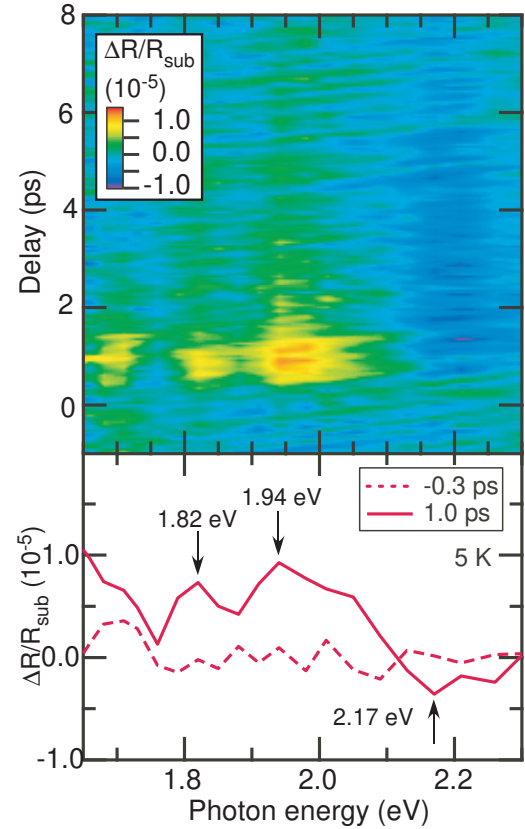
Fig. 1 An intensity plot of transient change of reflectivity \Delta R/R_{\text{sub}} as a function of probe photon energy at 5 K and probe photon energy spectra of \Delta R/R_{\text{sub}} at -0.3 ps (dashed line) and 1.0 ps (solid line). Note that \Delta R/R_{\text{sub}} was obtained by subtracting the data at 122 K.
