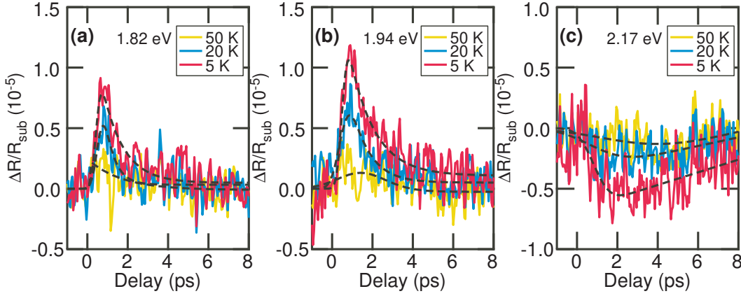
Fig. 2 (a)-(c): \Delta R/R_{\text{sub}} at 1.82 eV, 1.94 eV and 2.17 eV for various temperatures, respectively.
