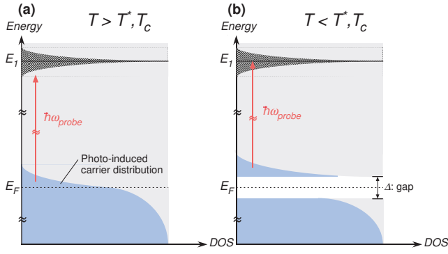
Fig. 4 Schematic illustrations of the optical transition in the probe process at (a) T > T^*, T_c and (b) T < T^*, T_c . E_1 and E_F denote an intramolecular excitation energy and the Fermi energy, respectively.
