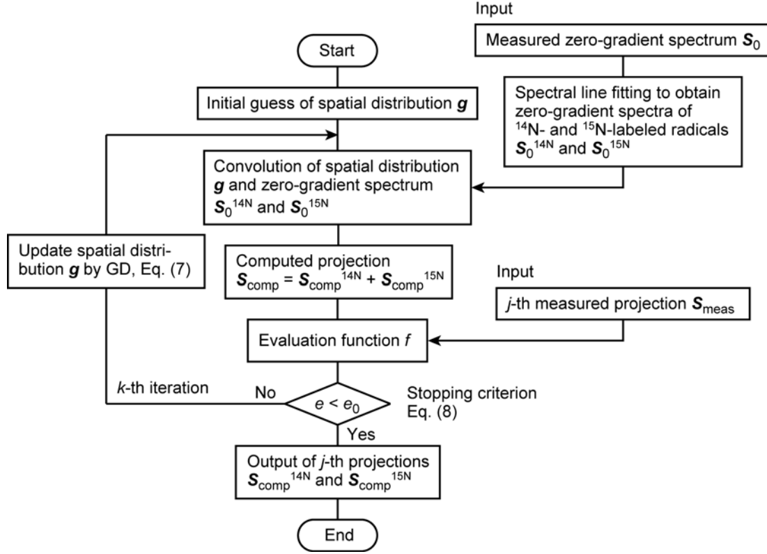
Fig. 2. Flowchart of the spectral projection separation process for ^{14}\text{N} - and ^{15}\text{N} -labeled nitroxyl radicals.
