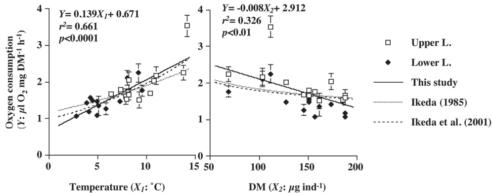
Fig. 2. Metridia pacifica adult females. Relationship between weight-specific oxygen consumption and experimental temperature (left), and weight-specific oxygen consumption and dry mass (right). Significant interactions were observed for both relationships. For comparison, regression lines from Ikeda (1985) and Ikeda et al. (2001) are also shown in the panels.
