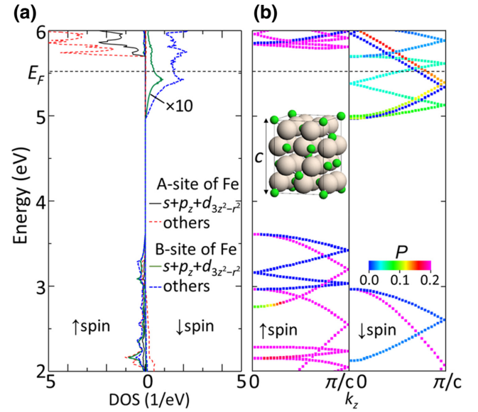
FIG. 6. Calculation results of (a) spin-dependent local density of states (DOS) and (b) E-k dispersion relation between \mathbf{k} = (0, 0, 0) and \mathbf{k} = (0, 0, \pi/c) . The unit cell for E-k calculations is shown in (b). In (a), the DOS of the sum of the s , p_z , and d_{3z^2-r^2} orbitals (the coherent orbitals) of the B site of Fe ions in the conduction band is shown magnified 10 times. The percentages of the summation of the coherent orbitals ( P ), which are hybridized with the wave functions transmitted through \text{MgO} in an \text{Fe}_3\text{O}_4/\text{MgO}/\text{Fe} junction, are plotted in color.
