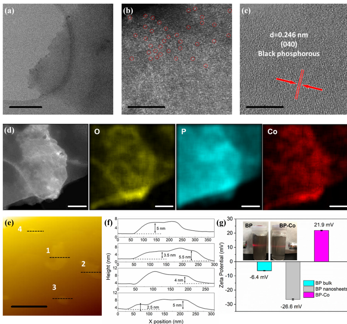
Figure 2. (a) Low resolution TEM (scale bar 100 nm), (b) HADDF-STEM (scale bar 5 nm) image (Co atoms are marked using red circles), (c) HRTEM image (scale bar 5 nm) with d-spacing 0.246 nm of BP-Co material. (d) EDS mapping images of as-prepared BP-Co material (scale bar 100 nm). (e) Tapping-mode AFM image (scale bar 500 nm) and (f) the related cross-sectional analysis (line 1 to line 4) of BP-Co. (g) Zeta-potential of BP bulk, freshly prepared BP nanosheets and BP-Co tested in ethanol solution. (Inset image: Observation of Tyndall effect of freshly prepared BP nanosheets and BP-Co dispersed in water.)
