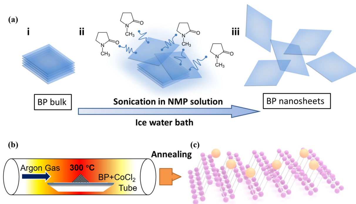
Figure 1. (a) Schematic illustration of NMP liquid solution assisted probe sonication exfoliation route in ice water bath to prepare few-layer BP nanosheets. (b) Proposed strategy to obtain uniform dispersed Co on BP nanosheets substrate. (c) Atomic structure of single atom dispersed BP nanosheets.
