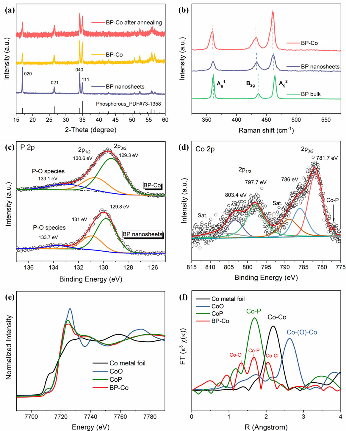
Figure 3. (a) XRD analysis of BP nanosheets and BP-Co before and after annealing process. (b) Raman spectra of BP bulk, BP nanosheets and BP-Co. (c) P 2p and (d) Co 2p binding energy spectra. (e) Co K-edge XANES spectra and (f) Fourier transform magnitudes of the experimental Co K-edge EXAFS spectra of BP-Co and reference samples.
