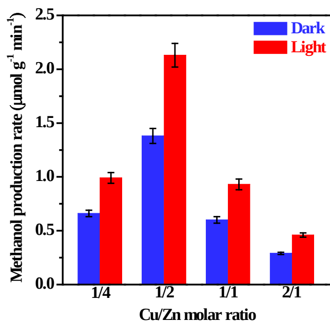
Fig. S11. Methanol production rate at 220 °C over Cu/ZnO catalysts with various Cu/Zn molar ratios.
