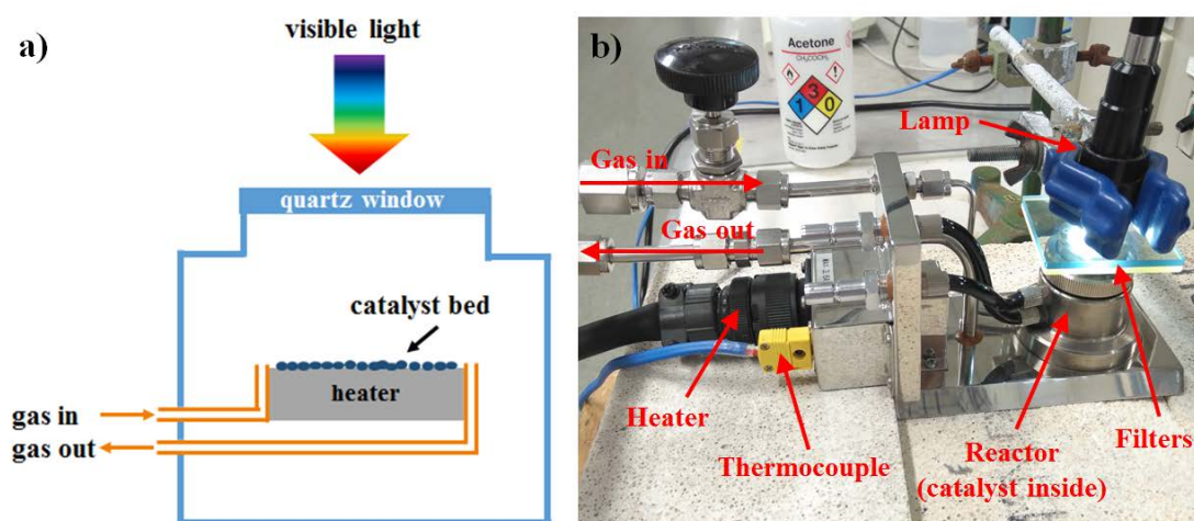
Fig. S1. Schematic of homemade fixed bed reactor (a) and photograph of reaction test setup (b)
