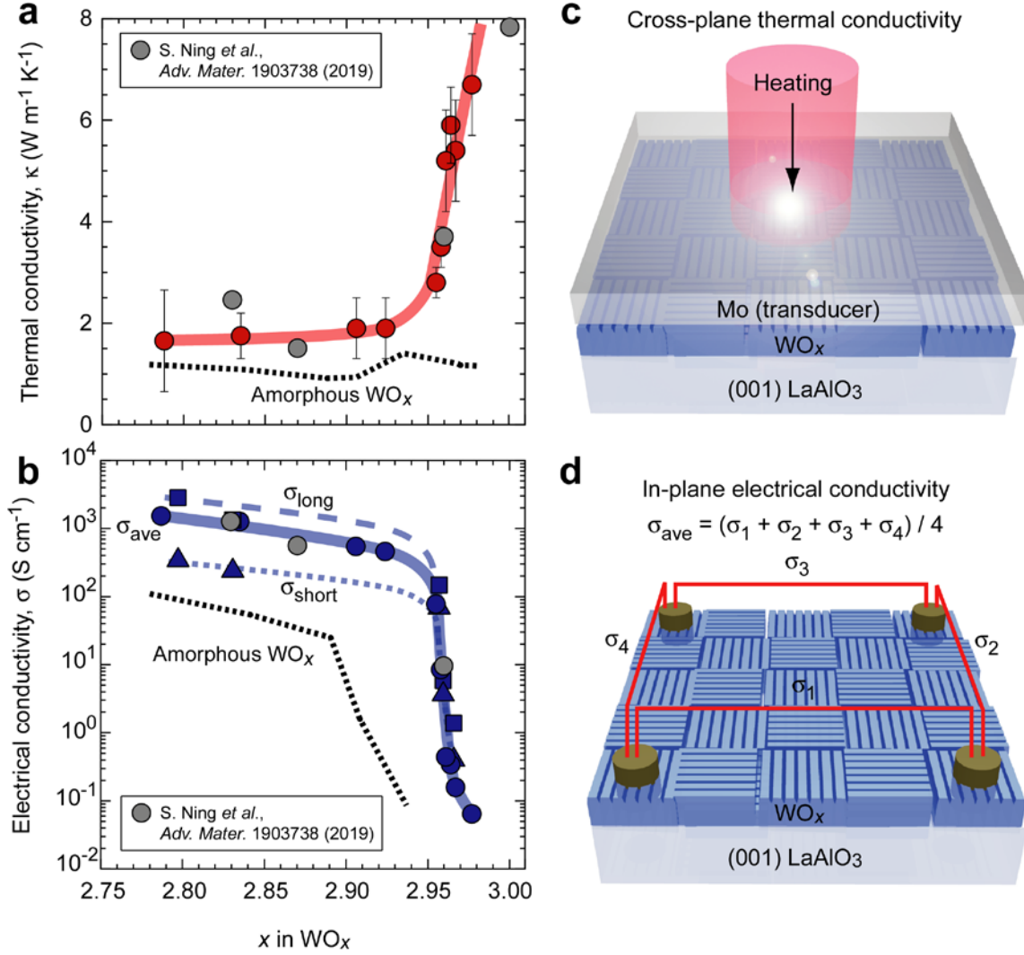
Figure 4. Coexistence of high electron conduction and low heat conduction in the \text{WO}_x epitaxial films with 1D atomic defect tunnels. (a) Cross-plane thermal conductivity \kappa extracted from the TDTR measurement. The \kappa of amorphous \text{WO}_x films 22 and epitaxial \text{WO}_x films 21 are also plotted. (b) In-plane electrical conductivity \sigma . The \sigma of amorphous \text{WO}_x films 22 and epitaxial \text{WO}_x films 21 are also plotted. (c) Schematic illustration of the TDTR measurement of the \text{WO}_x films. (d) Schematic illustration of the electrical conductivity measurement of the \text{WO}_x films.
