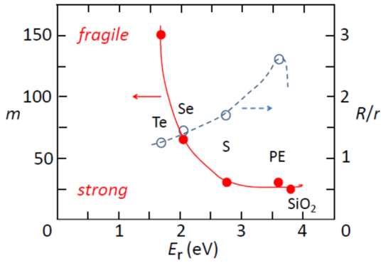
Fig. 2. The fragility m and a distance ratio R/r as a function of the covalent bond strength E_r (the data from Table 1).
