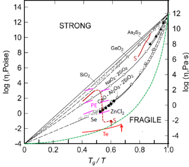
Fig. 1. Viscosities \eta(T_g/T) for \text{SiO}_2 and Se, [2] with additions of S (brown), [38,40,41] Te (red), [48] and PEs (violet) [59] with n \approx 300, 800 , and 2000 (from low to upper) for T_g = 200 and 250 K (left and right). Arrows indicate T_m positions, and a dashed green line shows the \eta variation with m = 150 .
