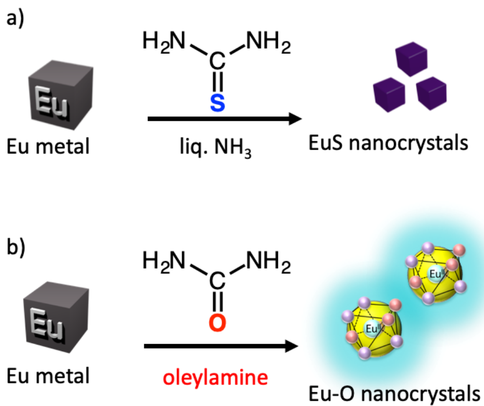
Figure 1. Conceptual synthetic schemes of Eu-S and Eu-O nanocrystals.
