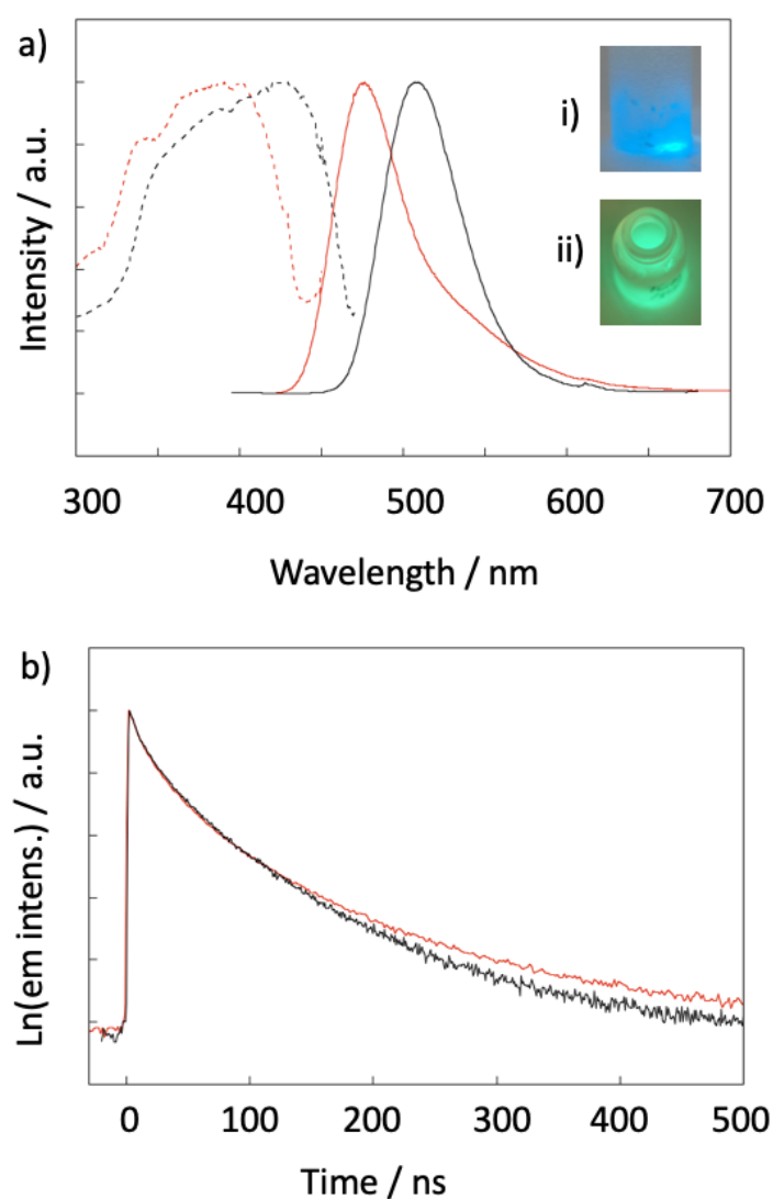
Figure 4. a) Emission and excitation spectra of i) \text{Eu}(\text{OCN})_2 nanocrystals (red line) and ii) \text{Eu}(\text{OCN})_2 -urea (black line). b) Emission decay profiles of \text{Eu}(\text{OCN})_2 -urea (black line) and (ii) \text{Eu}(\text{OCN})_2 nanocrystals (red line).
