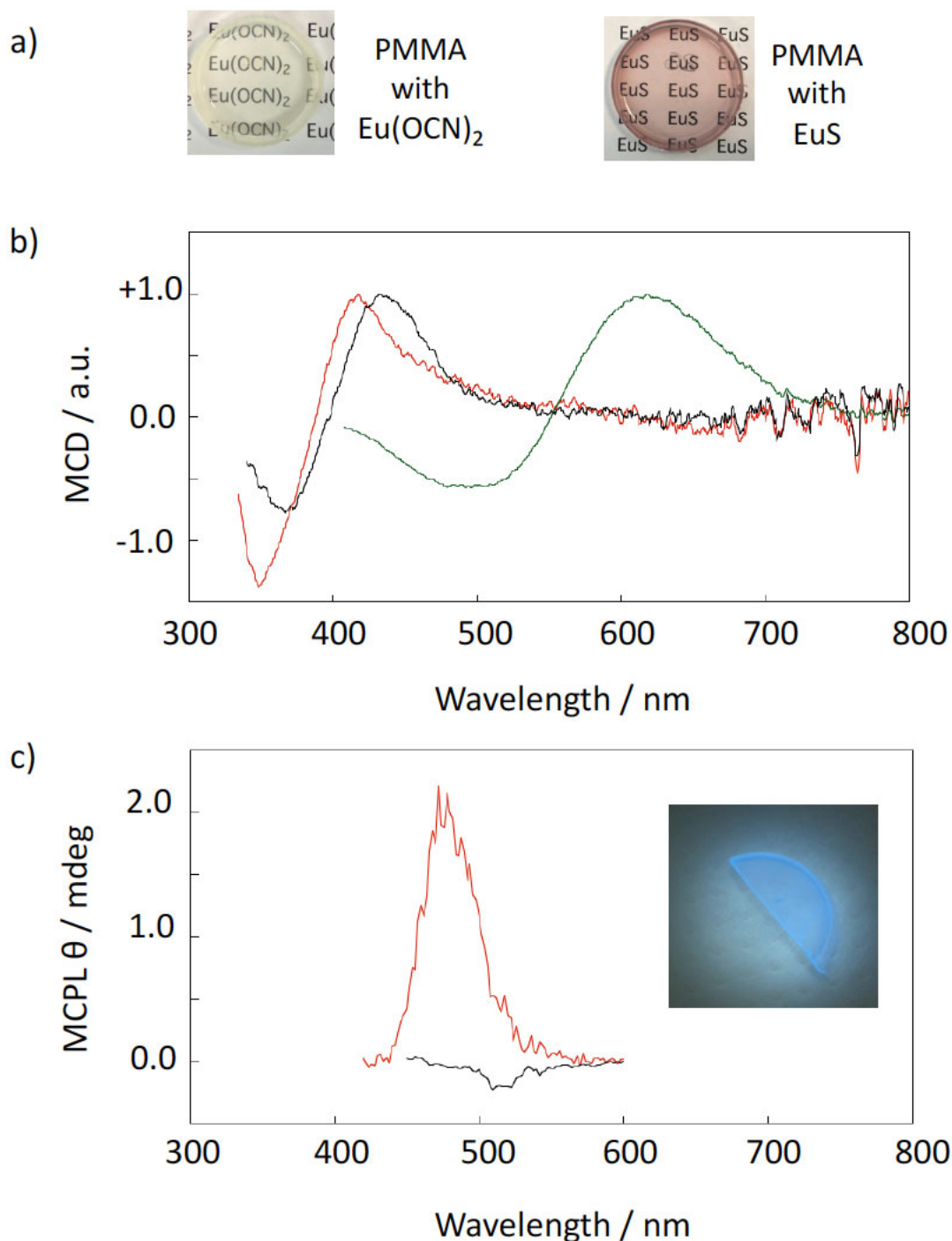
Figure 5. a) Image pictures of PMMA disks containing \text{Eu(OCN)}_2 and \text{EuS} nanocrystals. b) Circularly polarized absorption (CD) spectra of \text{Eu(OCN)}_2 (red line), \text{Eu(OCN)}_2 -urea (black line) and \text{EuS} (green line) nanocrystals under 1.6 T. Concentration of nanocrystals in polymer films: 0.5wt%. c) Circularly polarized luminescence (CPL) of PMMA disks containing \text{Eu(OCN)}_2 (red line) and \text{Eu(OCN)}_2 -urea (black line) under 1.6 T. Inset picture is a luminescent PMMA disk containing \text{Eu(OCN)}_2 under 100K.
