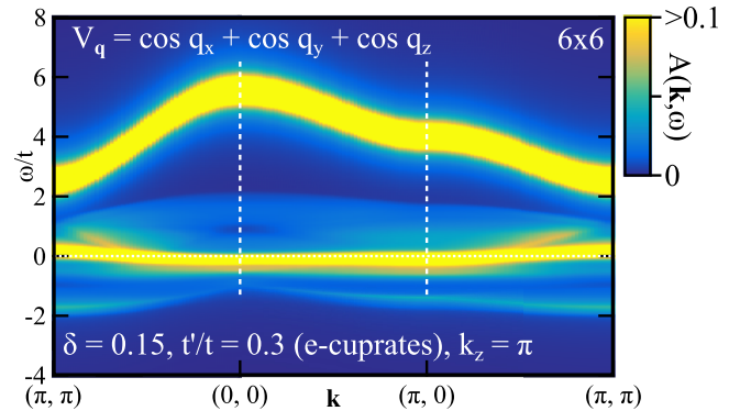
FIG. 17. Intensity map of A(\mathbf{k}, \omega) in the absence of the long-range Coulomb interaction along the direction (\pi, \pi) \rightarrow (0, 0) \rightarrow (\pi, 0) \rightarrow (\pi, \pi) in the particle picture; both on-site charge and bond-charge fluctuations are taken into account. k_z dependence is weak and k_z = \pi is taken as a representative value. The corresponding result in the hole picture is presented in Fig. 13.
