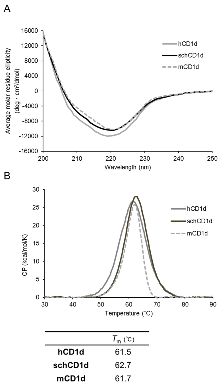
Fig. 6. Characterization of CD1d. (A) CD spectrum of CD1d proteins. (B) DSC curves and T_m value of CD1d proteins.
