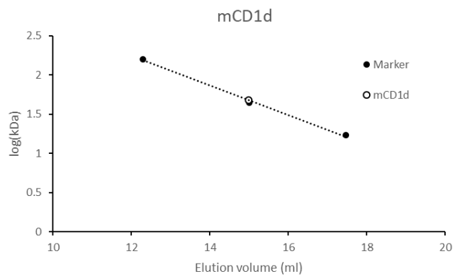
Supplementary Fig. 2. Standard curve for size exclusion chromatography. The filled circles indicate the positions of the protein standard. The open circles indicate the positions of peak of (A) hCD1d, (B) schCD1d and (C) mCD1d, respectively.
