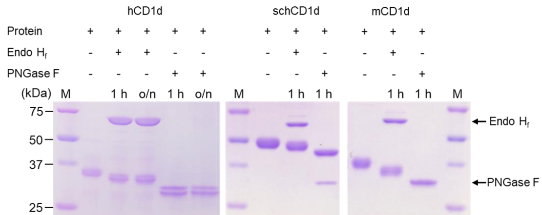
Fig. 5. SDS-PAGE images analyzing the CD1d digested by endoglycosidases. End H f digestion splits hCD1d (left) into two bands, and hCD1d became one band in the lower position due to digestion of PNGase F. The upper band of PNGase F + hCD1d is PNGase F. The schCD1d (middle) and the mCD1d (right) were digested similarly to hCD1d. The band of mCD1d digested by PNGase F overlaps with the band of PNGase F.
