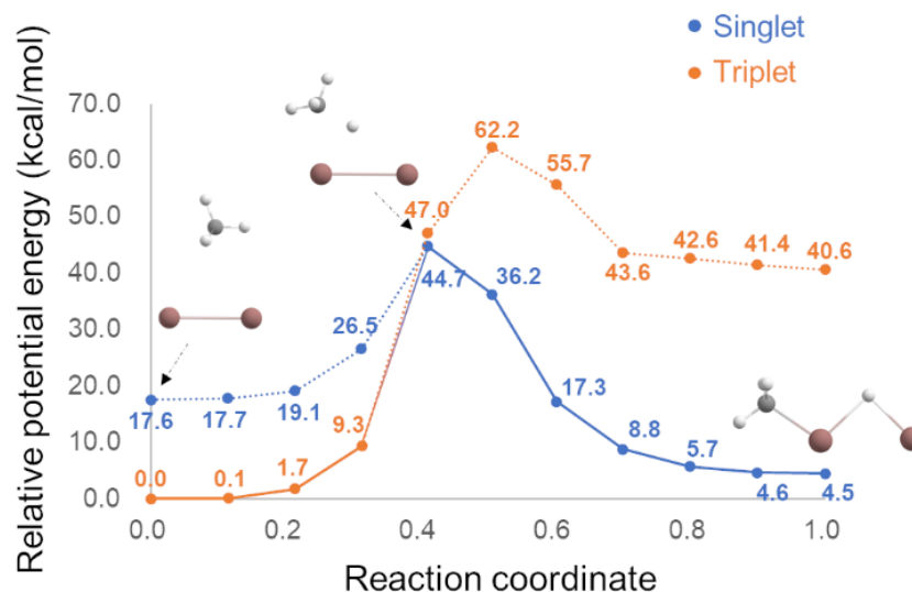
(a) Intermediate image number equals to 9
