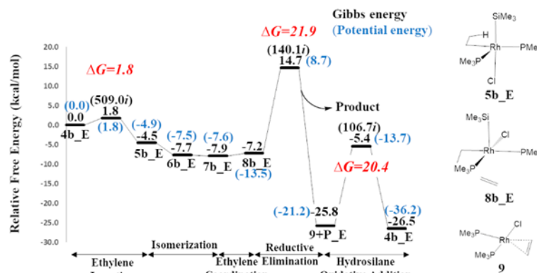
Figure 6 Gibbs free energy profile for the CH mechanism in ethylene hydrosilylation.
