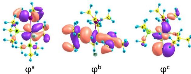
Figure 9 Important molecular orbitals of 4a'_E ( \phi^a ) and 4c ( \phi^b and \phi^c )
