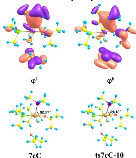
Figure 5 Interactions between Si and O in 7cC ( \phi^i ), ts7cC-10 ( \phi^k ).
