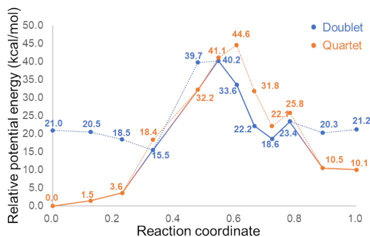
Figure 12 Relative potential energy profile of \text{CoH}^+ -catalyzed methane activation. Calculated by using two-image-selection scheme.
