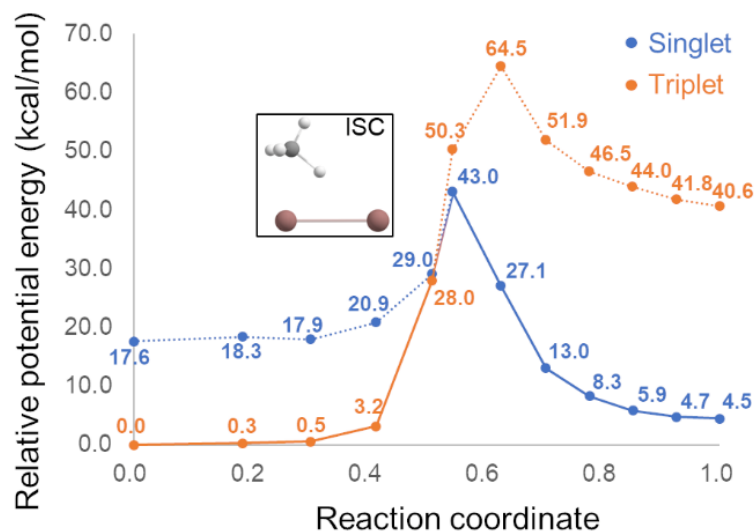
Figure 6 (a)Relative potential energy profile of \text{In}_2 -catalyzed C-H bond activation with 9 intermediate images (No image was optimized as ISC point). (b) Relative potential energy profile of \text{In}_2 -catalyzed C-H bond activation with 10 intermediate images (One image was optimized as ISC point).
