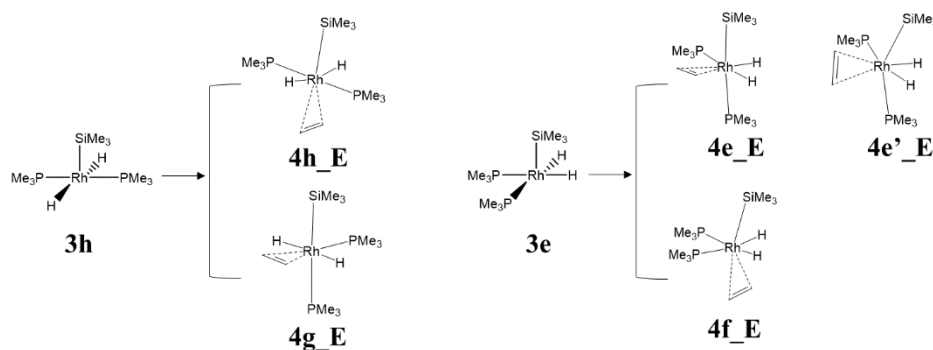
Figure 14 Possible isomers after the ethylene coordination to 3h (left) and 3e (right).
