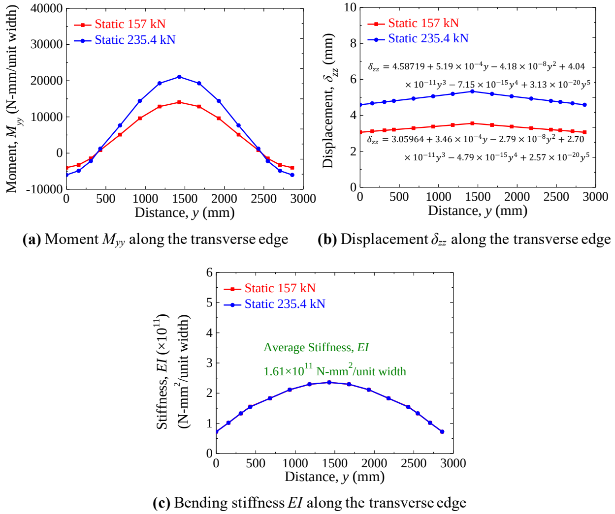
Figure 5.3 Bending stiffness EI along the transverse edge of the panel slab (load at location D)
