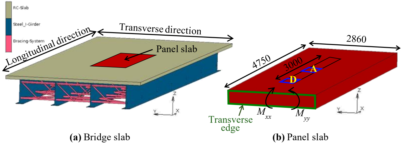
Figure 5.1 Illustration of the bridge slab and its corresponding panel slab (mm)
