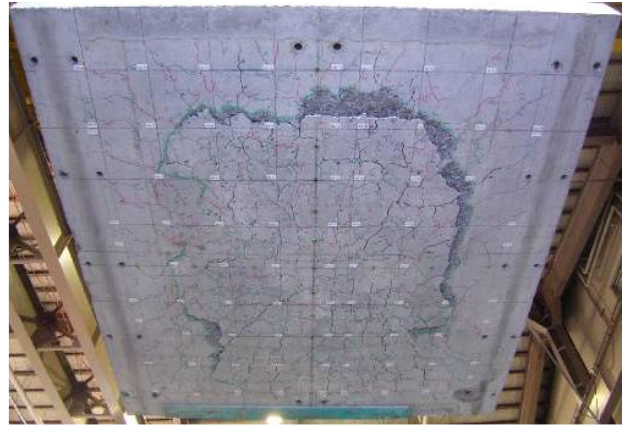
(b) Punching shear failure at the bottom surface of the panel RC slab
