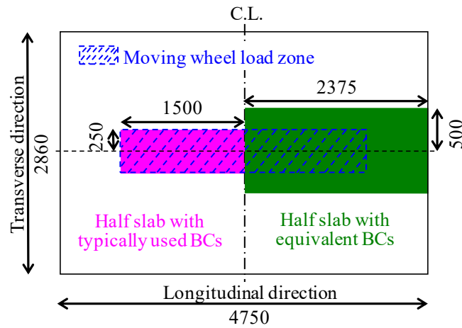
Figure 6.11 Grid crack pattern zone (mm)
