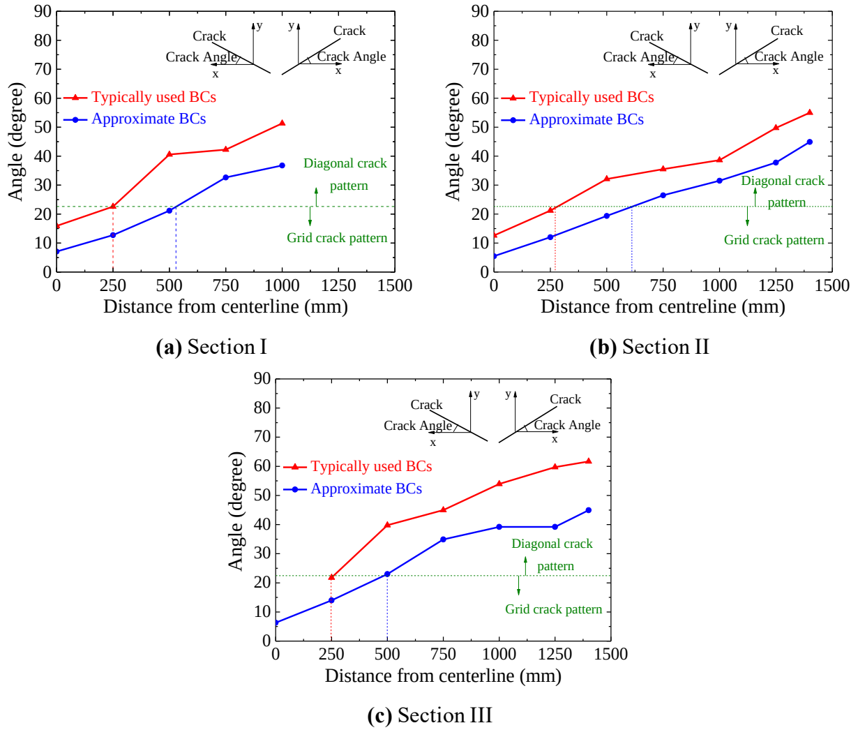
Figure 4.9 Crack angle along the transverse direction
