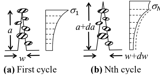
Figure 2.3 Crack propagation due to bridging stress degradation
