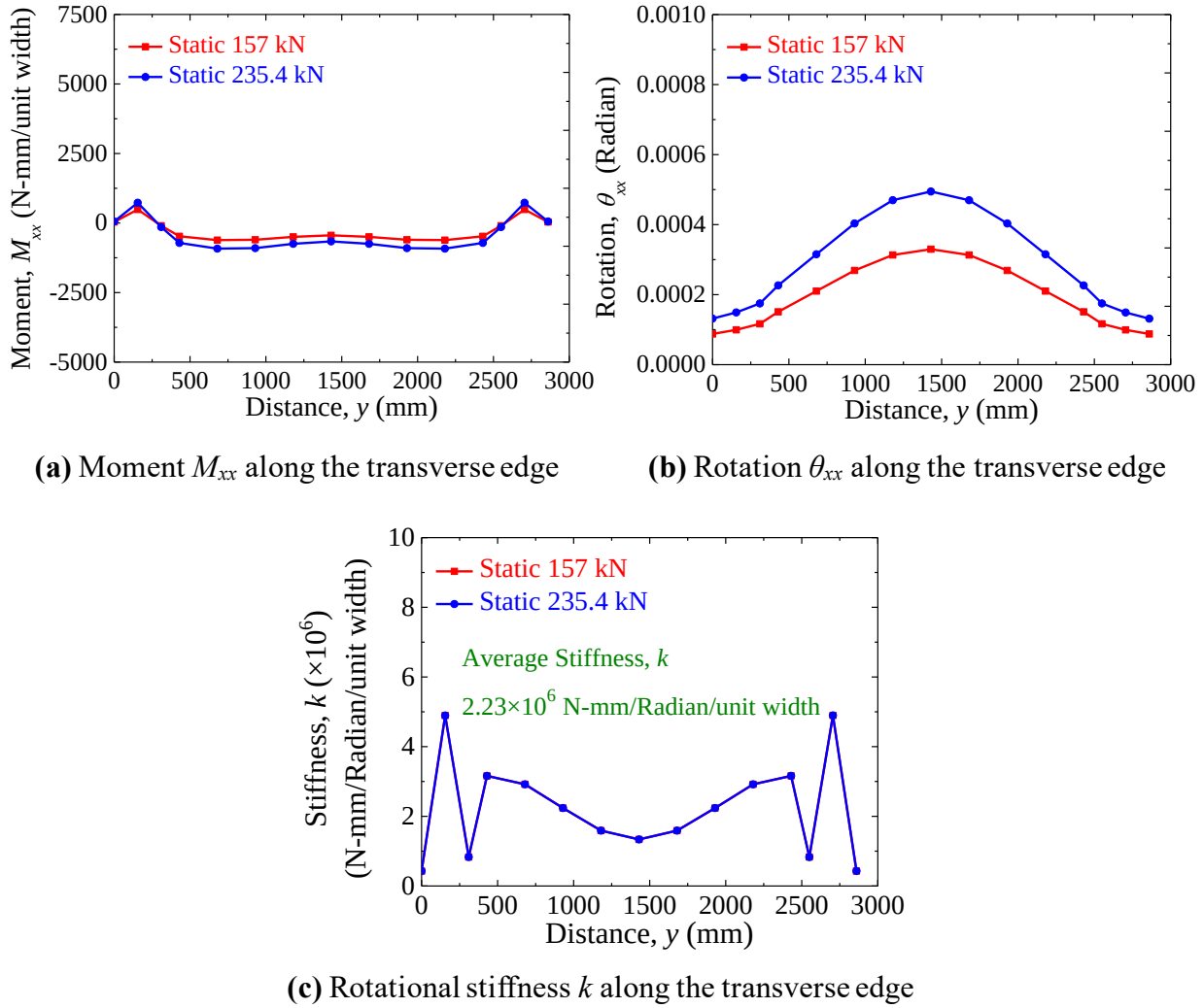
Figure 5.5 Rotational stiffness k along the transverse edge of the panel slab (load at location D)
