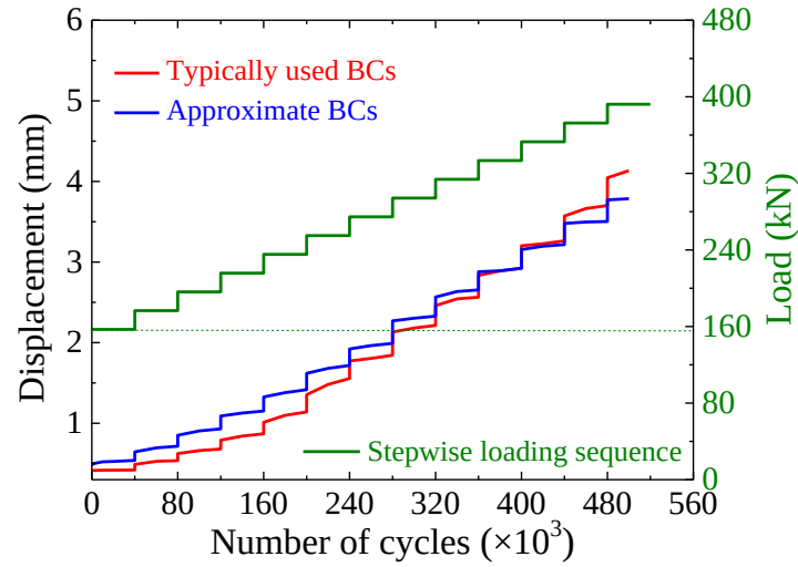
Figure 4.6 Center displacement evolution
