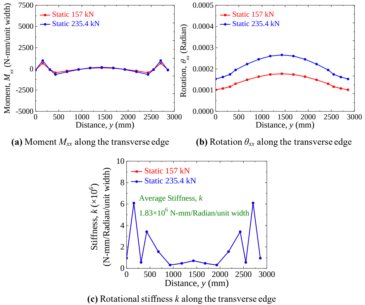
Figure 5.4 Rotational stiffness k along the transverse edge of the panel slab (load at location A)
