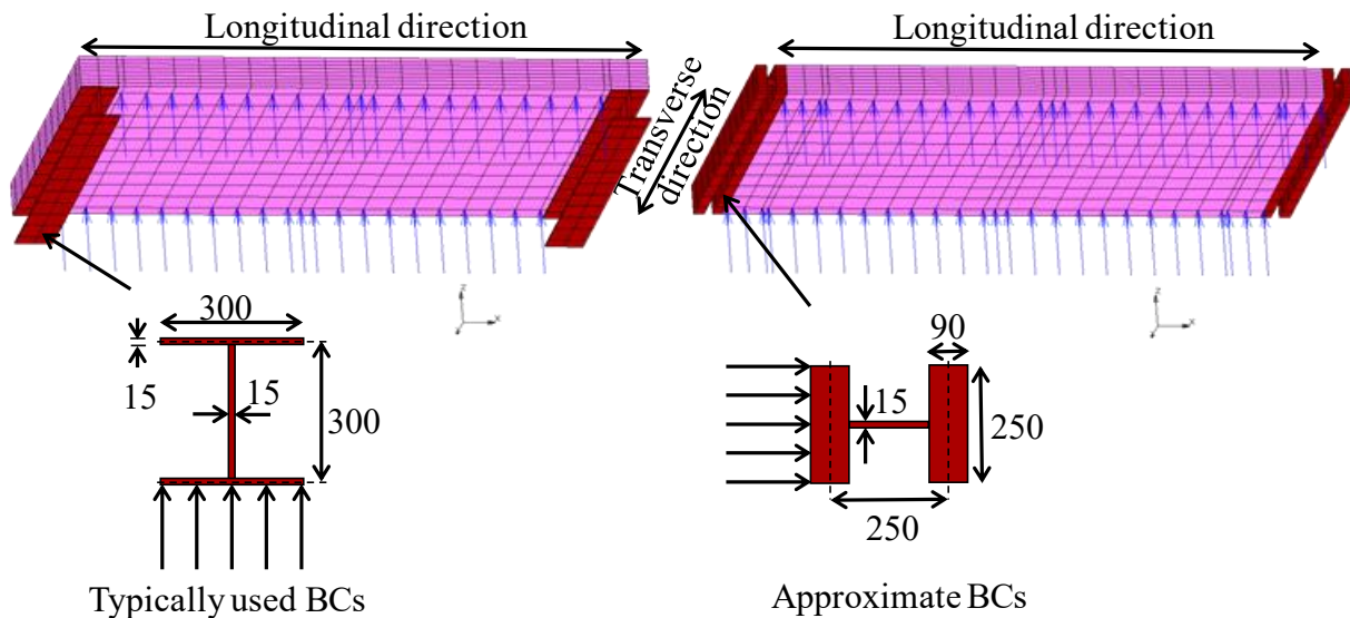
Figure 4.1 Illustration of BCs (mm)
