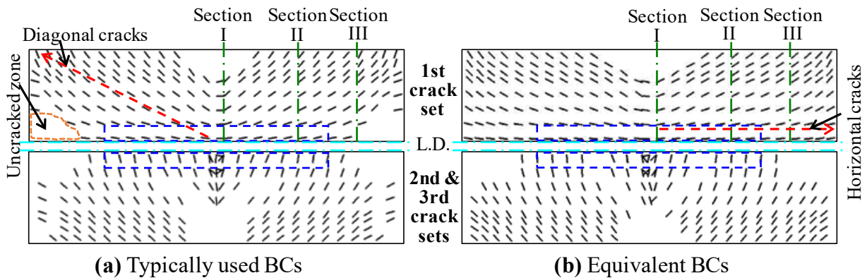
Figure 6.9 Crack patterns
