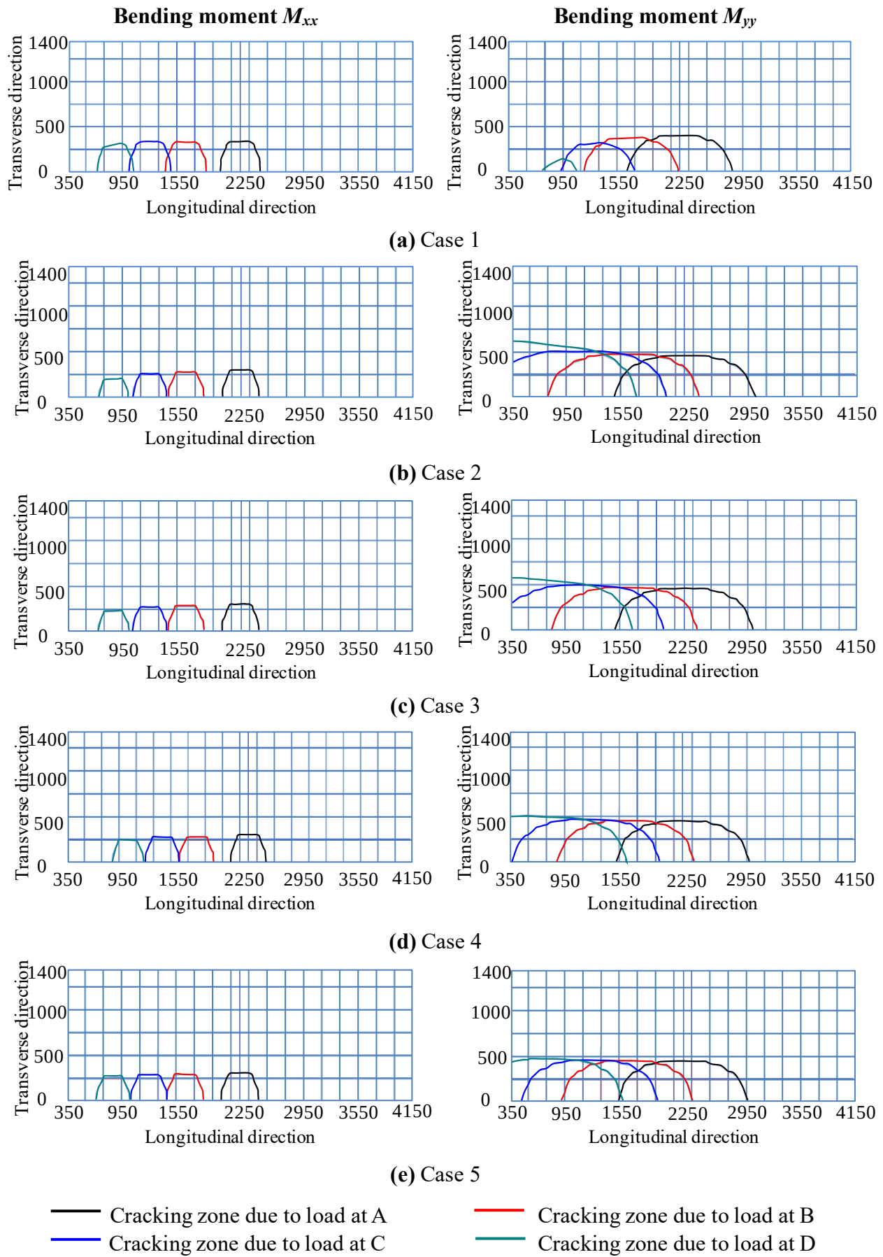
Figure 3.6 Bending moment cracking zones
