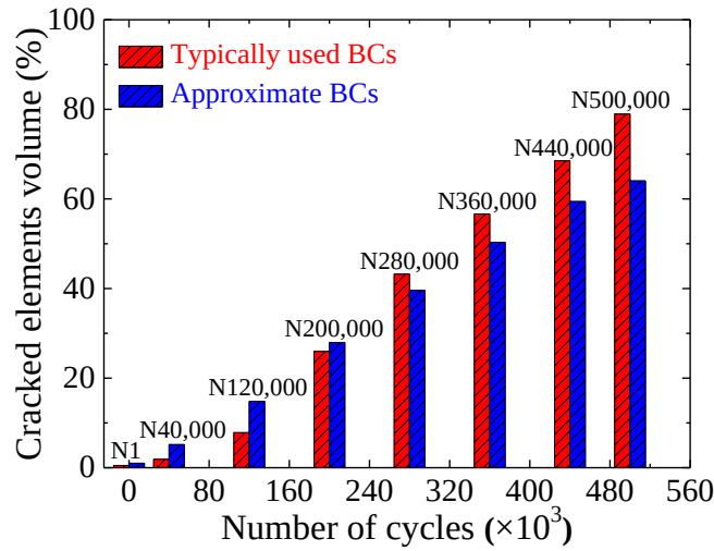
Figure 4.4 Percentage of the volume of cracked elements
