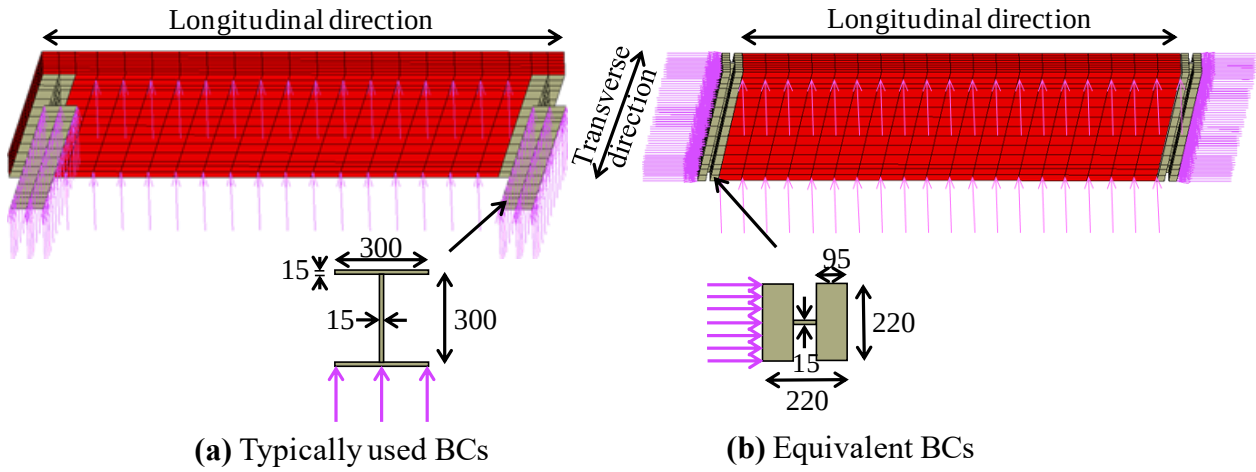
Figure 6.2 Illustration of the boundary conditions (mm)
