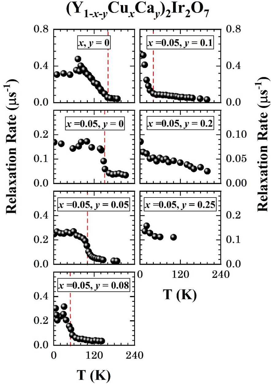
Fig. 3.10. The temperature dependence of the relaxation rate of (Y_{1-x-y}Cu_xCa_y)_2Ir_2O_7 .
