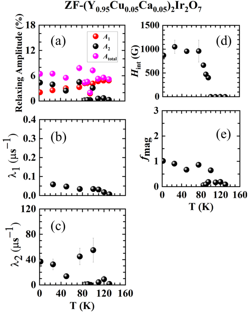
Fig. 3.15. Temperature dependences of (a) initial asymmetry of each component, (b) slow-relaxation rate \lambda_1 , (c) fast-relaxation rate \lambda_2 , (d) internal field H_{\text{int}} at muon sites and (e) magnetic volume fraction f_{\text{mag}} of (Y 0.95 Cu 0.05 Ca 0.05 ) 2 Ir 2 O 7 .
