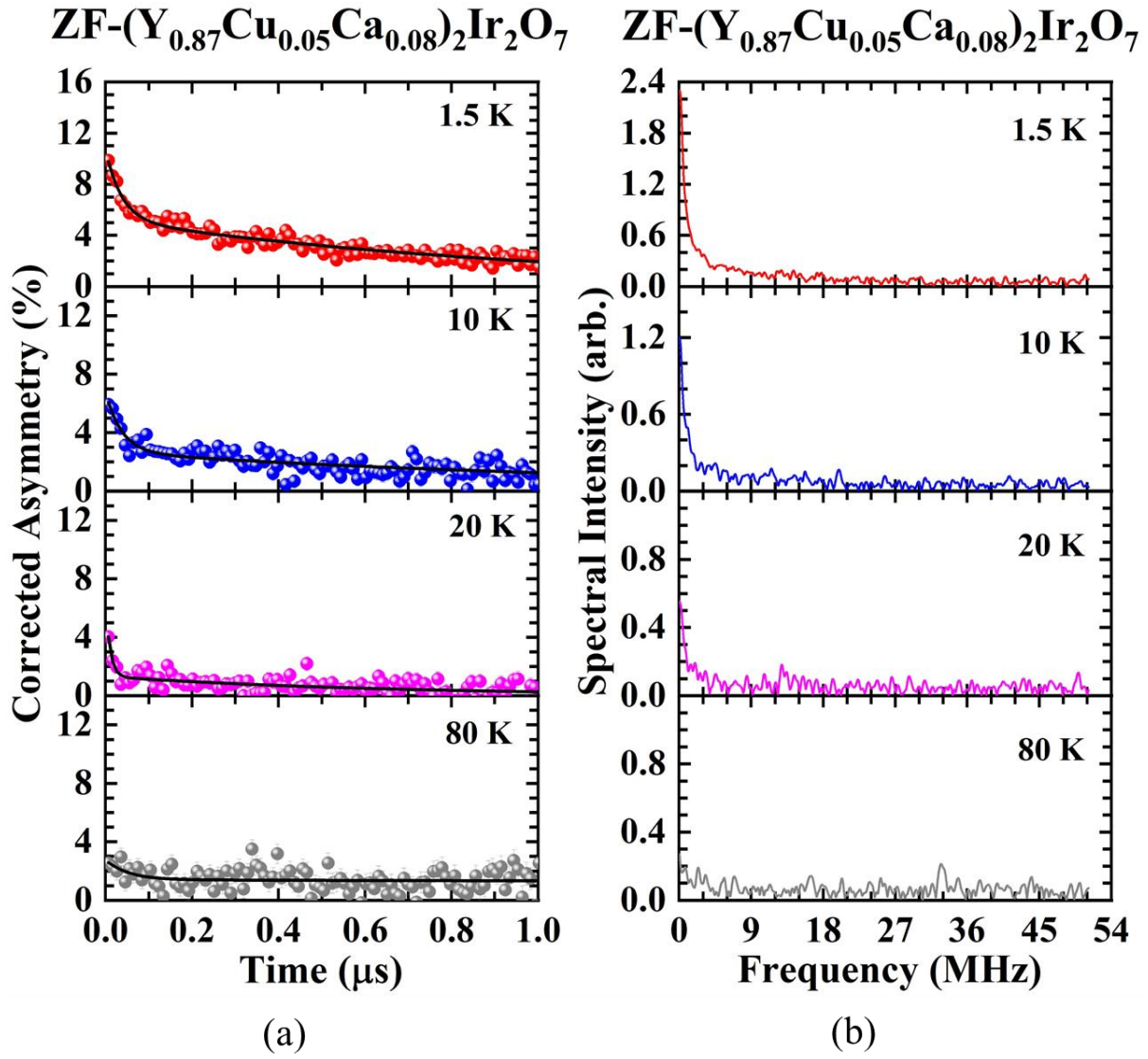
Fig. 3.16. (a) ZF- \mu SR time spectra and (b) FFT plot of ZF- \mu SR time spectra of (Y_{0.87}Cu_{0.05}Ca_{0.08})_2Ir_2O_7 ( (Y_{1-x-y}Cu_xCa_y)_2Ir_2O_7 with x = 0.05 , y = 0.08 ). Solid lines are fits to Eq. (3.4) as described in the text.
