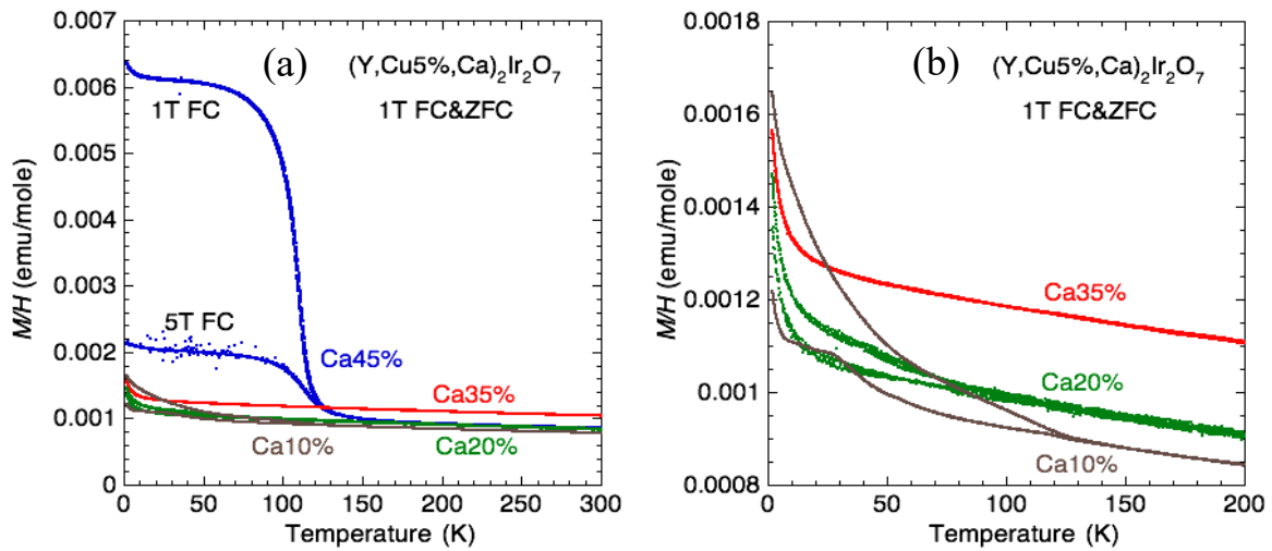
Fig. A.1. (a) Magnetic susceptibility of (Y_{1-x-y}Cu_xCa_y)_2Ir_2O_7 with x = 0.05 ; y = 0.10, 0.20, 0.35 , and 0.45 . (b) magnification of (a), except (Y_{0.5}Cu_{0.05}Ca_{0.45})_2Ir_2O_7 . Figure is provided by Dr. K. Matsuhira.
