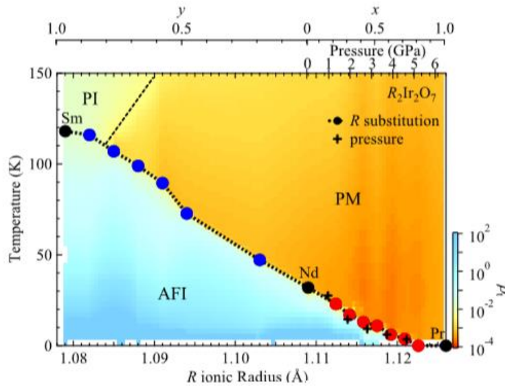
Fig. 1.10. Contour map in the plane of R ionic radius and temperature for resistivity in (Nd_xPr_{1-x})_2Ir_2O_7 and (Sm_yNd_{1-y})_2Ir_2O_7 . The color bar at the side of the map represents the magnitude of the resistivity, and the dots indicate the transition temperature [20].
