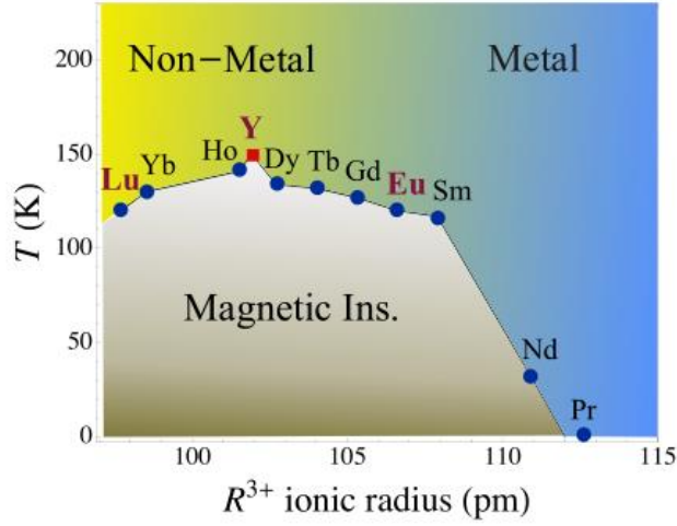
Fig. 1.9. Phase diagram of R277 according to transport and magnetic measurements, which is supplemented and modified from [15]. The R -elements that do not have a local magnetic moment are in bold magenta. The only non-lanthanide is denoted by a square ( R = Y ) [2].
