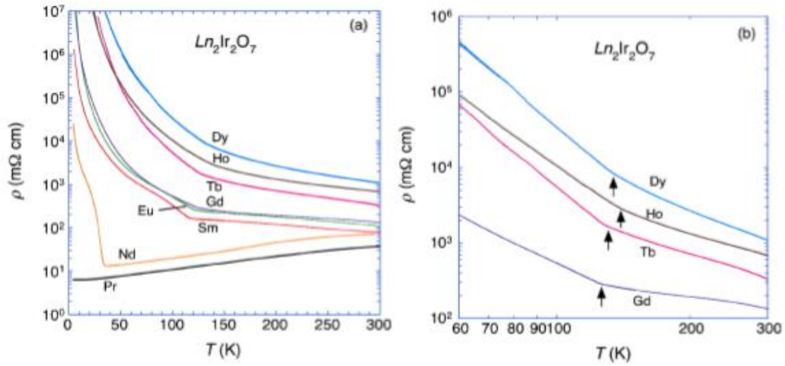
Fig. 1.7. (a) Electrical resistivities of R227 for R = \text{Pr} , \text{Nd} , \text{Sm} , \text{Eu} , \text{Gd} , \text{Tb} , \text{Dy} , and \text{Ho} . (b) enlarged view for R = \text{Gd} , \text{Tb} , \text{Dy} , and \text{Ho} [15].
