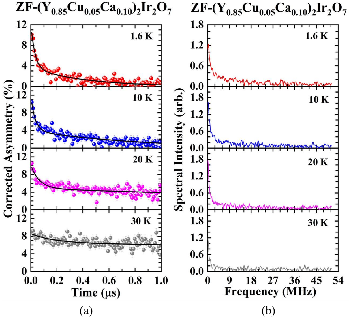
Fig. 3.18. (a) ZF-μSR time spectra and (b) FFT plot of ZF-μSR time spectra of (\text{Y}_{0.85}\text{Cu}_{0.05}\text{Ca}_{0.10})_2\text{Ir}_2\text{O}_7 ( (\text{Y}_{1-x-y}\text{Cu}_x\text{Ca}_y)_2\text{Ir}_2\text{O}_7 with x = 0.05 , y = 0.10 ). Solid lines are fits to Eq. (3.4) as explained in the text.
