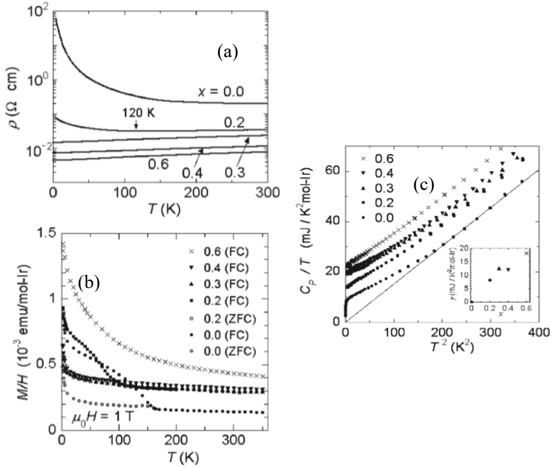
Fig. 1.12. (a) Resistivity and (b) magnetic susceptibilities of \text{Y}_{2-x}\text{Ca}_x\text{Ir}_2\text{O}_7 . Solid and open symbols denote the data obtained after field-cooling and after zero-field-cooling, respectively. (c) C_p/T vs. T^2 below 20 K; inset: \gamma vs. x [18].
