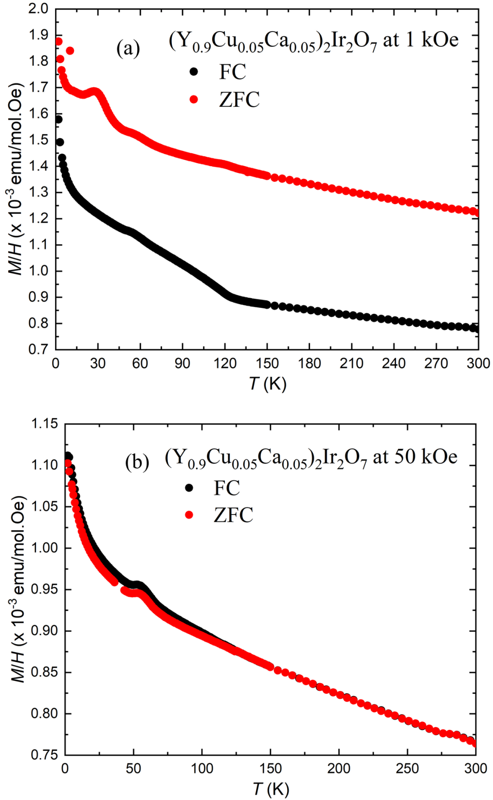
Fig. 3.4. Magnetic susceptibility of (Y_{1-x-y}Cu_xCa_y)_2Ir_2O_7 for x = 0.05 and y = 0.05 measured at Tokyo University of Science in (a) ZFC and FC conditions under 1 kOe and (b) ZFC and FC conditions under 50 kOe.
