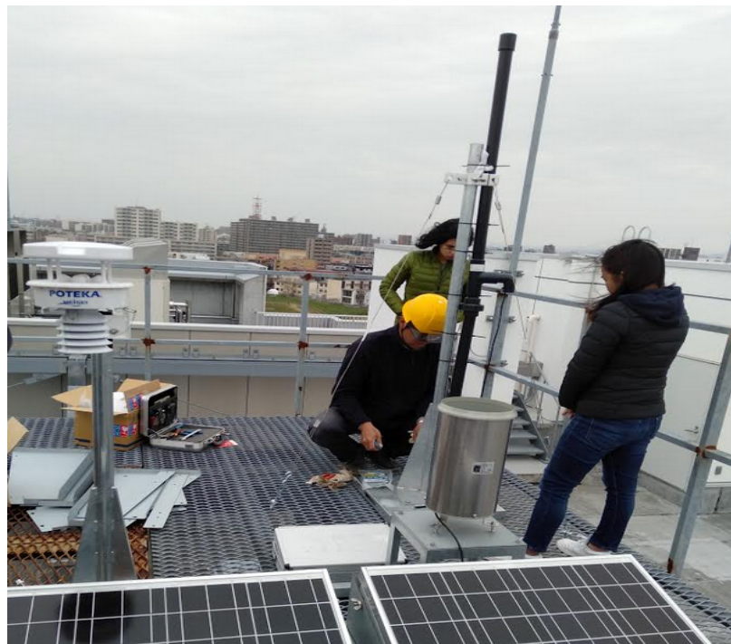
Figure 2.3. Example of V-POTEKA installed on roof top building of Hokkaido University. This kind of V-POTEKA is distributed to Philippines as Philippines Nation-wide Network
