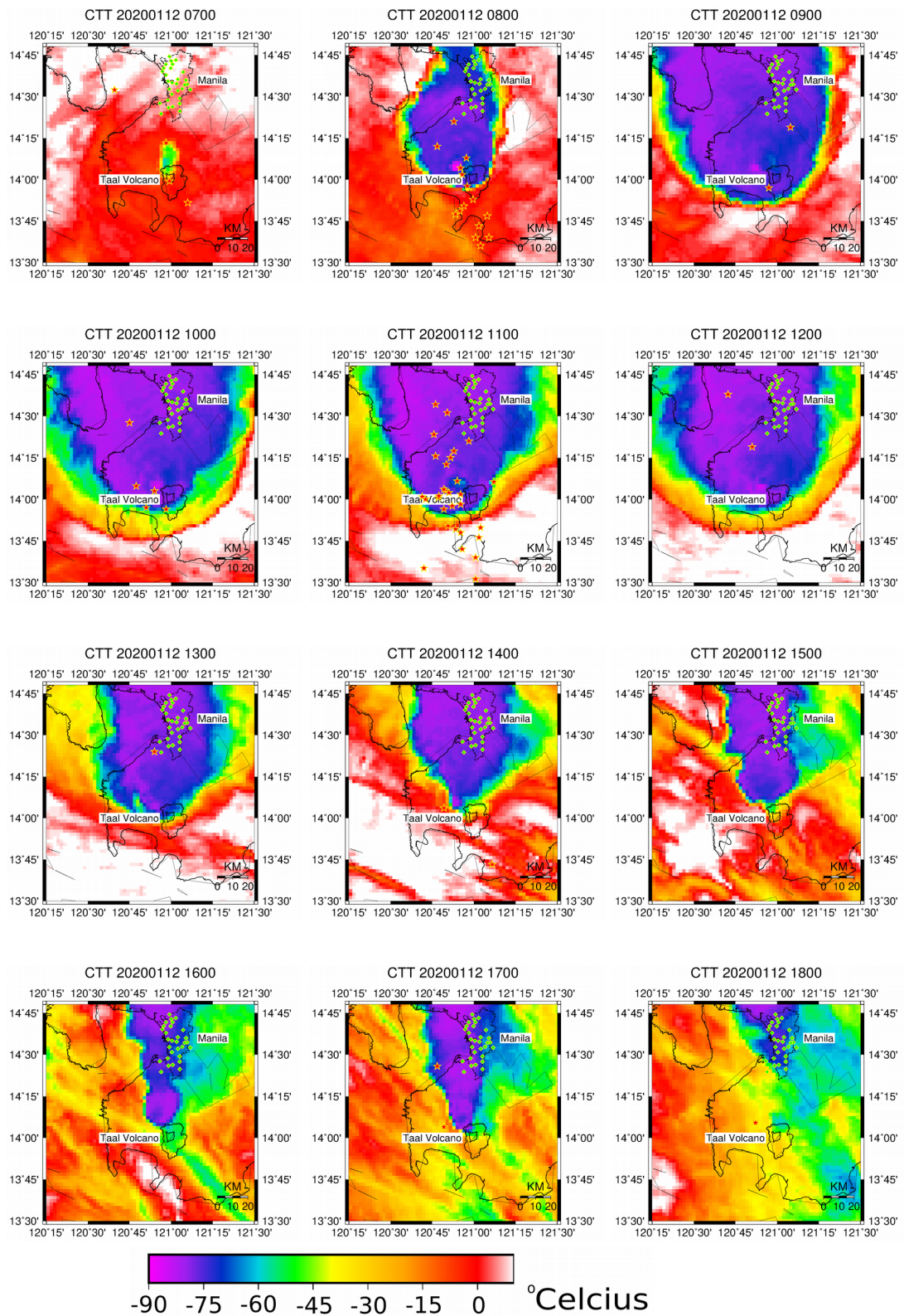
Figure 2.44. Taal volcano eruption detection from space by Himawari 8 Band 15 (12 \mu m) And the lightning detected by V-POTEKA network (red star). Green diamond is the P-POTEKA location in Metro Manila.
