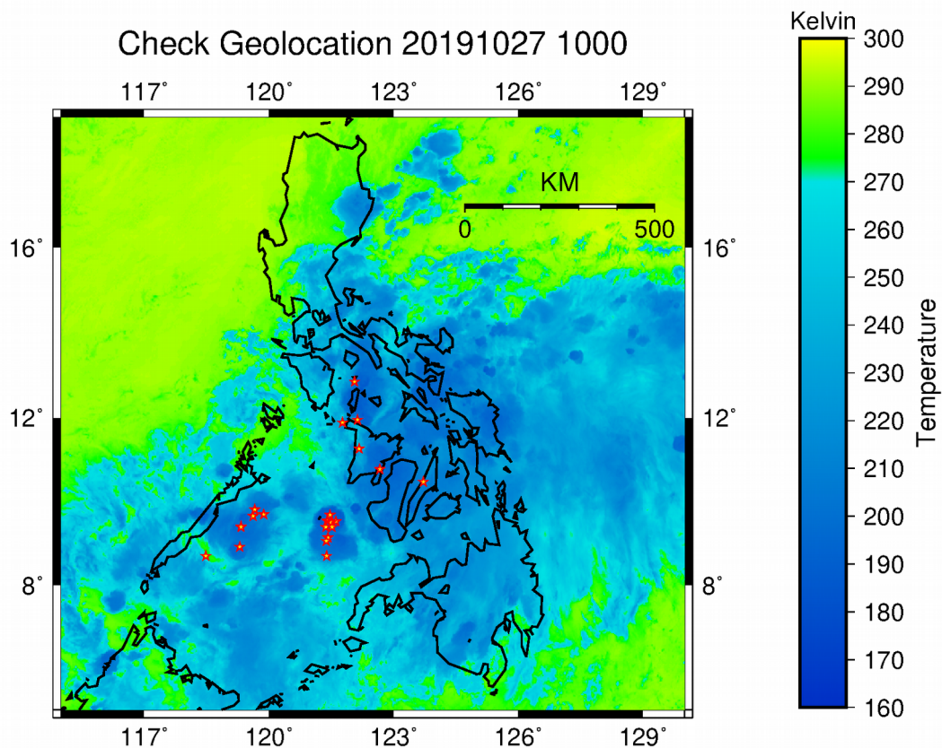
Figure 2.23. Example lightning geo-location result for 10 minutes duration and overlay with Himawari 8 band 15 ( 12.4\ \mu\text{m} )
