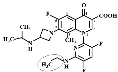
Figure 15. Chemical structures of fluoroquinolones used in the present study.
