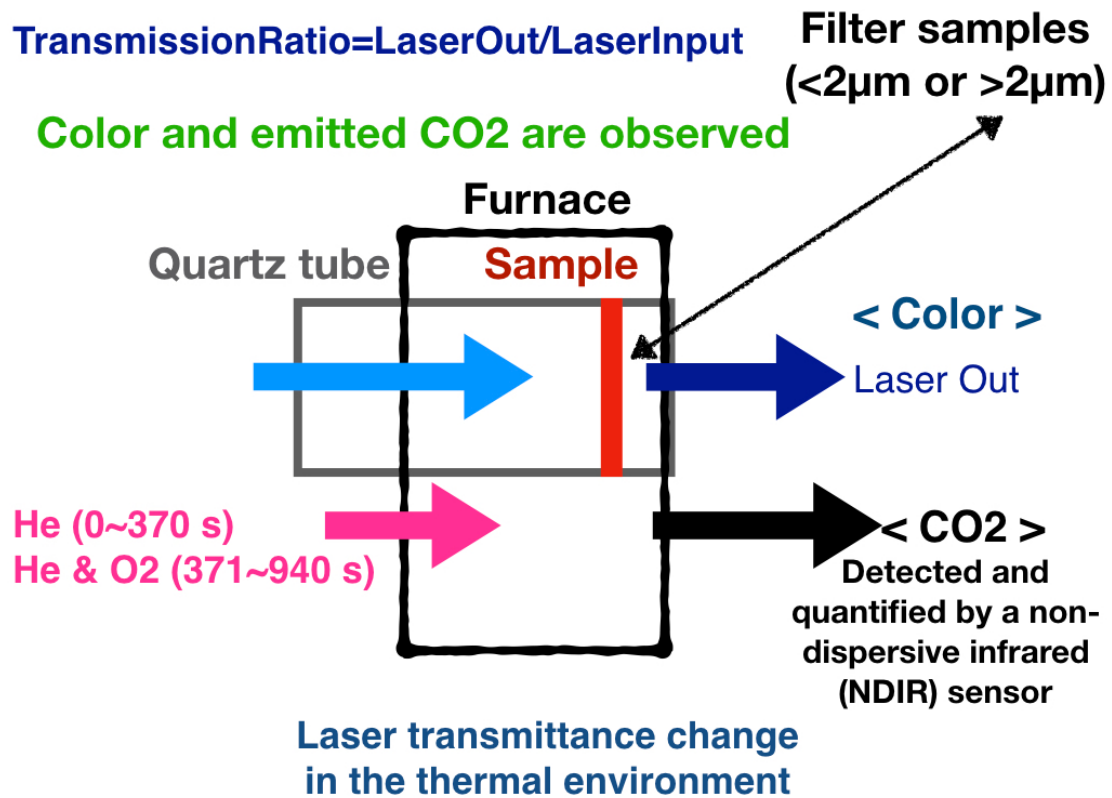
Figure 10. The device schematic of thermal optical transmittance (TOT).
