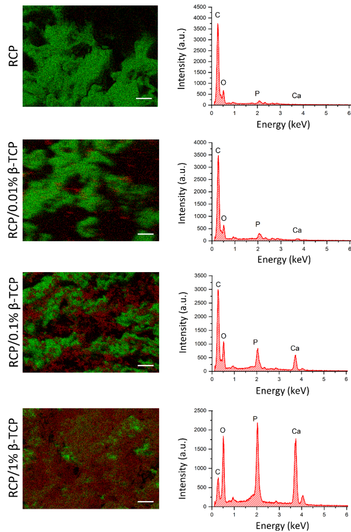
Figure 2. EDX analysis
