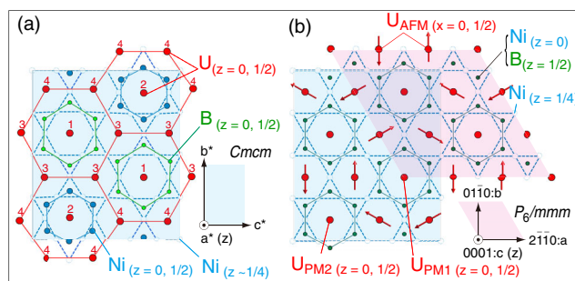
FIG. 1. Crystal and magnetic structure of \text{UNi}_4\text{B} , reported for B = 0 [16,18]. (a) The pseudo-honeycomb network consists of two-thirds of U ions with Cmcm lattice. Red, blue, and green circles indicate U and Ni or B on the layer at z = 0, 1/2 , respectively. Dashed lines with open circles show the (pseudo) Kagome layer of Ni atoms at z \sim 1/4 . (b) Colored backgrounds with pink-rhomboidal and blue-rectangular shapes denote antiferromagnetic unit cells in hexagonal ( P6/mmm ) and orthorhombic ( Cmcm ) symmetry, respectively.
