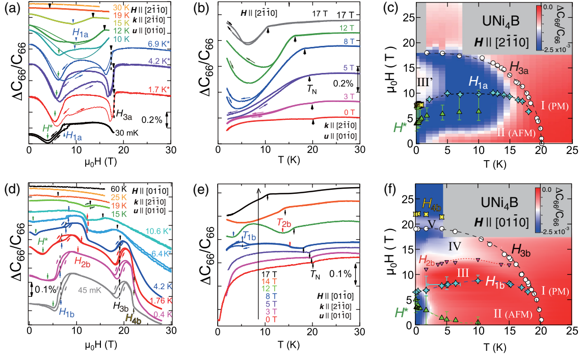
FIG. 4. Magnetic-field dependence of C_{66} for (a) H \parallel [2\bar{1}\bar{1}0] and (d) H \parallel [0\bar{1}\bar{1}0] of \text{UNi}_4\text{B} at selected temperatures. C_{66} vs temperature under various magnetic fields for (b) H \parallel [2\bar{1}\bar{1}0] and (e) H \parallel [0\bar{1}\bar{1}0] . In each panel, vertical arrows indicate elastic anomalies, which correspond to phase boundaries in the magnetic field-temperature phase diagram of \text{UNi}_4\text{B} for (c) H \parallel [2\bar{1}\bar{1}0] and (f) H \parallel [0\bar{1}\bar{1}0] . Dotted and dashed lines are guides for the eyes. The relative change of the elastic constant C_{66} is highlighted by the color map from zero (red) to large negative (blue) values.
