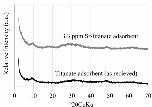
Figure 2. XRD patterns of titanate adsorbent before and after loading with \text{Sr}^{2+}
