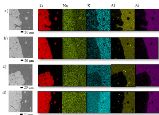
Figure 5. SEM images and elemental maps of specimens with titanate adsorbent; a) before, and after b) 19days, c) 90days, and d) 360 days of leaching in deionized water
