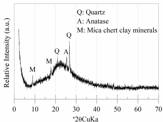
Figure 1. XRD pattern of the metakaolin precursor
