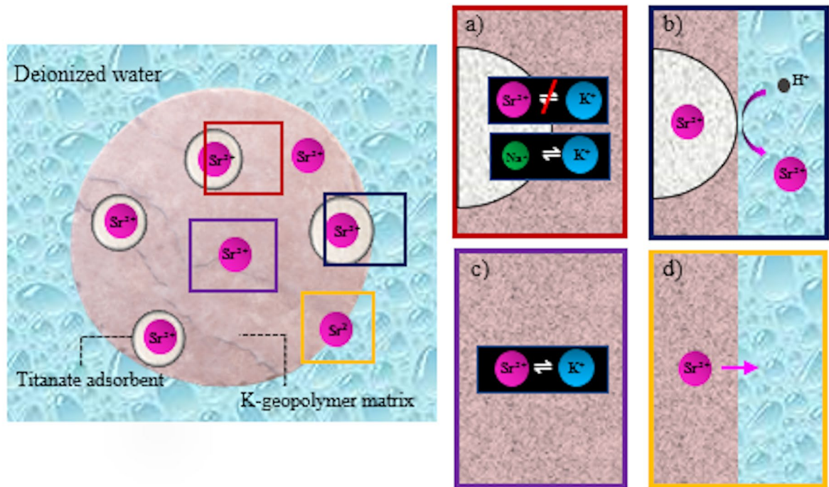
Figure 8. Schematic diagram of geopolymer matrix encapsulated titanate adsorbent adsorbed strontium, the interaction where a) between titanate adsorbent and geopolymer matrix inside specimen, b) the edge between titanate adsorbent and deionized water, c) geopolymer binder area, d) the edge between geopolymer matrix and deionized water.
