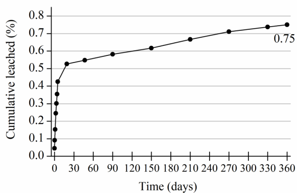
Figure 3. Cumulative leaching of \text{Sr}^{2+} from geopolymer mixed with titanate adsorbent, applying the ANSI/ANS 16.1 test method with full replacement of leachate at each sampling
