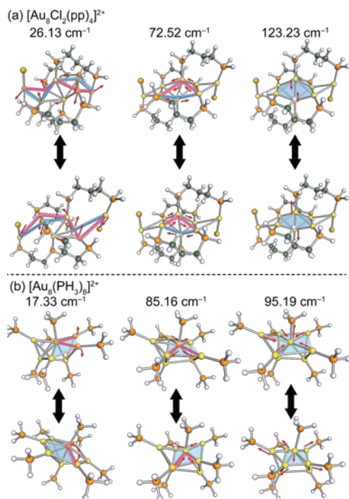
Figure 3. (a) Representative vibrational modes of 1' at 26.13 \text{cm}^{-1} for \delta(\text{Au}_{\text{exo}}-\text{Au}_{\text{edge}}-\text{Au}_{\text{center}}) and \nu(\text{Au}_{\text{edge}}-\text{Au}_{\text{exo}}) , 72.52 \text{cm}^{-1} for \nu_{\text{as}}(\text{Au}_{\text{edge}}-\text{Au}_{\text{center}}-\text{Au}_{\text{edge}}) , and 123.23 \text{cm}^{-1} for the \text{Au}_6 core breathing. (b) Representative vibrational modes of 2' at 17.33 \text{cm}^{-1} for \delta(\text{Au}_{\text{seat-f}}-\text{Au}_{\text{center}}-\text{Au}_{\text{seat-f}}) , 85.16 \text{cm}^{-1} with \nu_{\text{as}}(\text{Au}_{\text{seat-b}}-\text{Au}_{\text{center}}-\text{Au}_{\text{seat-f}}) and 95.19 \text{cm}^{-1} for the seat expanding mode. Seat planes are also shown in blue for 2' . Au, P, C, H and Cl atoms are in yellow, orange, green, white and brown, respectively. Movies showing these vibrational modes are available in the SI.
