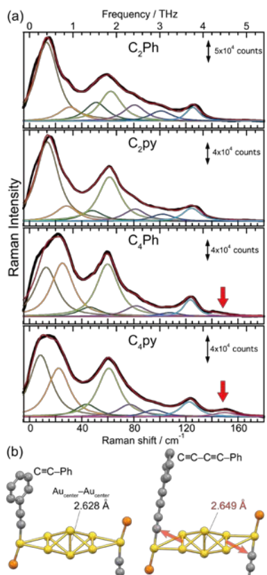
Figure 4. (a) THz Raman spectra of mono- and di-acetylenic \text{Au}_8 clusters of [\text{Au}_8\text{X}_2(\text{dppp})_4](\text{NO}_3)_2 ( \text{X} = \text{C}_2\text{Ph}, \text{C}_2\text{py}, \text{C}_4\text{Ph}, \text{C}_4\text{py} ) with deconvoluted peaks. Excitation wavelength: 785 nm; power input: \sim 1 mW. Arrows in red indicate the characteristic peak for the di-acetylenic \text{Au}_8 clusters. (b) Schematic representation of the \text{Au}_8 framework of the \text{C}_2\text{Ph} and \text{C}_4\text{Ph} complexes with \text{Au}_{\text{center}}\text{--Au}_{\text{center}} bond lengths. 13,36 The red arrows indicate \text{Au}\cdots\pi interactions between the \text{C}_\alpha atom of \text{C}_4\text{Ph} and the \text{Au}_{\text{edge}} atom.
