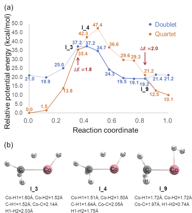
FIG. 7. (a) Reaction pathway of CoH + catalyzed methane activation (two images, I 3 and I 9 , were optimized as MEISC points, and one image, I 4 , was optimized as TS). (b) Geometric information of important images. The definition of reaction coordinate can be found in the supplementary material .
