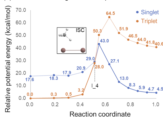
FIG. 4. (a) Relative potential energy profile of \text{In}_2 -catalyzed C–H bond activation with nine intermediate images (No image was optimized as the MEISC point). (b) The relative potential energy profile of \text{In}_2 -catalyzed C–H bond activation with ten intermediate images (one image was optimized as the MEISC point). The definition of the reaction coordinate can be found in the supplementary material .
