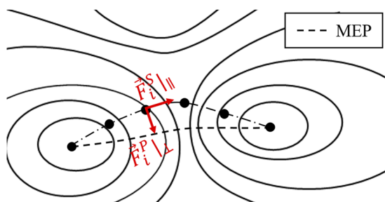
FIG. 1. Schematic illustration of the forces and the relation to MEP. Image i is driven to a point on the MEP under forces \vec{F}_i^P and \vec{F}_i^S in Eq. (3). After all the images are converged together, they compose MEP.
