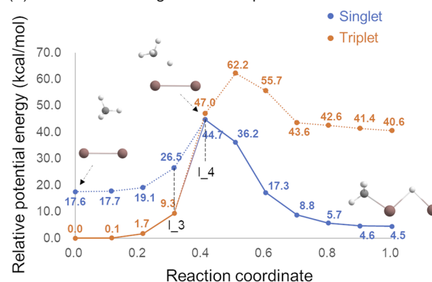
(a) Intermediate image number equals to 9
