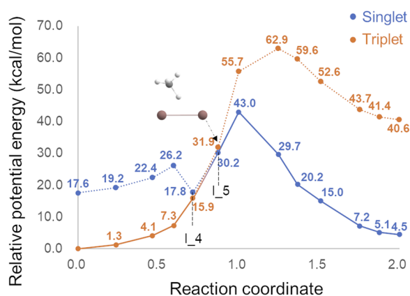
FIG. 5. The result of stepwise MS-NEB. Image 5 was optimized as the MEISC. The definition of the reaction coordinate can be found in the supplementary material .
