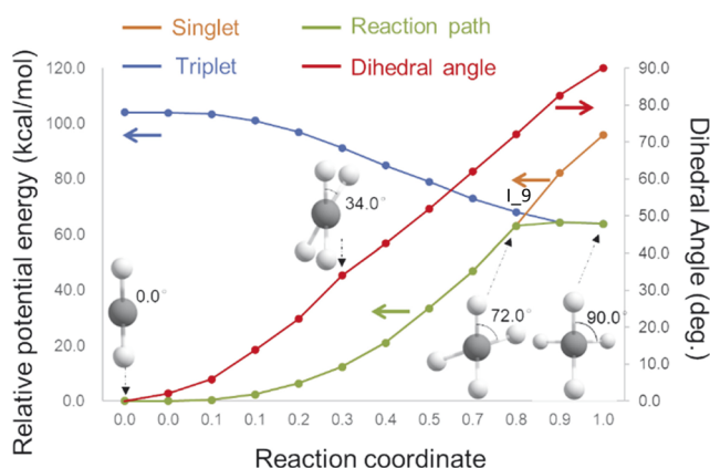
FIG. 3. Relative potential energy curves of ethylene C–C double bond rotation obtained by the MS-NEB method. Orange and blue lines are for singlet and triplet states, respectively. The green line represents the reaction pathway (singlet state from image 0 to image 10 and the triplet state from image 11 to image 12). The H–C–C–H dihedral angle of each image is represented by the red line. The definition of the reaction coordinate can be found in the supplementary material .
