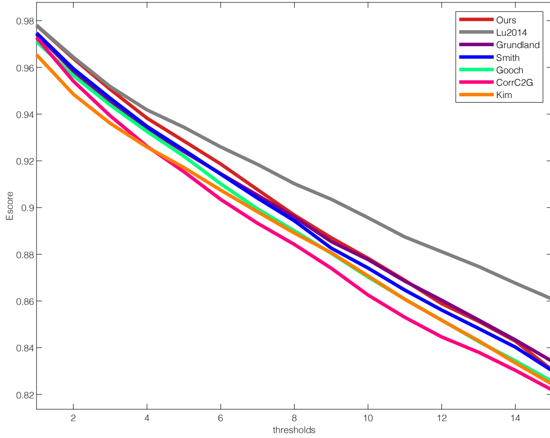
Fig 9 Comparison of seven color to gray methods based on the E-score.
