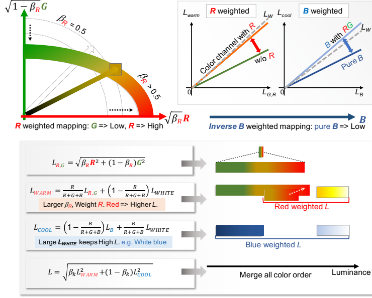
Fig 3 Remodeling of luminance space based on our two weighting functions one each for warm and cool colors. Here, luminance is defined as the Euclidean distance of warm/cool color. The included color panels aid in intuitive understanding of the proposed method.
