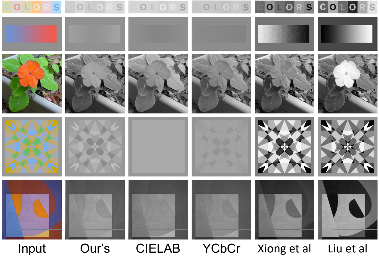
Fig 16 Color to gray conversion comparison using five images from Cadik's dataset. 27 Decolorization methods: Ours, CIELAB, YCbCr, Xiong et al., 34 and Liu et al. 35
