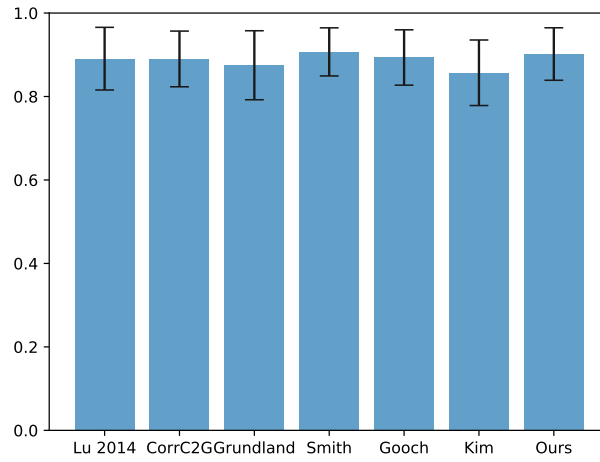
Fig 10 Comparison of seven color to gray methods based on the C2G-SSIM score.
