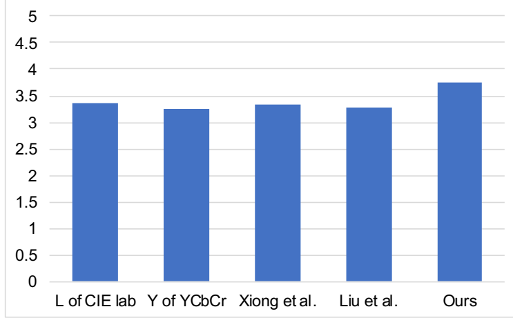
Fig 15 Mean opinion score from the tone mapping subjective user study.
