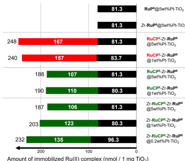
Figure 1. Estimated amounts of the Ru(II) PS (red: \text{RuCP}^2 , black: \text{RuP}^6 , and green: \text{RuCP}^6 ) immobilized on the Pt-TiO 2 nanoparticle surface determined by UV-Vis absorption spectra of the supernatant solutions obtained from the immobilization experiments. Numerical values in each bar show the immobilized amount of Ru(II) PS (nmol / 1 mg \text{TiO}_2 ). The total amount of Ru(II) PSs of double-PS-layered nanoparticle is given on the left side of each bar.
