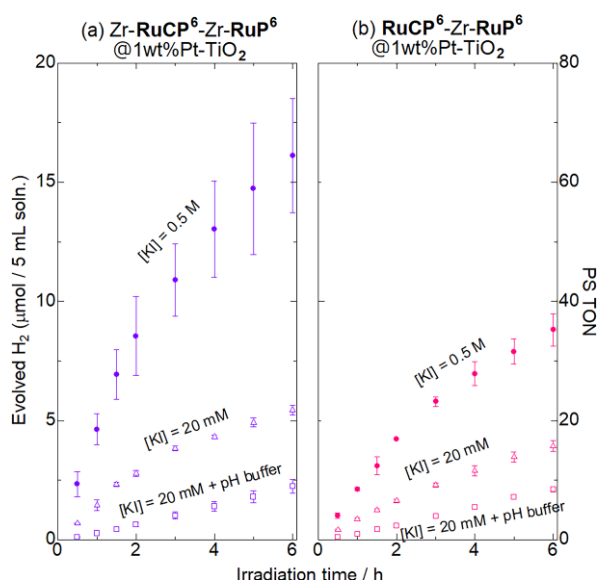
Figure 4. The effects of initial KI concentration and phosphate buffer on the photocatalytic H 2 evolution reaction driven by (a) Zr-RuCP 6 -Zr-RuP 6 @1 wt%Pt-TiO 2 and (b) RuCP 6 -Zr-RuP 6 @1 wt%Pt-TiO 2 (100 μM Ru(II) dye). Closed circles show the results in 0.5 M KI without pH buffer (the initial pH = 2.0, the same data shown in Figures 3(a) and 3(b)), and open triangles and squares are the results obtained in the 0.02 M KI without and with phosphate pH buffer, respectively (pH = 2.0, λ = 470 ± 10 nm).
