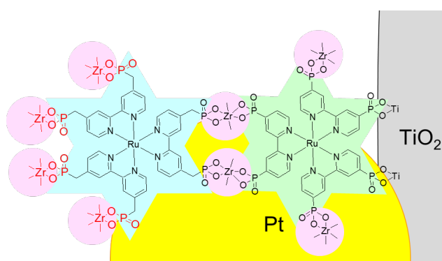
Scheme 1. Schematic structure of double-PS-layer nanoparticle photocatalyst \text{Zr-RuCP}^6\text{-Zr-RuP}^6\text{@Pt-TiO}_2 .
