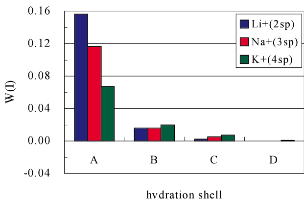
図6. イオンの最外殻軌道の水和の各層ととの間の average overlap population
