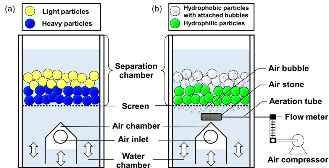
Fig. 1 A schematic illustration of (a) RETAC jig, and (b) Hybrid jig.
