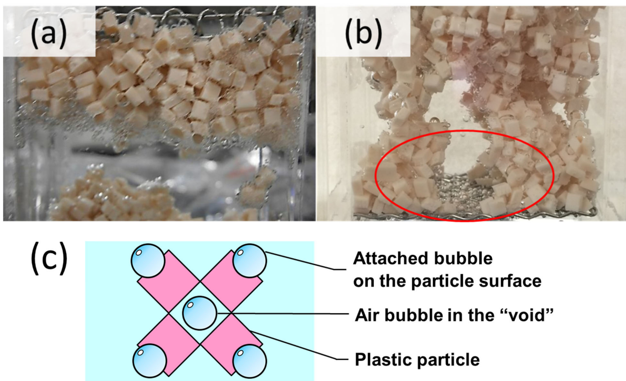
Fig. 7 Photographs of (a) bubbles in the “void” and (b) bubbles attached on the bottom screen, and (c) a schematic diagram of air bubble in the void and on the particle surface.
