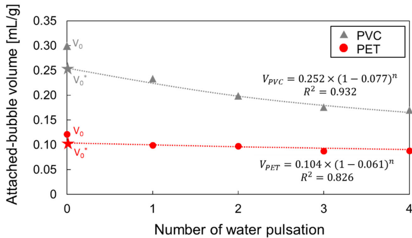
Fig. 6 Attached-bubble volume on PVC and PET as a function of water pulsation without air introduction.
