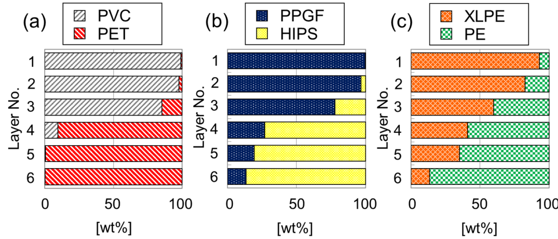
Fig. 5 The proportion of plastics in each layer after hybrid jig separation of (a) PVC/PET with 50 ppm of NaLS, (b) PPGF/HIPS with 350 ppm of TA, and (c) XLPE/PE with 50 ppm of TA.
