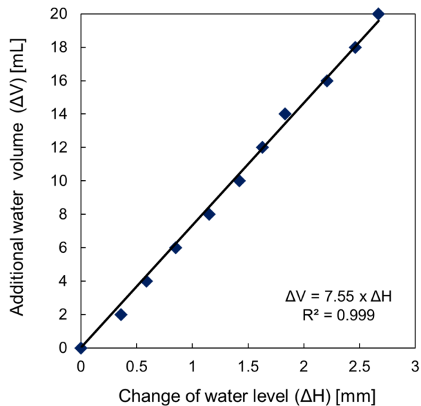
Fig. 3 Relationship between volume increase and water level rise in water chamber after bubble introduction.
