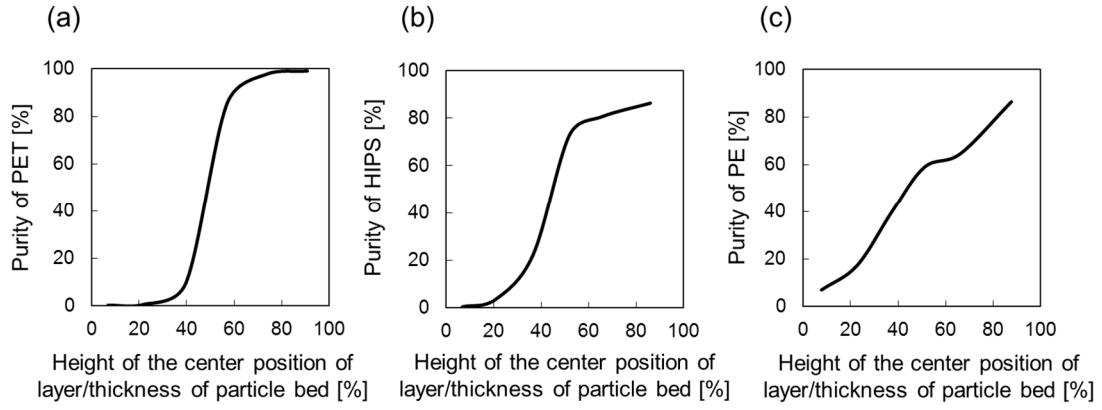
Fig. 9 Purity distribution curves as a function of height of hybrid jig separation of (a) PVC/PET with 50 ppm of NaLS, (b) PPGF/HIPS with 350 ppm of TA, and (c) XLPE/PE with 50 ppm of TA.
