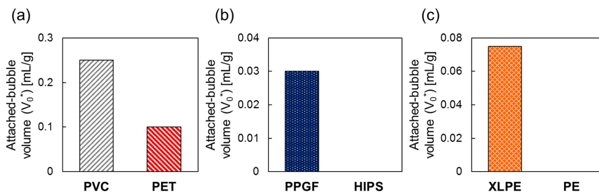
Fig. 8 Estimated volume of attached bubble on (a) PVC/PET in NaLS 50 ppm solution, (b) PPGF/HIPS in TA 100 ppm solution, and (c) XLPE/PE in TA 50 ppm solution.
