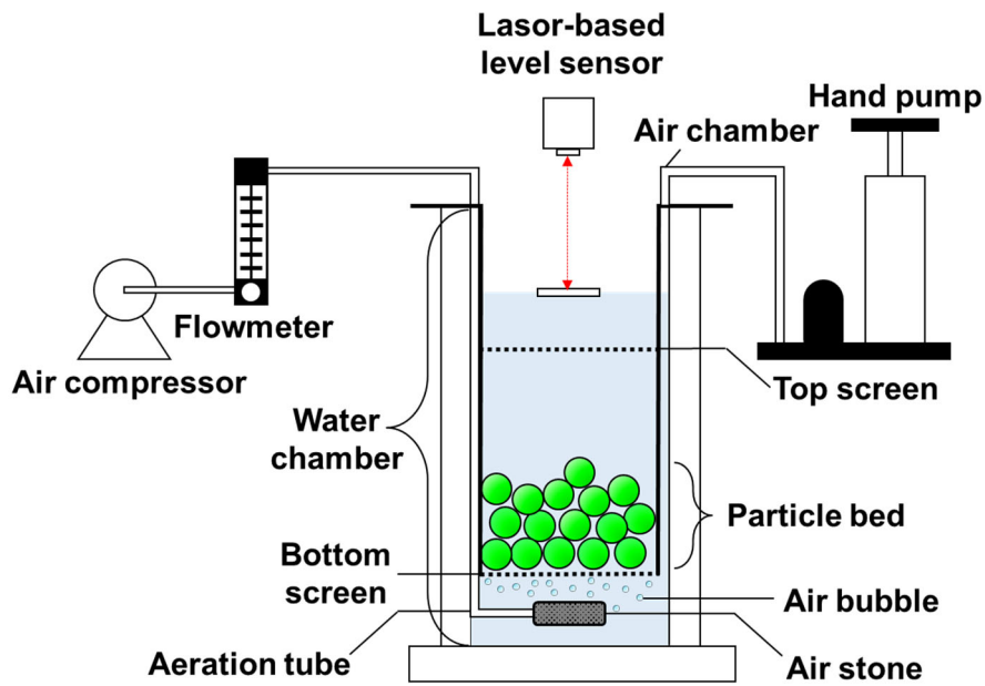
Fig. 2 A schematic diagram of the laser-assisted measurement setup for the determination of attached-bubble volume.
