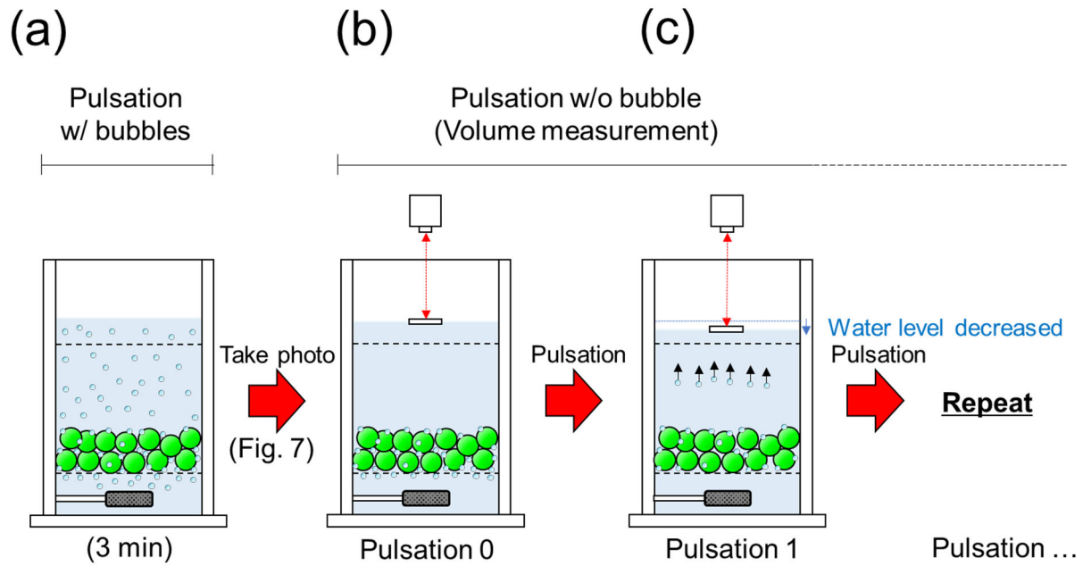
Fig. 4 A schematic diagram of attached-bubble volume measurement procedure; (a) water pulsation with bubble generation for 3 min, (b) measurement of water level after step (a), and (c) measurement of water level after one pulsation of water without bubble generation to remove trapped bubbles in voids with in particle bed.
