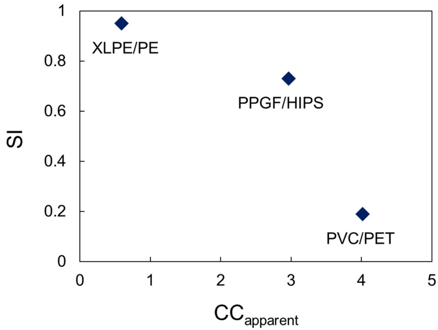
Fig. 10 Relationship between sharpness index (SI) and concentration criterion using apparent specific gravity (CC apparent ).
