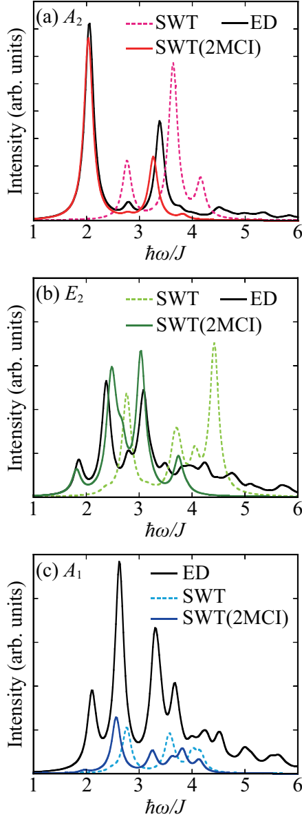
Figure 5 The fourth-order magnetic Raman spectra on the N = 16 sites cluster for (a) A_2 mode, (b) E_2 mode, and (c) A_1 mode. Spectra are calculated by Lancz s exact diagonalization (ED), spin-wave theory without magnon-magnon interactions (SWT), and spin-wave theory with magnon-magnon interactions introduced by two-magnon excitation CI method [SWT(2MCI)].
