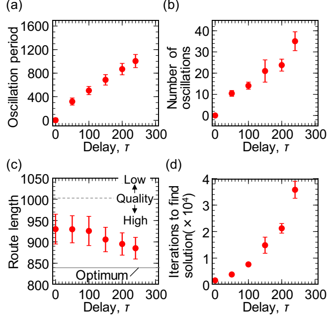
Fig. 3: Solution search performance as a function of the length of delay evaluated by solving 10-city TSP instance. The average number of (a) periods and (b) oscillations. (c) Solution quality. Solid line indicates the optimal route length and broken line indicates an average length of possible routes obtained from the random sampling algorithm after 10,000 trials. (d) The number of iterations to find a solution. Error bars are the standard deviation derived by 100 trials for each delay length.
