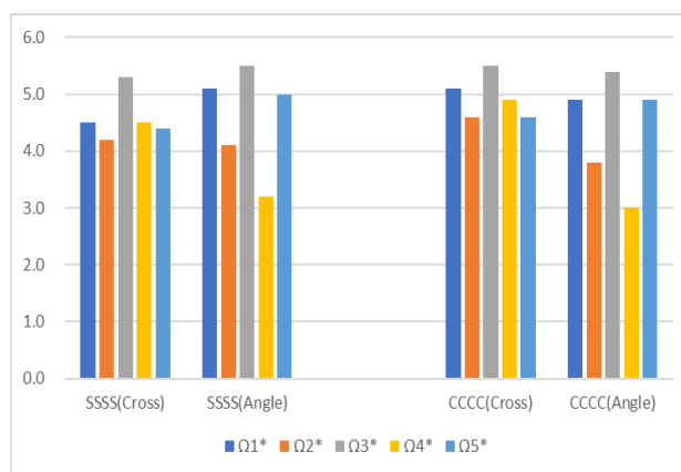
Figure 2. Comparison of percentage differences between cross-ply and angle-ply square plates with SSSS and CCCC boundary conditions (Mat.4)
