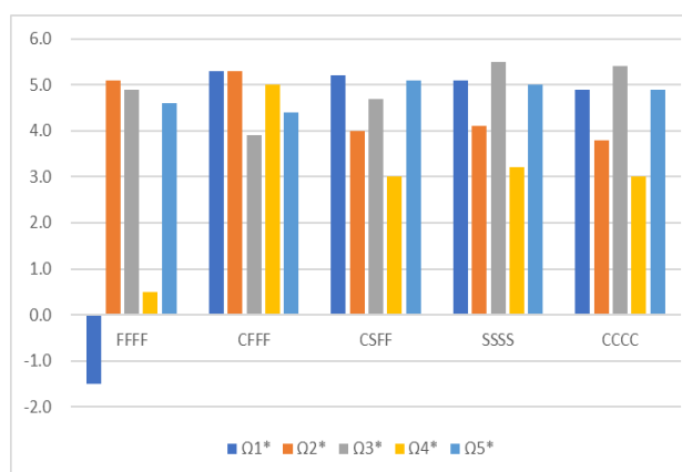
Figure 3. Comparison of percentage differences in angle-ply square plates among five sets of boundary conditions (Mat.4)
