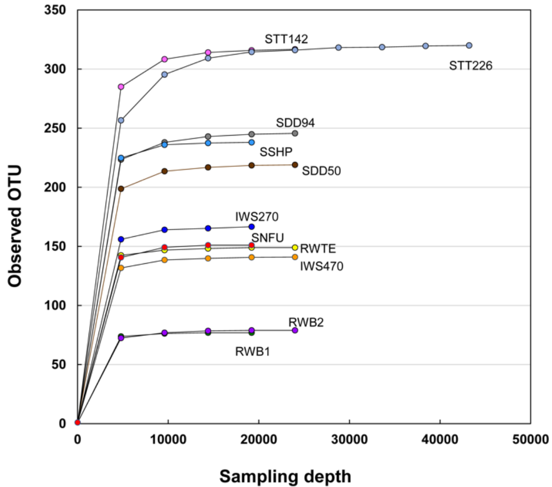
Figure 6 Rarefaction curve of operational taxonomic units (OTUs) defined by 3% sequence variation in 16S rRNA sequencing reads in samples from the indigo fermentation system. STT142, 226: sukumo (produced in Tokushima by TT) fermentation prepared in the laboratory, aged 142 and 226 d; SDD50, 94: sukumo (produced in Date, Hokkaido by KS) fermentation prepared in the laboratory, aged 50 and 94 d; SNFU: sukumo (produced in Tokushima by ON) fermentation; SSHP: sukumo (main constituent was produced in Tokushima by AS) fermentation; RWB 1, 2: Ryukyu-ai based fermentation with wheat bran as the nutrient; RWBE: Ryukyu-ai based fermentation with wheat bran and ethanol as nutrients, and tamarind as the additive; IWS270, 470: Indian indigo-based fermentation with wheat bran as the nutrient.
