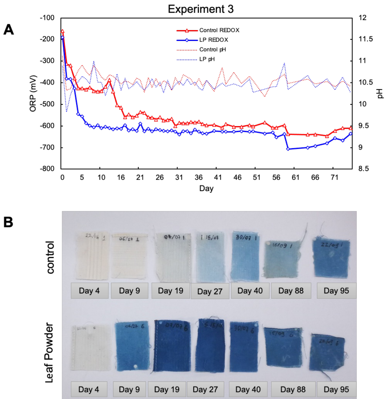
Figure 20 Changes in redox potential (ORP) and pH from day 1 to day 75 (A) and dyeing results from day 4 to day 95 of Experiment 3 with (LP) and without (control) Indigofera tinctoria leaf powder.
