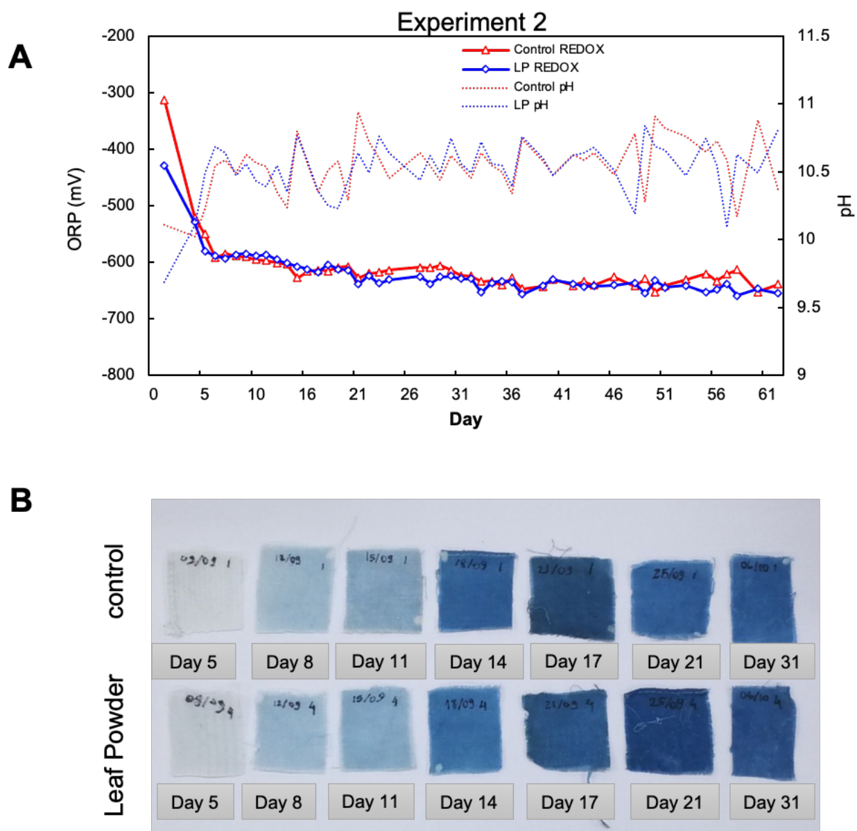
Figure 19 Changes in redox potential (ORP) and pH from day 1 to day 62 (A) and dyeing results from day 5 to day 31 of Experiment 2 with (LP) and without (control) Indigofera tinctoria leaf powder.
