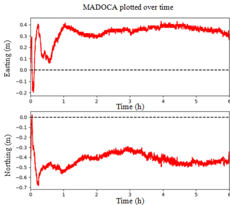
Figure 4.8 Result from the performance evaluation under static conditions of the MADOCA positioning augmentation system plotted in time series.
