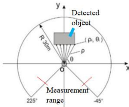
Figure 3.8 Schematic diagram of laser rangefinder.
