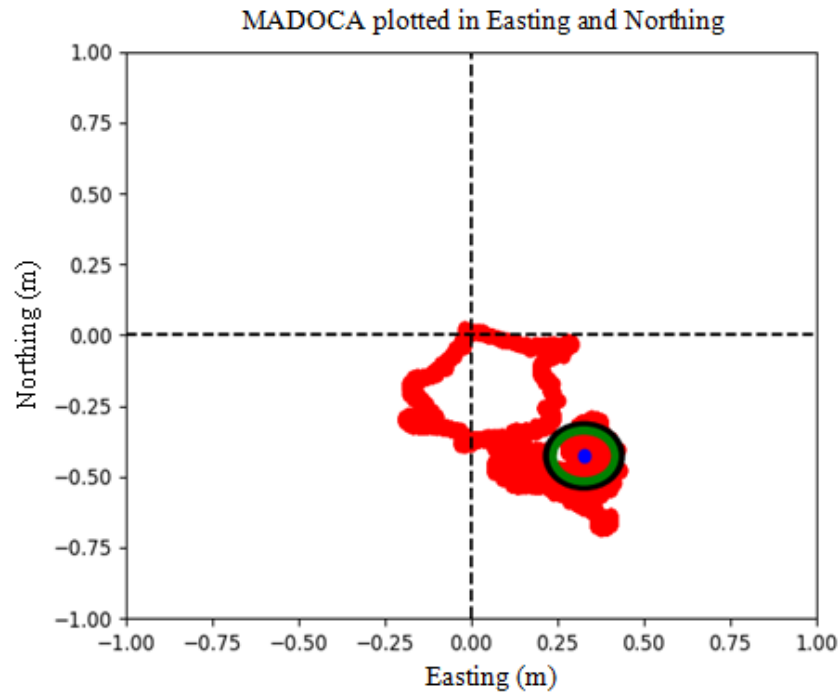
Figure 4.6 Result from the performance evaluation under static conditions of the MADOCA positioning augmentation system plotted in Easting and Northing coordinates.
