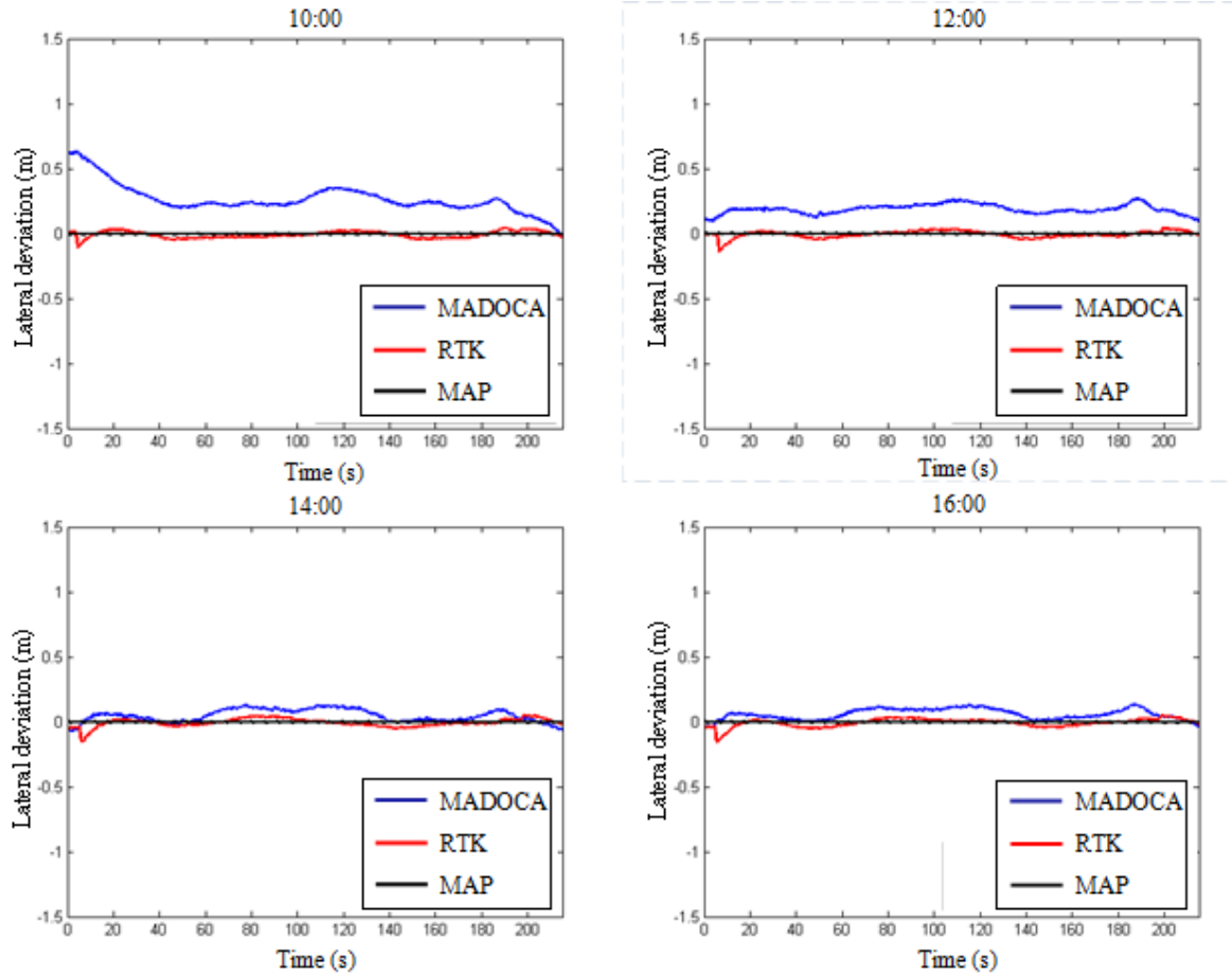
Figure 5.5 Second feasibility test by utilizing the RTK positioning augmentation system as a navigation sensor for the auto-guided combine harvester logged with the MADOCA.
