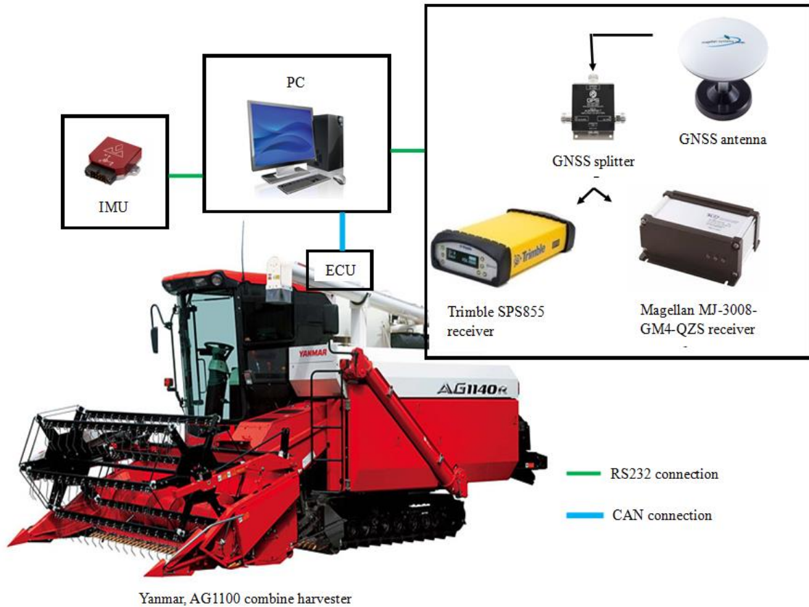
Figure 5.1 The overall setup of three feasibility tests.
