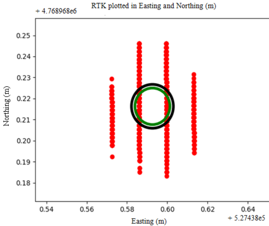
Figure 4.3 Result from the performance evaluation under static conditions of the RTK positioning augmentation system plotted in Easting and Northing coordinates.
