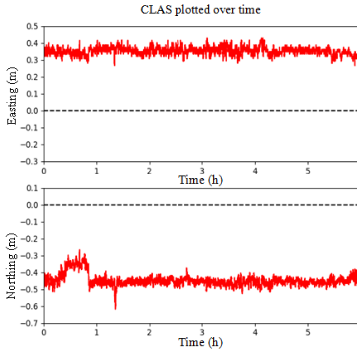
Figure 4.7 Result from the performance evaluation under static conditions of the CLAS positioning augmentation system plotted in time series.
