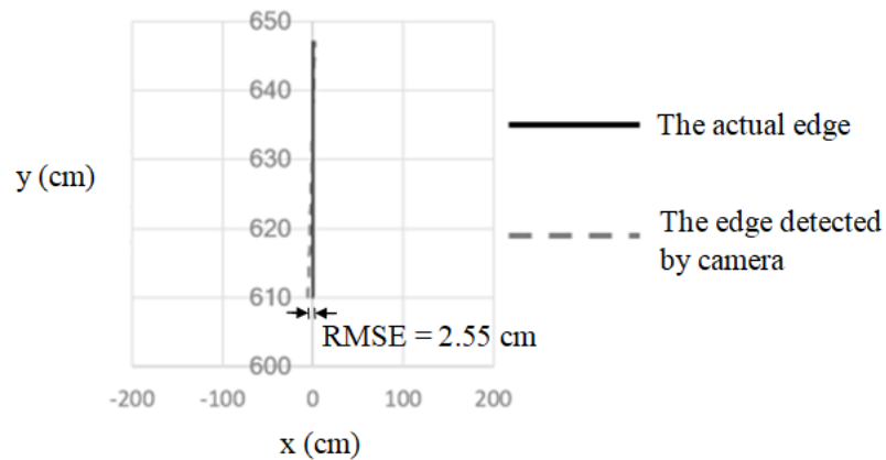
Figure 3.10 The actual edge of card boxes and the edge detected by RGB camera.
