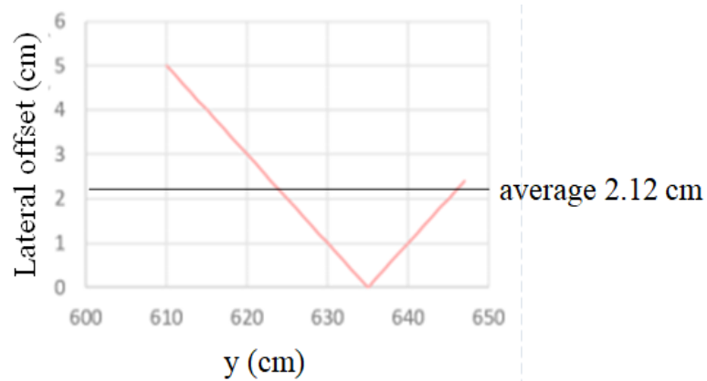
Figure 3.11 The lateral offset of edge detection by using an RGB camera.
