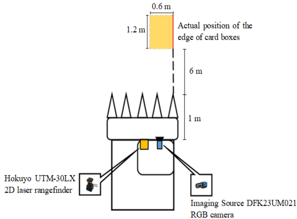
Figure 3.2 Diagram of simulation experiment.
