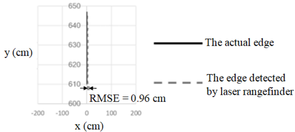
Figure 3.12 The actual edge of card boxes and the edge detected by laser rangefinder.
