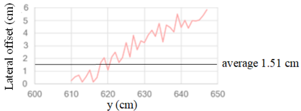
Figure 3.15 The lateral offset of edge detection by using sensor fusion.
