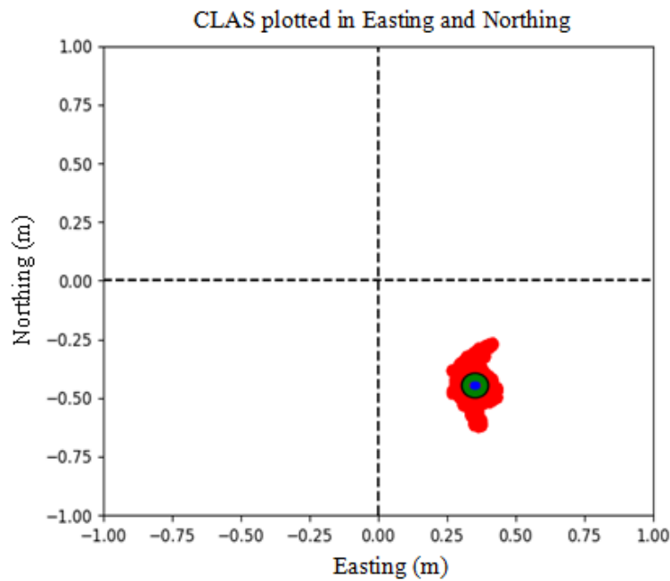
Figure 4.5 Result from the performance evaluation under static conditions of the CLAS positioning augmentation system plotted in Easting and Northing coordinates.
