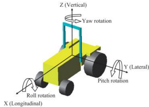
Figure 2.6 Definition of the roll, pitch, and yaw angle.
