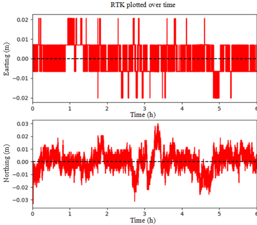
Figure 4.4 Result from the performance evaluation under static conditions of the RTK positioning augmentation system plotted in time series.
