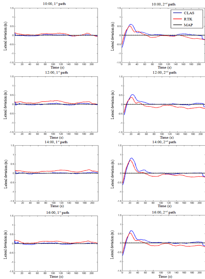
Figure 5.6 Third feasibility test by utilizing the CLAS positioning augmentation system as a navigation sensor for the auto-guided combine harvester logged with the RTK.
