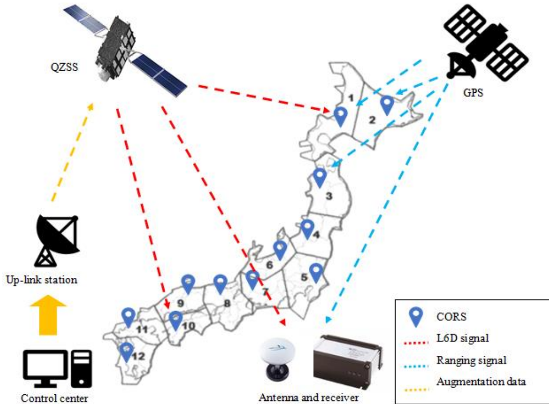
Figure 2.10 Diagram of the CLAS positioning augmentation system.
