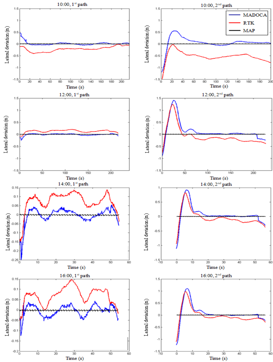
Figure 5.7 Third feasibility test by utilizing the MADOCA positioning augmentation system as a navigation sensor for the auto-guided combine harvester logged with the RTK.
