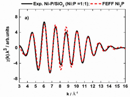
Figure 6. Comparison between theoretical \text{Ni}_2\text{P} (red broken line) and experimental EXAFS spectra of \text{Ni-P/SiO}_2 ( \text{Ni:P} = 1:1 ) (black line).
