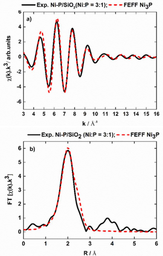
Figure 10. a) Comparison between theoretical Ni 3 P (red broken line) and experimental (black line) EXAFS spectra of Ni-P/SiO 2 (Ni:P = 3:1) (black line); b) corresponding Fourier transforms.
