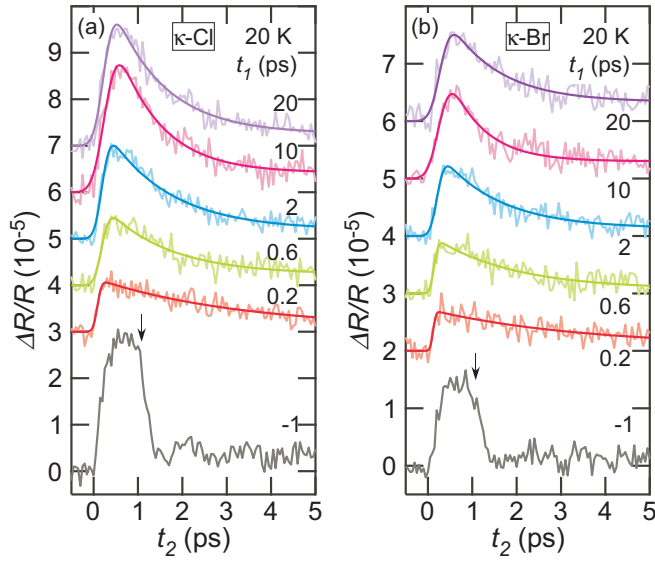
FIG. 2. Transient change in reflectivity \Delta R/R as a function of t_2 at T = 20 K for t_1 = 0.2, 0.6, 2 and 10 and 20 ps in (a) \kappa -Cl and (b) \kappa -Br. The measurements were performed with fluence of the P pulse of F = 231 \mu\text{J}/\text{cm}^2 . The solid lines are the result fitted by Eq. (2). The data are shifted for clarity. The arrows denote arrival of the P pulse.
