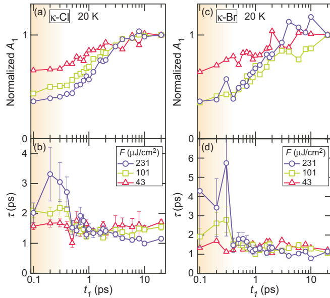
FIG. 4. (a) Normalized A_1 and (b) decay time \tau as a function of t_1 at T = 20 K for F = 43, 101 , and 231 \mu\text{J}/\text{cm}^2 in \kappa\text{-Cl} . (c) Normalized A_1 and (d) decay time \tau as a function of t_1 at T = 20 K for F = 43, 101 , and 231 \mu\text{J}/\text{cm}^2 in \kappa\text{-Br} .
