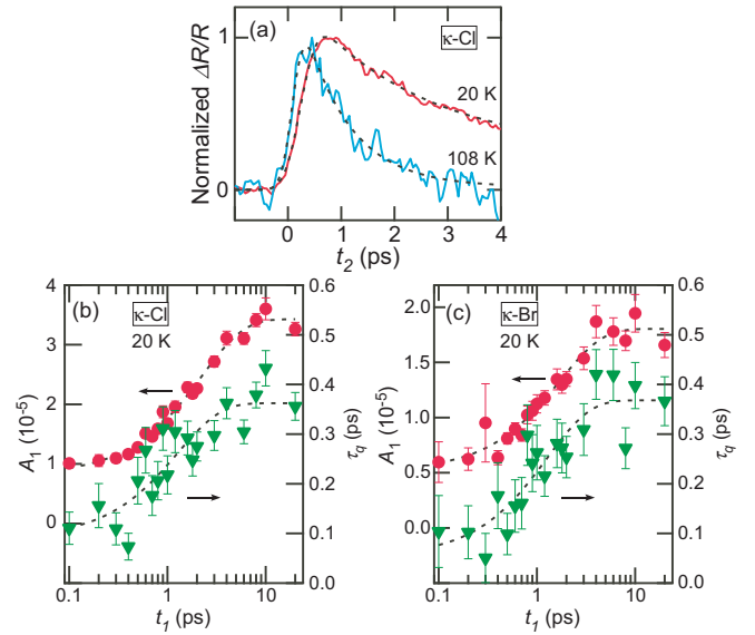
FIG. 5. (a) Comparison of the polarized pump probe reflectivity transients \Delta R/R in \kappa\text{-Cl} at T = 20 K and 108 K. t_1 dependences of A_1 and \tau_q for F = 231 \mu\text{J}/\text{cm}^2 in (b) \kappa\text{-Cl} and (c) \kappa\text{-Br} .
