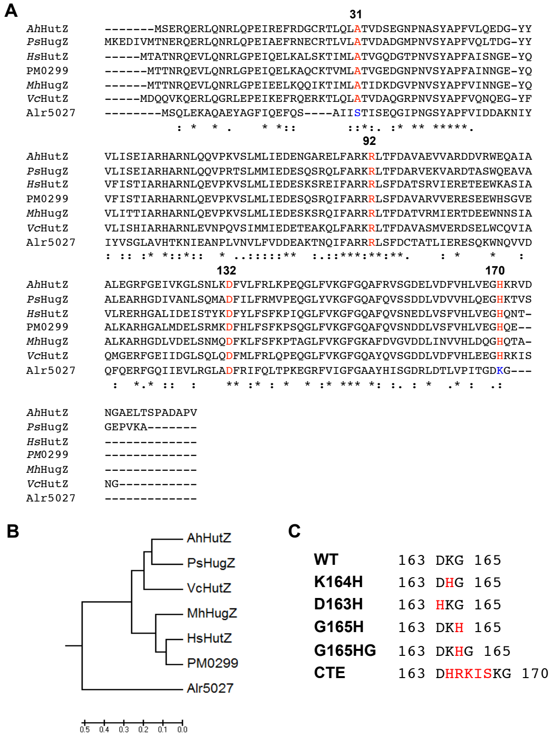
Fig. 1. Sequence alignment of Alr5027. (A) Sequence alignment of the HutZ family and Alr5027. The alignment was performed using ClustalW2 ( http://www.ebi.ac.uk/Tools/msa/clustalw2/ ). The active site arginine, aspartate, and histidine are shown in red bold type. Proteins used in the alignment are (from top to bottom) Aeromonas hydrophila subsp. hydrophila ATCC 7966 HutZ, Plesiomonas shigelloides HugZ, Histophilus somni HutZ, multocida str. Pm70 PM0299, Mannheimia haemolytica PHL213 HugZ, Vibrio cholerae HutZ, and Nostoc sp. PCC 7120 Alr5027. (B) Phylogenetic tree of Alr5027 with the HutZ family. The tree was obtained from the sequence alignment in Fig 1A. The maximum likelihood method was used for tree construction and bootstrap analysis (parameter set at 1000 resampling), performed using MEGA 7 software. (C) Alignment of Alr5027 WT and mutants in the C-terminal region (163–165).
