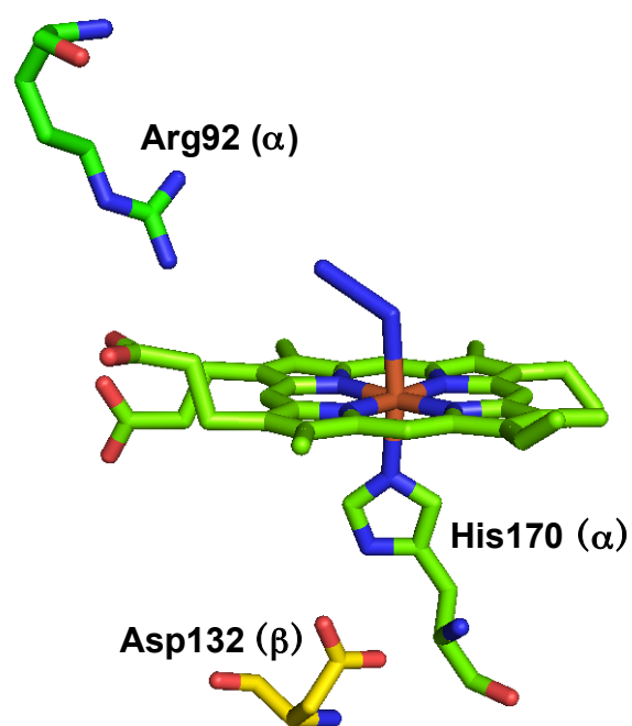
Fig S3. Putative active site of the VcHutZ homologous protein, HugZ, from H. pylori (PDB ID 3GAS). Residue numbering is based on VcHutZ
