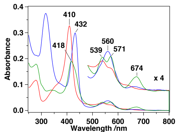
Fig. S8. Absorption spectrum of the heme-K164H mutant. Ferric form (red), ferrous form (blue), reduced by sodium dithionite (0.2 mM), oxyferrous form, produced by air to ferrous form (green). The samples were in 50 mM Tris-HCl and 150 mM NaCl (pH 8.0). Although 1 \mu M catalase was involved in the solution to decompose \text{H}_2\text{O}_2 produced by reduction of contaminated molecular oxygen by dithionite, the spectra of catalase was subtracted from each spectrum.
