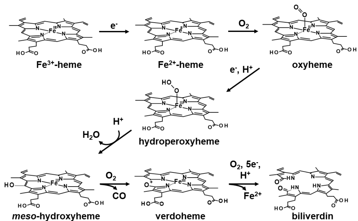
Fig S1. Heme-degradation mechanism of HutZ.
