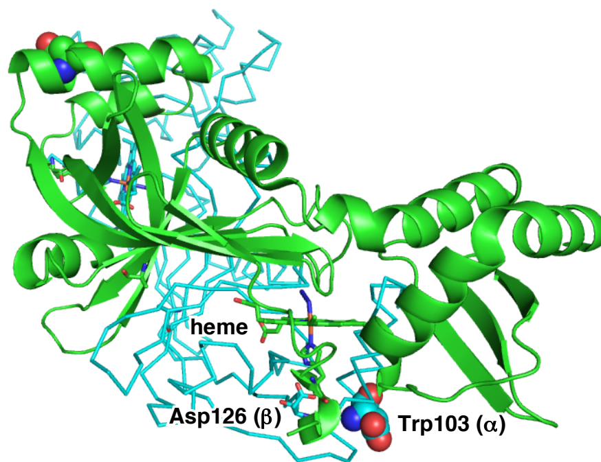
Fig S10. Location of Trp103 and heme on the HugZ crystal structure (PDB 3GAS). Residues are numbered according to the amino acid sequence of Alr5027 from cyanobacteria Nostoc sp. PCC7120. Green and cyan show each protomer. Trp103 is present in a different protomer (green) from that (cyan) containing the nearby Asp126 in a different subunit.
