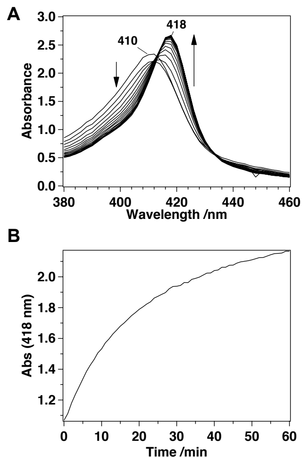
Fig. S7. Determination of the reduction rate of heme. (A) Absorption spectra of heme-K164H after the addition of 1 mM ascorbic acid at pH 8.0 under a CO atmosphere. (B) Time course of absorbance changes at 418 nm.
