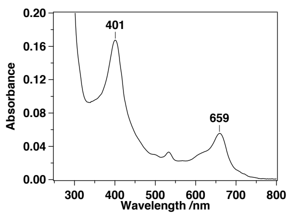
Fig S6. Absorption spectra of verdoheme in aqueous pyridine. (A) K164H and (B) CTE heme-bound mutants were reacted with \text{H}_2\text{O}_2 under the same conditions at those in Figure 5. Pyridine (final concentration, 33%) was added to the reaction mixture 10 min after the reaction to liberate the product from the protein.
