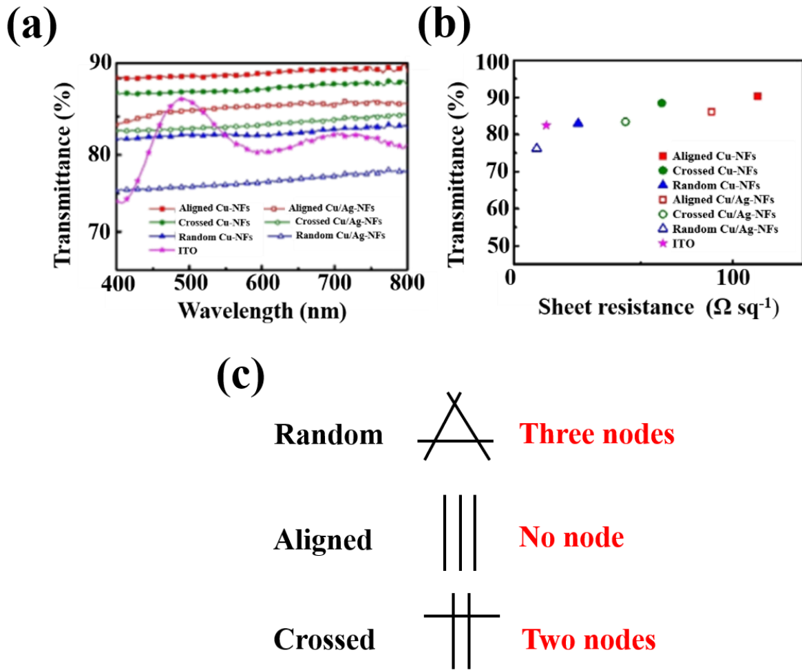
Figure 2.9. (a) Transparency test of Cu-NFs and the Cu/Ag NFs with three architectures (aligned, crossed, random). (b) transmittance ( T ) plotted against sheet resistance ( R_s ) by morphological type (aligned, crossed, and random) of Cu-NFs and Cu/Ag NFs. (c) Nodes theory of transmittance ( T ).
