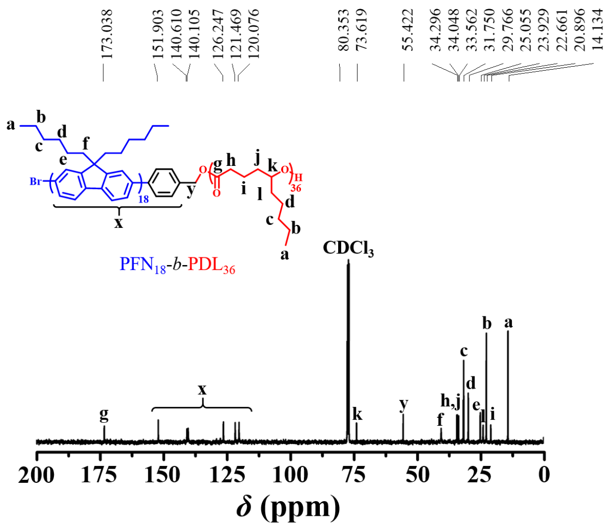
Figure 4.7. The ^{13}\text{C} NMR with peak designation of the polymerization of \text{PFN}_{18}\text{-}b\text{-PDL}_{36} via smart synthesis.
