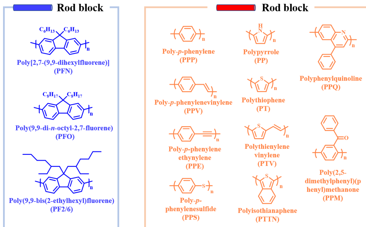
Figure 1.9. The General form from the polymer structures of PF-based conjugated rod-rod block copolymers (BCPs).
