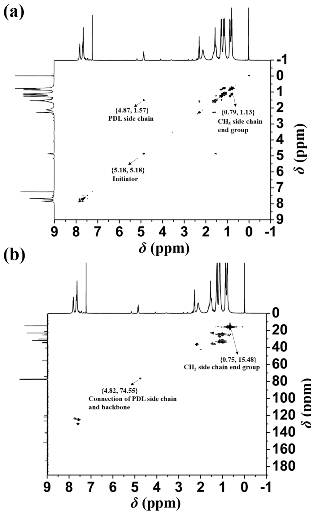
Figure 4.12. The representative ^1\text{H} , ^{13}\text{C} , and 2D NMR spectra of the \text{PFN}_{18}\text{-}b\text{-PDL}_{36} in \text{CDCl}_3 .
