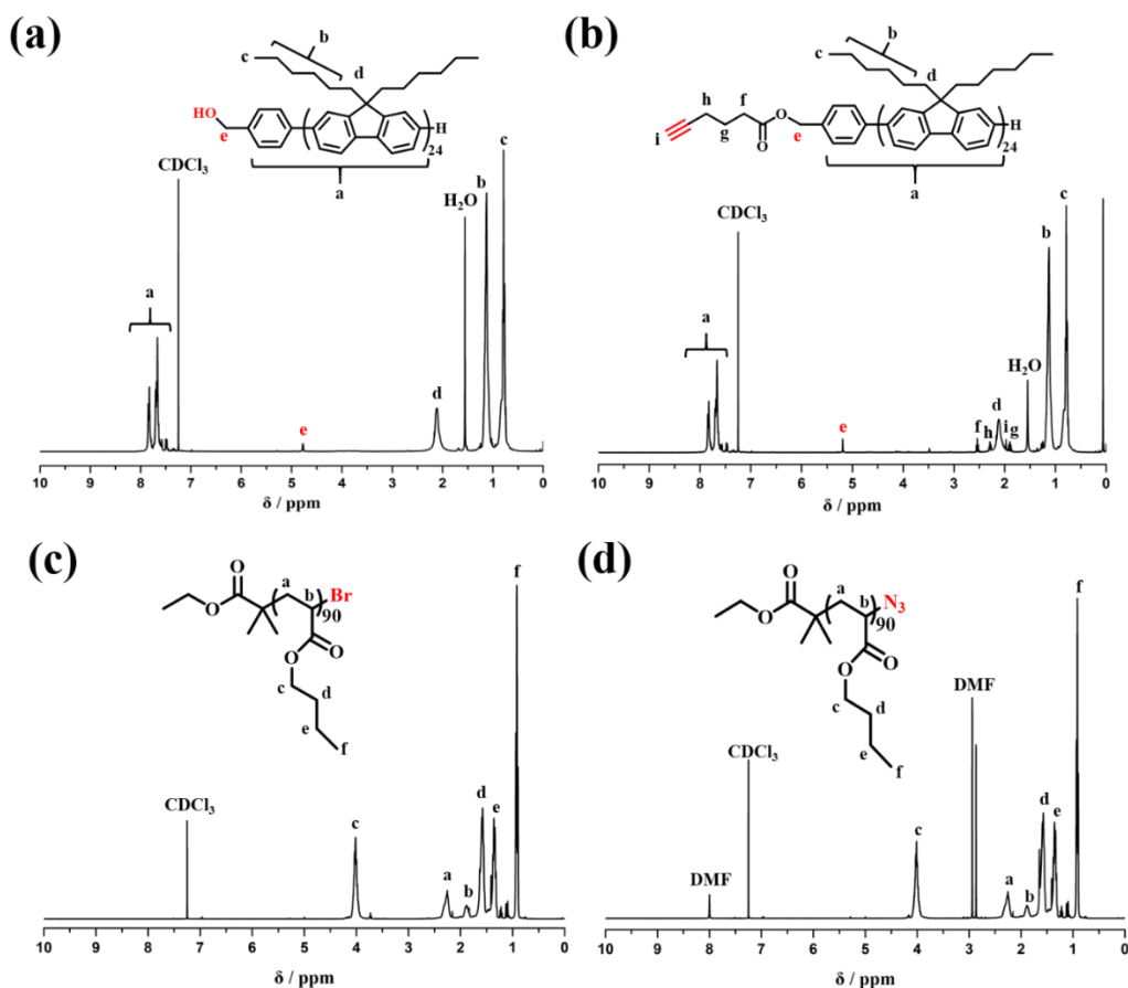
Figure 3.1. ^1\text{H} -NMR spectra of the (a) PFN 24 -BnOH, (b) PFN 24 -C \equiv CH, (c) PBA 90 -Br 3 (d) PBA 90 -N 3 in chloroform- d_1 ( \text{CDCl}_3 ).
