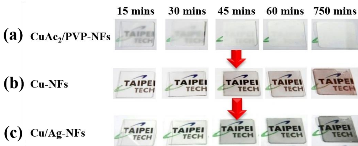
Figure 2.10. Digital photos show the color change of samples (a) \text{CuAc}_2/\text{PVP-NFs} (the precursor samples) (b) \text{Cu-NFs} fabricated by the thermal treatment in the \text{H}_2 atmosphere with 300^\circ\text{C} (red color) and (c) \text{Cu/Ag} core/shell NFs fabricated by the electroless plating process with immersed Ag ink for 15 s.
