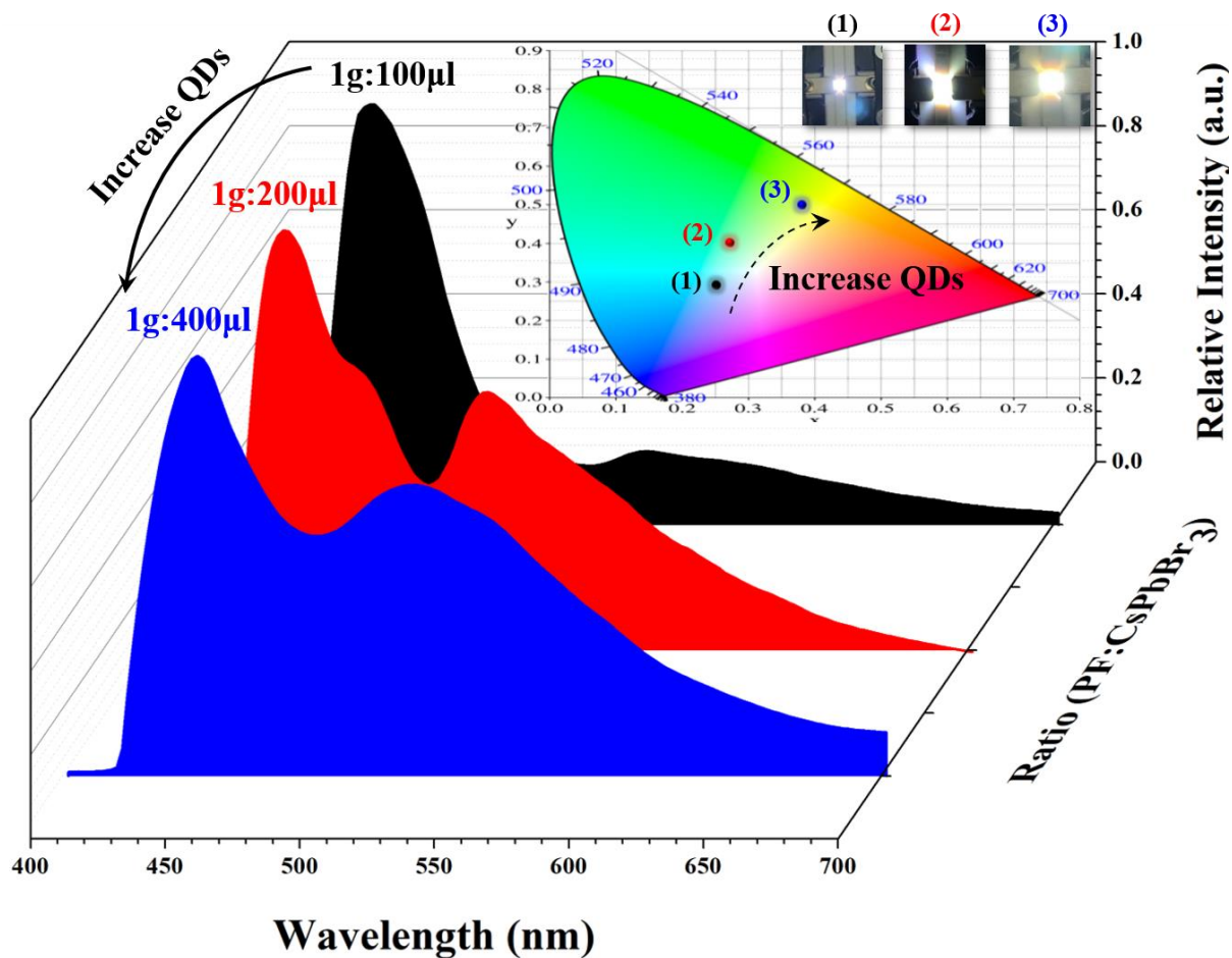
Figure 3.9. Emission spectra of different color LEDs with CIE color coordinates by using CsPbBr 3 @ PFN 24 - b -PBA 90 composite fibers under UV chip (380 nm) excitation and an applied voltage 3V. (Inset images show the LEDs applied by 1:100, 1:200, and 1:400 (g/μl) ratio of QD/polymer composite fibers)
