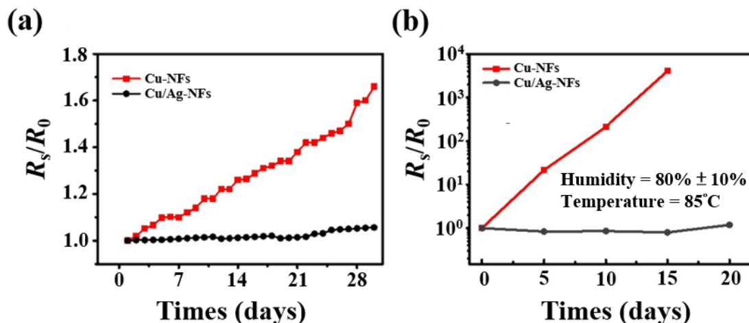
Figure 2.7. Oxidation test of Cu-NFs and Cu/Ag core/shell NFs at (a) room temperature and (b) humidity of 80% \pm 10% and 85°C.
