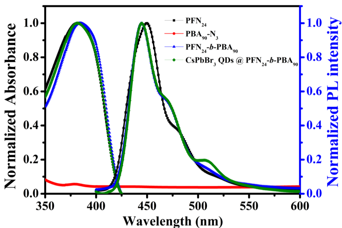
Figure 3.7. UV-vis absorption and PL emission spectrum of the PFN 24 -C≡CH, PBA 90 -N 3 , PFN 24 -b-PBA 90 , and CsPbBr 3 QDs@PFN 24 -b-PBA 90 films (1g/400 μl).
