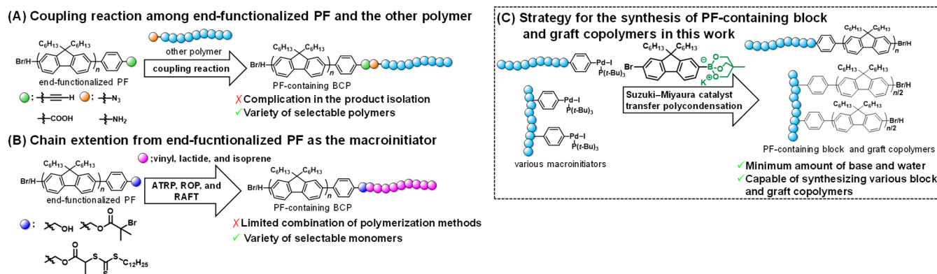
Figure 1. Schematic for the synthesis of the PF-containing block and graft copolymers. (A) Coupling reaction between end-functionalized PF and the other polymer. (B) Chain extension from end-functionalized PF as the macroinitiator. (C) Macroinitiator approach: Our strategy for the synthesis of PF-containing block and graft copolymers by SCTP of triolborate-type fluorene monomer.
