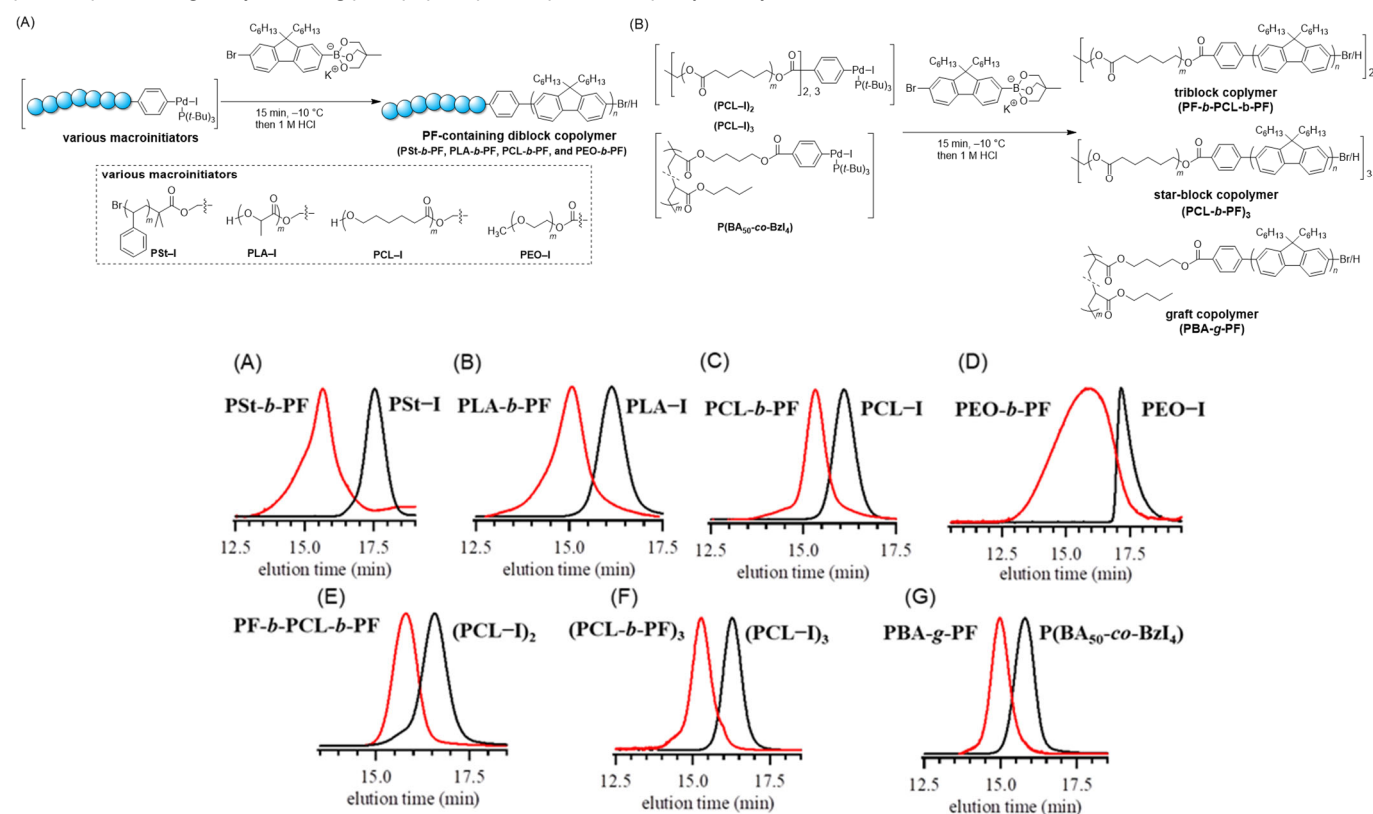
Figure 5. SEC traces of PF-containing block and graft copolymers (red curves: A, PSt- b -PF; B, PLA- b -PF; C, PCL- b -PF; D, PEO- b -PF; E, PF- b -PCL- b -PF; F, (PCL- b -PF) 3 ; and G, PBA- g -PF) and the corresponding macroinitiators (black curves: A, PSt-I; B, PLA-I; C, PCL-I; D, PEO-I; E, (PCL-I) 2 ; F, (PCL-I) 3 ; and G, P(BA 50 - co -BzI 4 )) detected by RI detector (eluent, THF; flow rate, 1.0 mL min -1 ).
