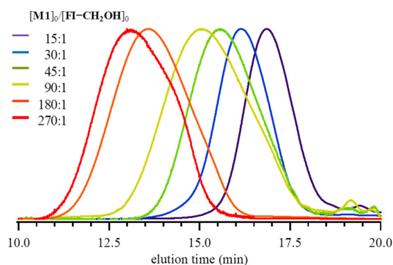
Figure 4. SEC traces of PFs obtained using different [M]_0/[FI-CH_2OH]_0 ratios (purple line, 15:1; blue line, 30:1; green line, 45:1; yellow line, 90:1; orange line, 180:1; red line, 270:1) detected by RI detector (eluent, THF; flow rate, 1.0 mL min ^{-1} ).
