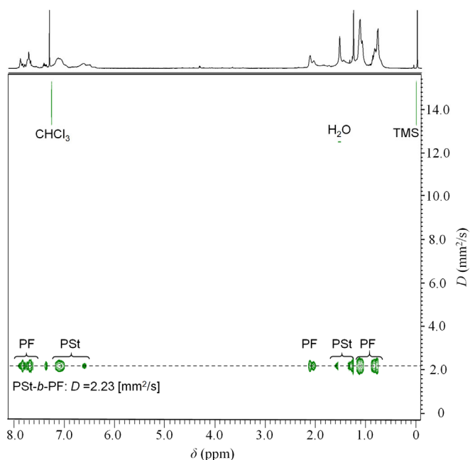
Figure 6. DOSY NMR spectrum of PST- b -PF (run 1, Table S3) in \text{CDCl}_3 (600 MHz).
