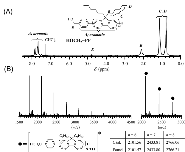
Figure 2. (A) 1 H NMR in CDCl 3 (400 MHz) and (B) MALDI-TOF MS spectra of HOCH 2 -PF obtained from run 5 (Table 1).
