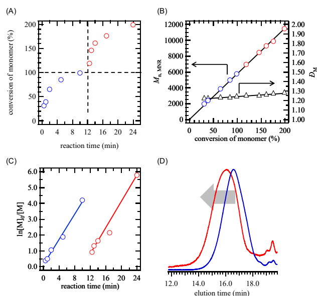
Figure 3. (A) Plot of time against conversion (blue, first polymerization; red, post-polymerization) for SCTP of M1 at [M]_0/[FI-CH_2OH]_0/[Pd_2(dba)_3 \cdot CHCl_3]/[t-Bu_3P] ratio of 15:1:0.3:2.2 in THF/water (10:1, v/v) at -10^\circ C . (B) Dependence of M_{n,NMR} (blue, first polymerization; red, post-polymerization) and D_M (triangle, dispersity) on monomer conversion. (C) First-order kinetic plots for SCTP (blue, first polymerization; red, post-polymerization). (D) SEC traces of PFs obtained before (blue line) and after (red line) second polymerization (eluent, THF; flow rate, 1.0 mL min ^{-1} ).
