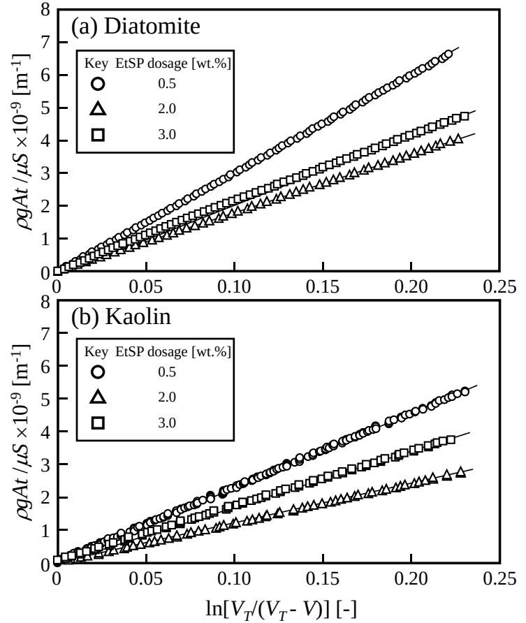
Figure 2 Determination of total filtration resistance, R , by fitting of the data to Equation (4) for (a) diatomite and (b) kaolin. The concentration of the particles was 20 \text{ kg/m}^3 . The value of the slope for the regression line (straight line) of the data corresponds to the total filtration resistance.
