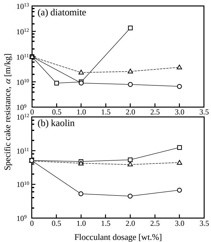
Figure 7 Comparison of the specific cake resistances, \alpha , of (a) diatomite and (b) kaolin flocs formed by EtSP (circle), chitosan (square) and PAC (triangle) as a function of flocculant dosage. The particle concentration is 20 g/L.
