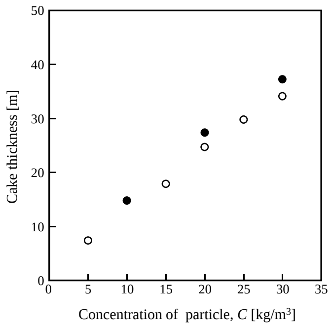
Figure 4 Effect of particle concentration, C , on the cake thickness for diatomite (open circle) and kaolin (solid circle). Dosage of EtSP was 1.5 wt.% of both the particles.
