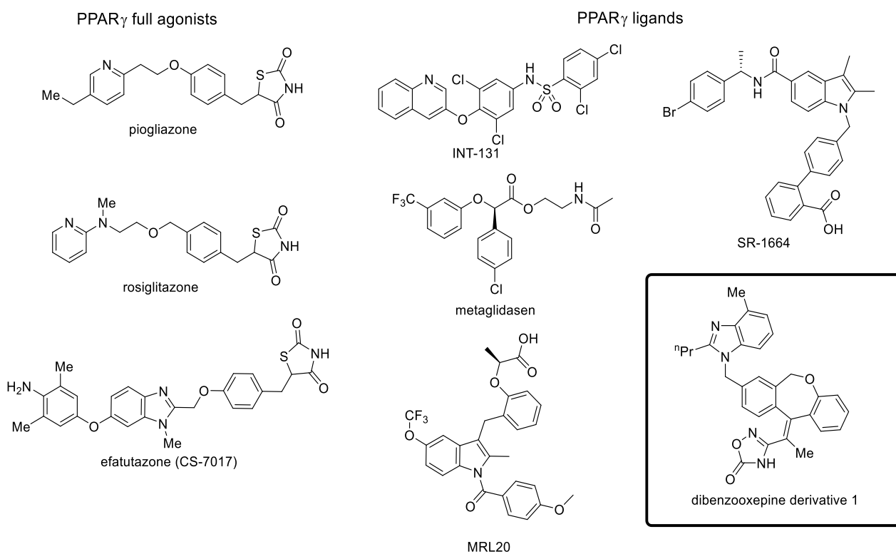
Figure 1. The representative PPAR \gamma ligands.
