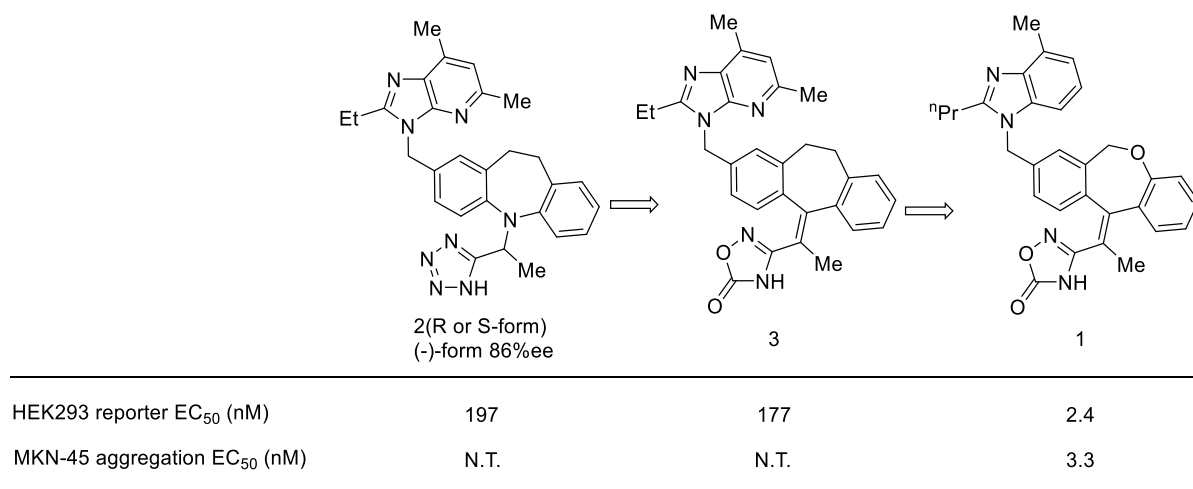
Figure 2. Identification of lead compound 1 from HTS hit compound 2 .
