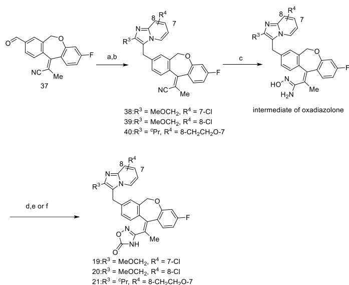
Scheme 3 Synthesis of the side chain structure from 8-formyldihydrodibenzooxepine a
