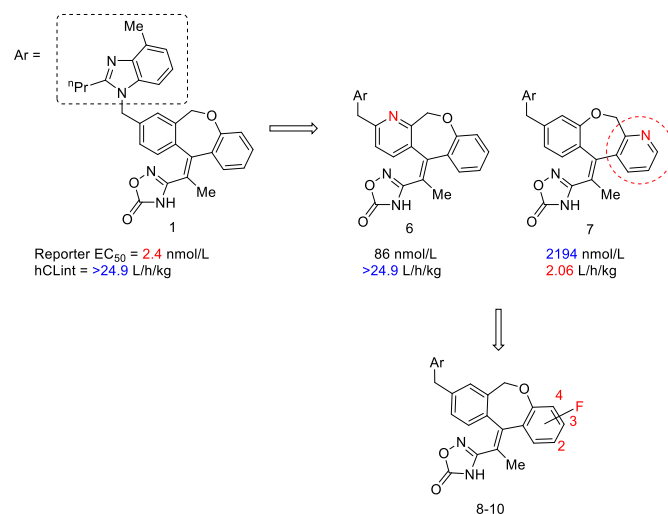
Figure 5. Improvement of the human metabolic stability of lead compound 1 by modification of the tricyclic core-structure.
