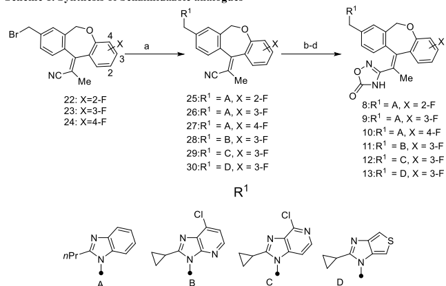
Scheme 1. Synthesis of benzimidazole analogues a
