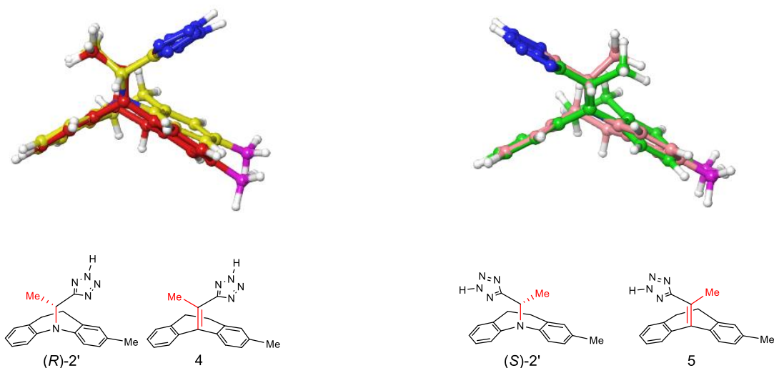
Figure 3. Overlay of the most stable conformations of the chiral model compounds ( R )-2' and ( S )-2' on their non-chiral olefinic bioisosters 4 and 5, respectively. Global energy minimum conformations of these compounds were calculated by the MacroModel. The hydrogens, nitrogens, and 2-methyl group are colored white, blue and magenta, respectively.
